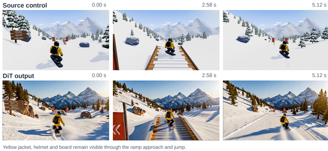
Figure 10 Recorded game control and anime-conditioned generation at matched timestamps. The source recording supplies the motion timeline; a locally edited first frame supplies appearance. This development example uses four denoiser evaluations and does not measure live game input-to-display latency.
