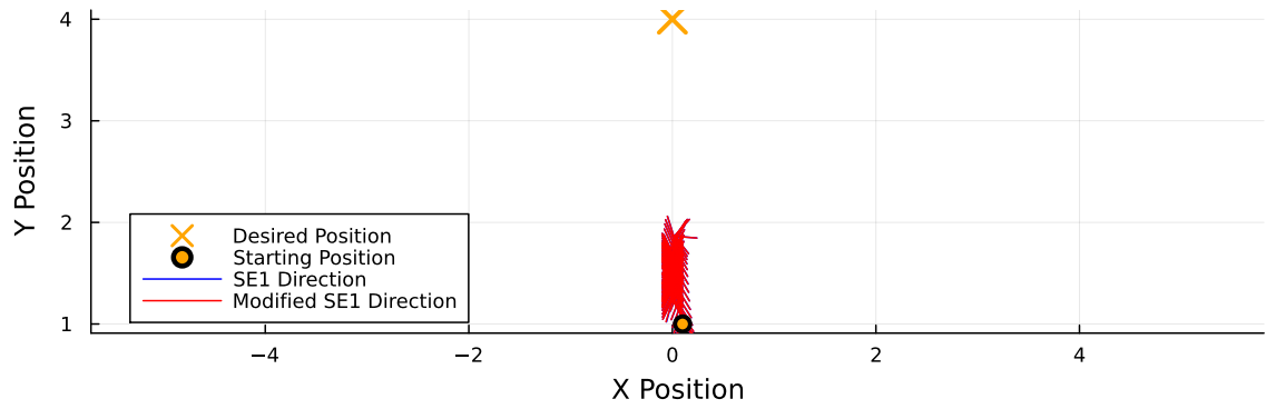
Figure 41: Comparison of SE1 and Modified SE1 for \alpha = 5.0 , N = 100 , l_0 = 2.5 , and x_0 = [0.1, 1.0]
