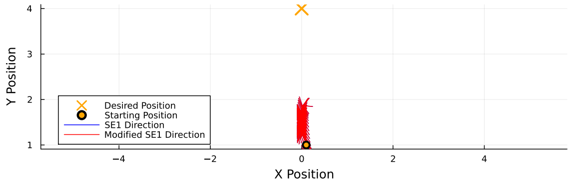
Figure 31: Comparison of SE1 and Modified SE1 for \alpha = 10.0 , N = 100 , l_0 = 2.5 , and \mathbf{x}_0 = [0.1, 1.0]
