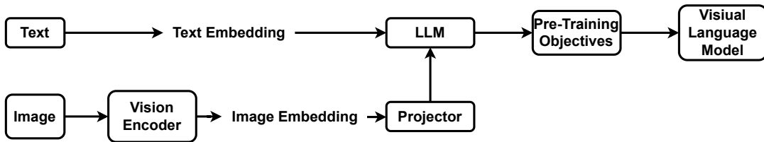
Figure 6: Conceptual VLM workflow: the vision encoder produces embeddings that are aligned and fused with LLM tokens to support multimodal reasoning and grounded responses.[LWD + 25]
