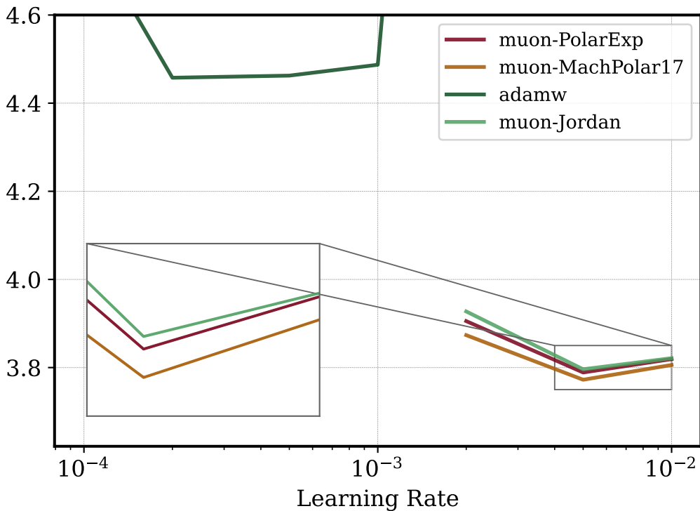
Final Validation Loss
