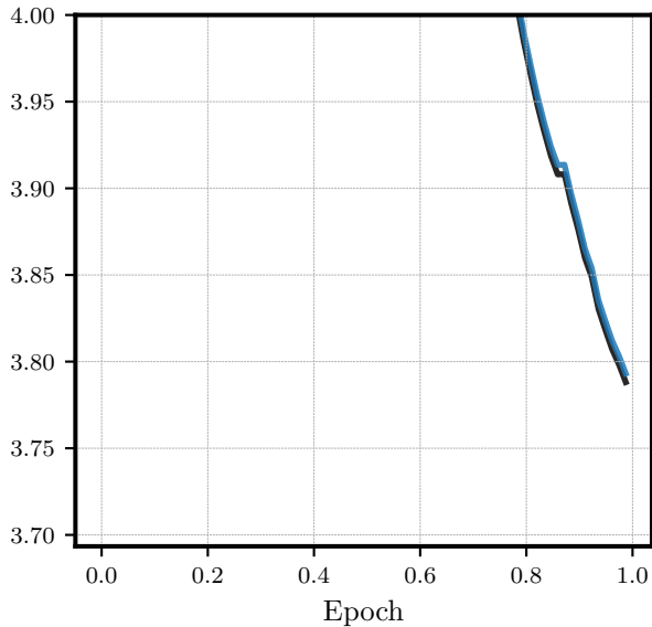
Validation Loss
