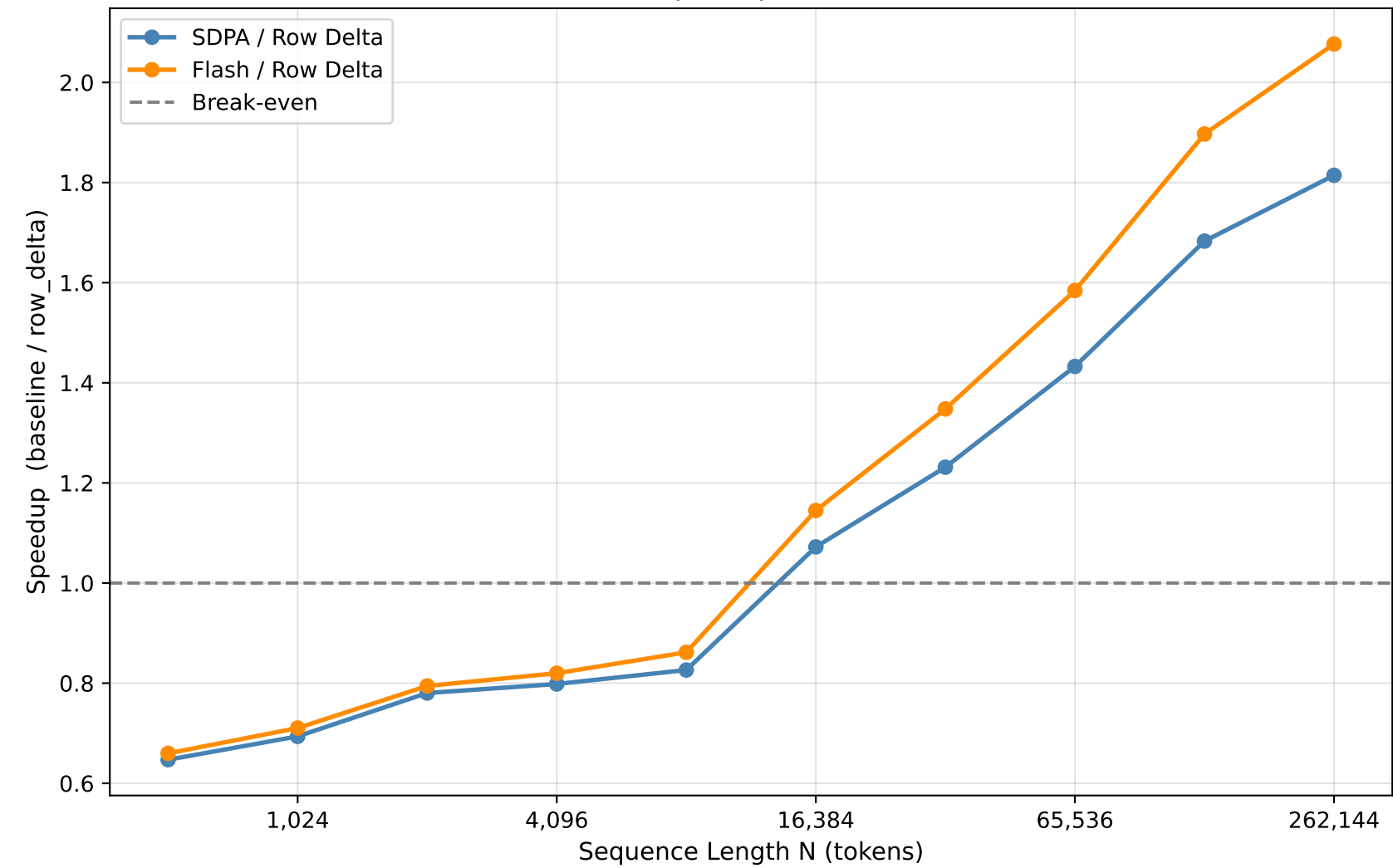
Overhead: time_delta_mm_pattern
