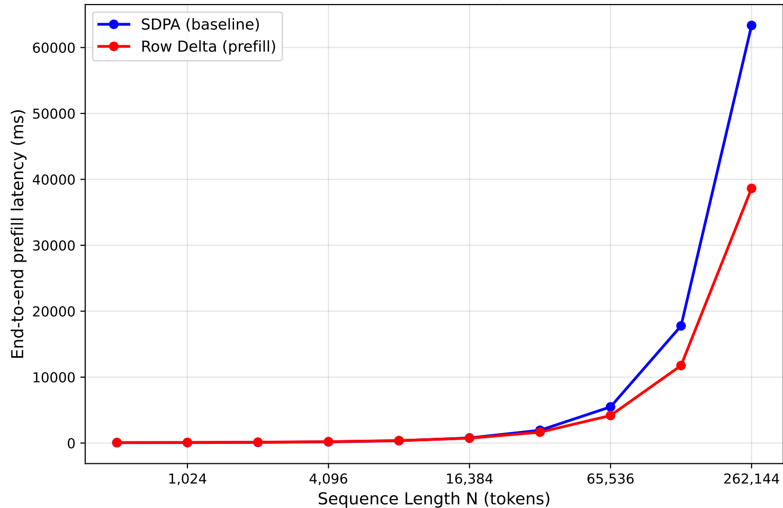
Absolute latency
