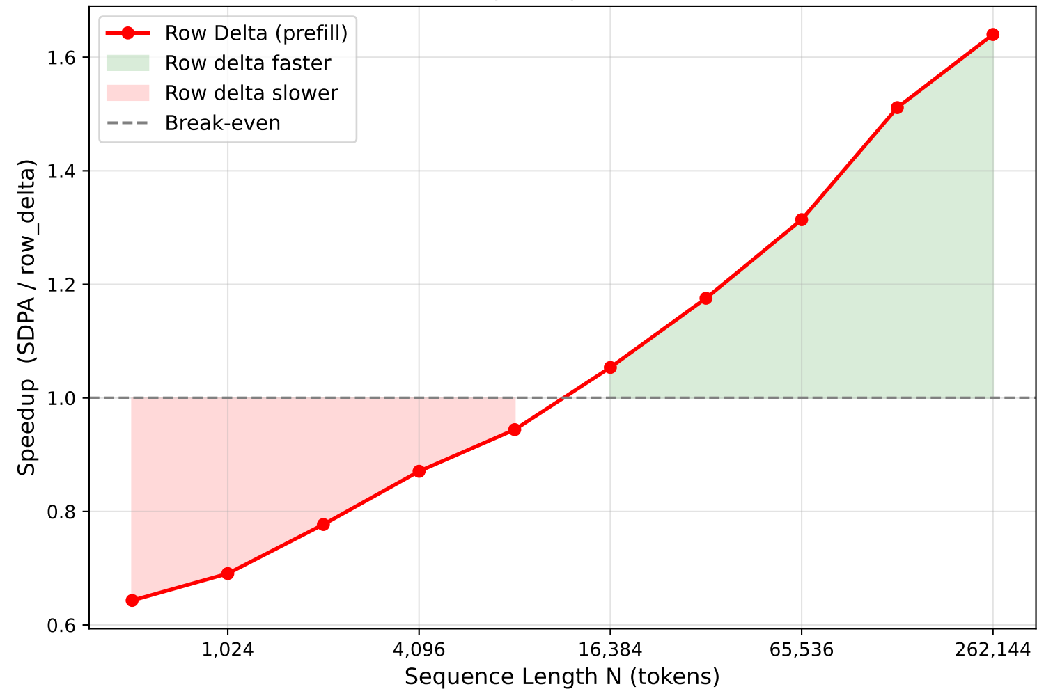
Speedup ratio
