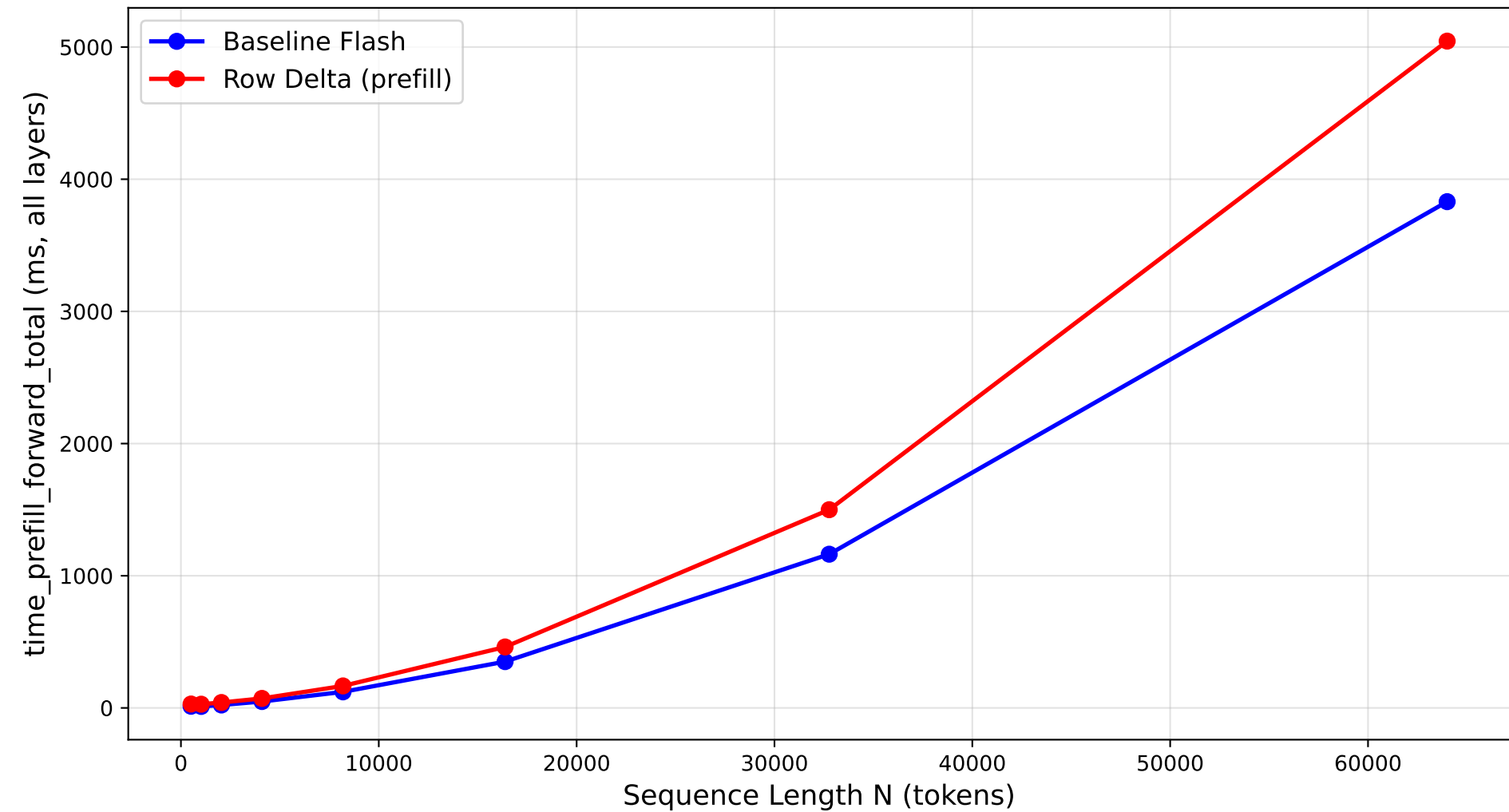
Prefill Latency: Row Delta vs Baseline Flash (LLaMA 3.1 8B-Instruct, Wikitext)
