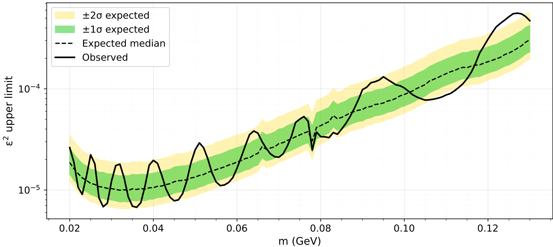
2015: expected/observed 95% CL upper limits on \varepsilon^2
