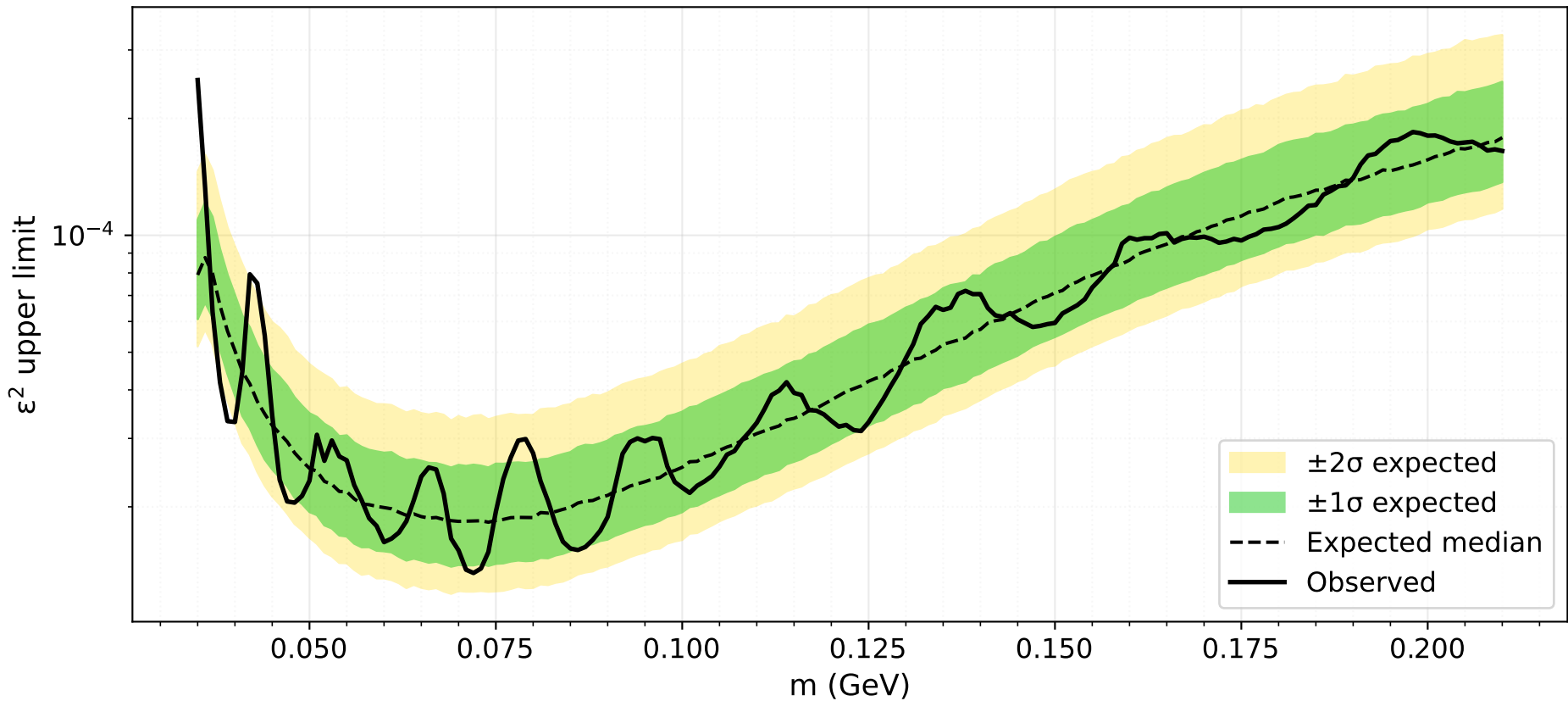
2016: expected/observed 95% CL upper limits on \varepsilon^2
