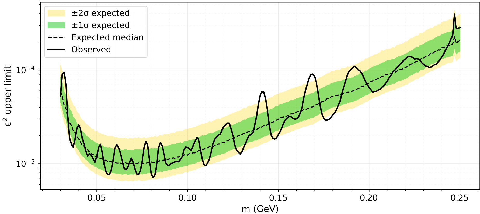
2021: expected/observed 95% CL upper limits on \varepsilon^2
