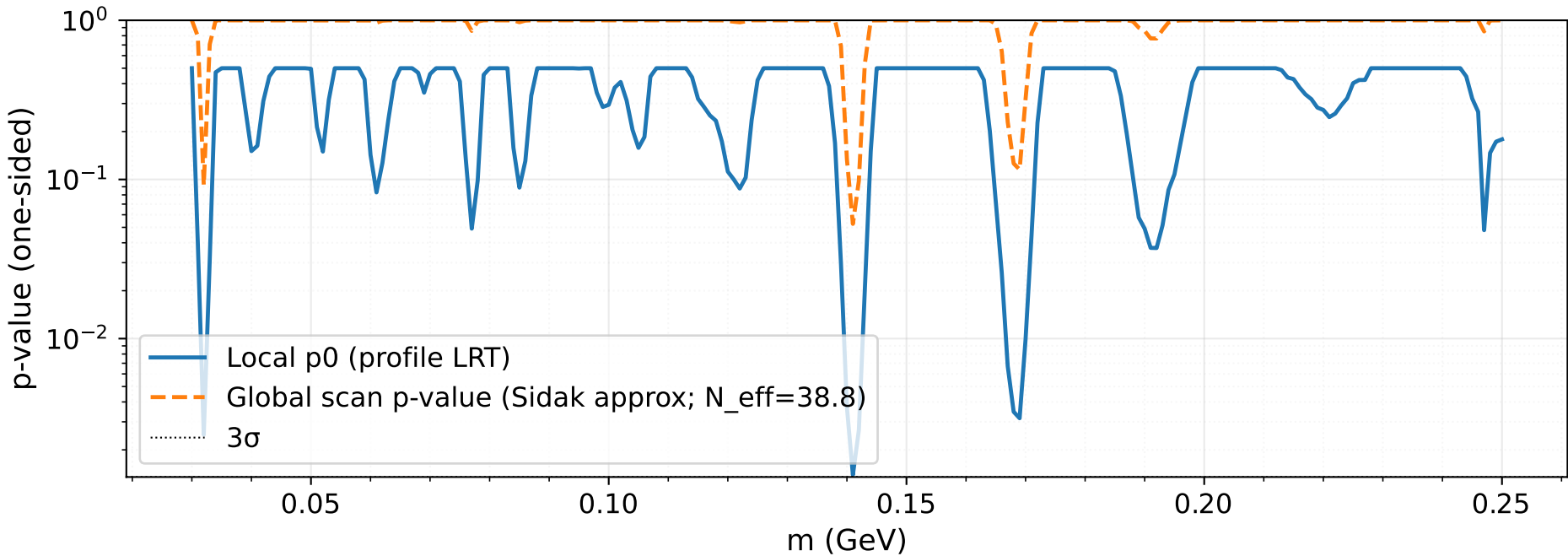
2021: local p0 and global p-value overlay
