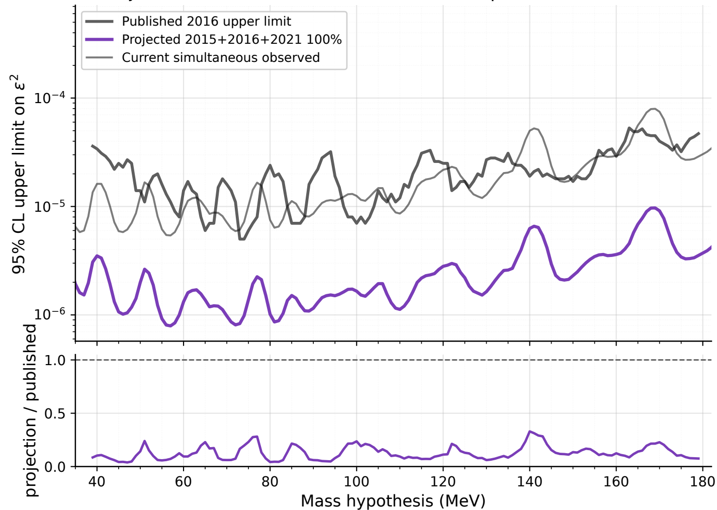
Projected full-dataset simultaneous limit vs published 2016 result
