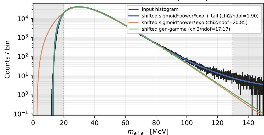
HPS 2015 candidate-family overlay
