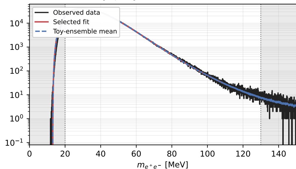
HPS 2015 / shifted sigmoid*power*exp + tail Scan [20, 130] MeV / N events = 2.145e+07
