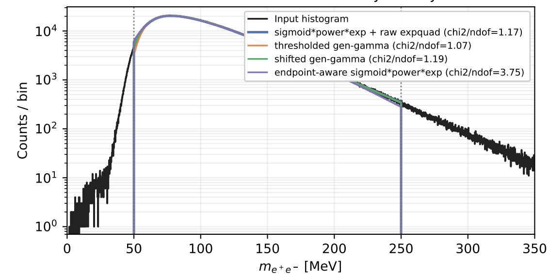
HPS 2021 1% candidate-family overlay
