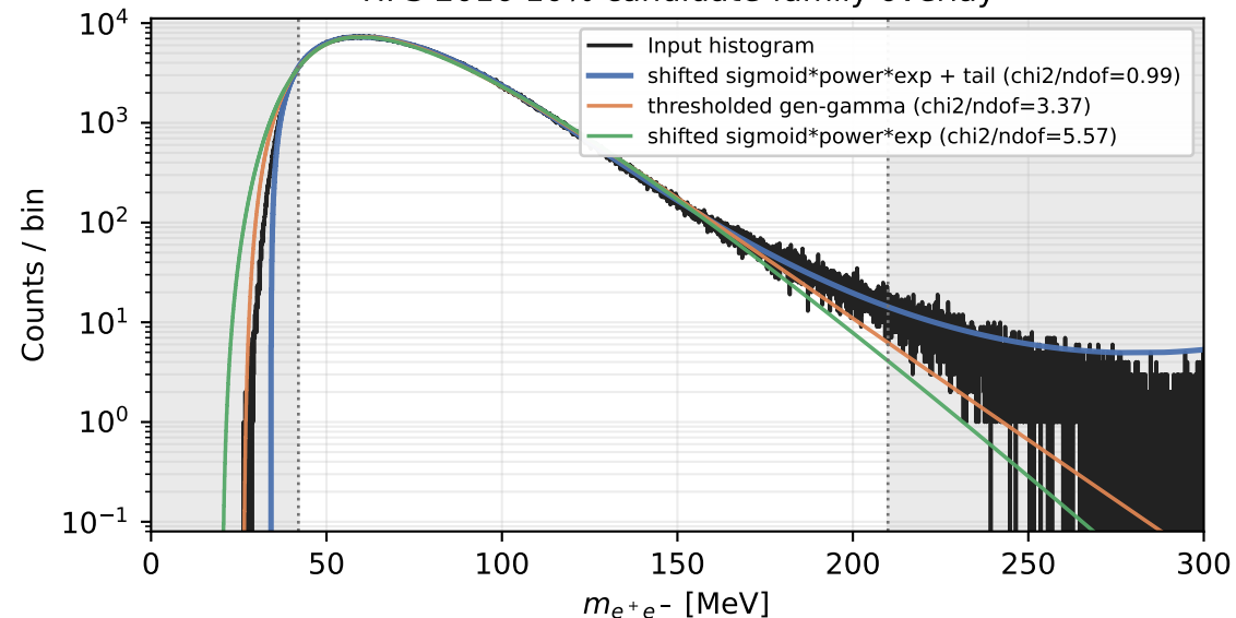
HPS 2016 10% candidate-family overlay
