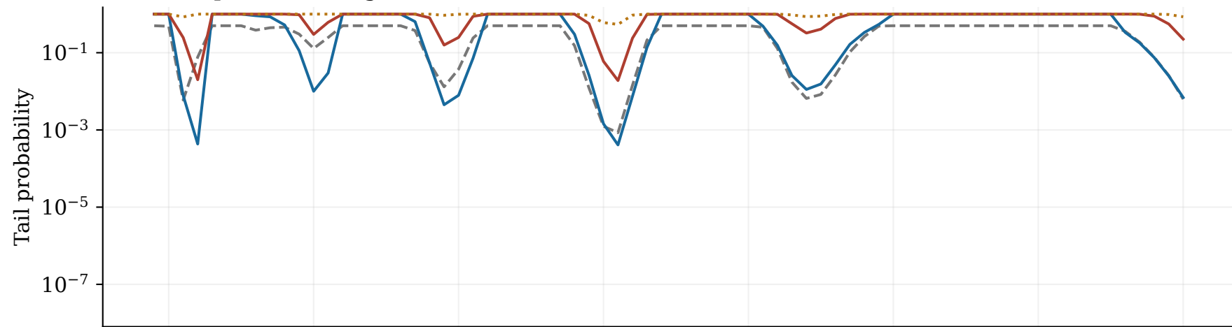
Gaussian-profiled background
