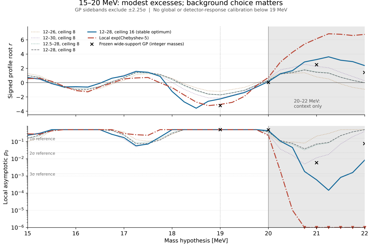
Figure 18: Signed roots and local asymptotic excess probabilities. All four initial GP supports reach the inherited ceiling of eight resolution units. Raising the nominal-support ceiling to 16 removes every active boundary; ceilings 32 and 64 recover the same optima, with maximum root changes below 0.00054. The local polynomial is a separate background-family check. Gray shading identifies the 20–22 MeV bridge. Triangles mark the 10^{-6} display floor, not resolved global tails.
