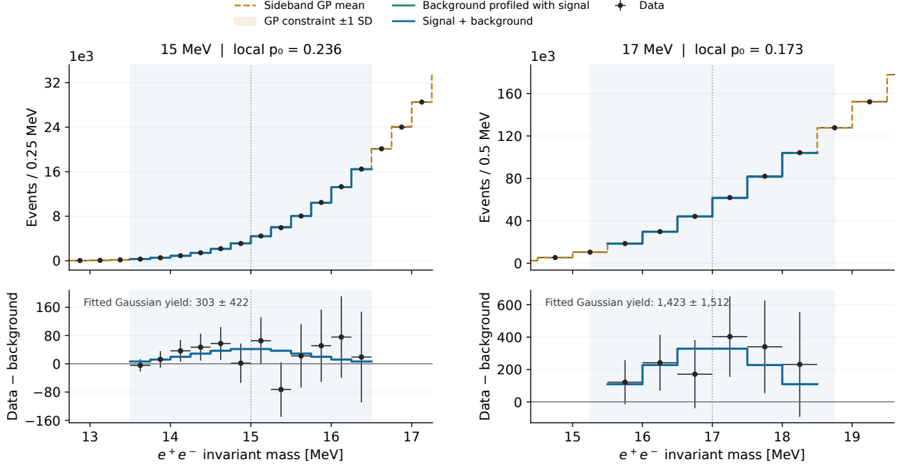
2015 full | GP support 12–28 MeV, stable ceiling 16 | Shading: fitted signal window Counting error bars only. Residuals share fitted-background uncertainty; they are not independent significances.
