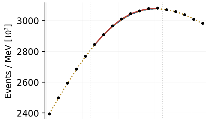
66 MeV: Common-bin sum
