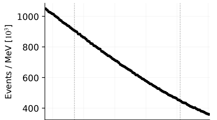
92 MeV: 2016 full
