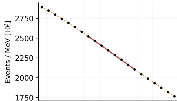
92 MeV: Common-bin sum
