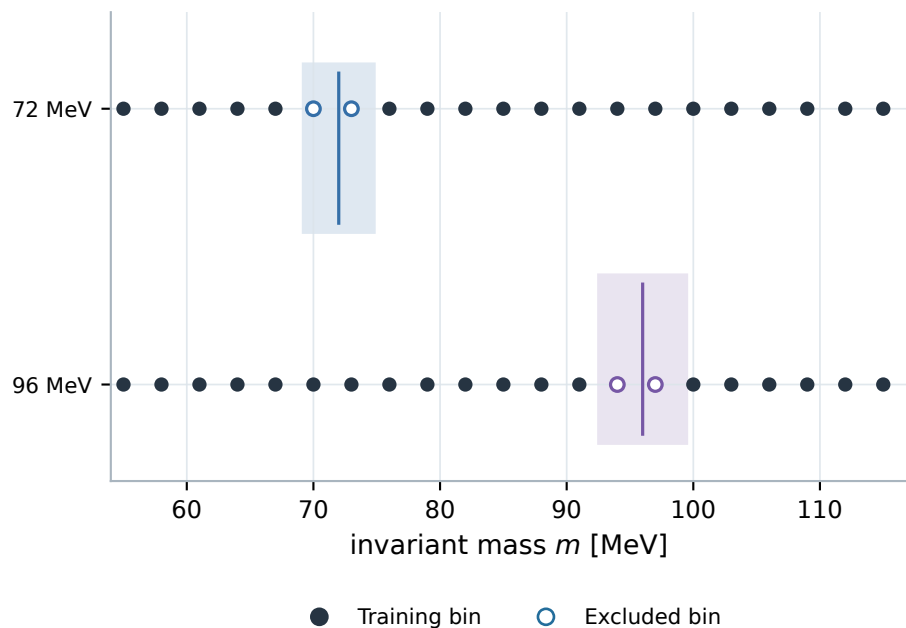
(c) Moving the test mass moves the mask
