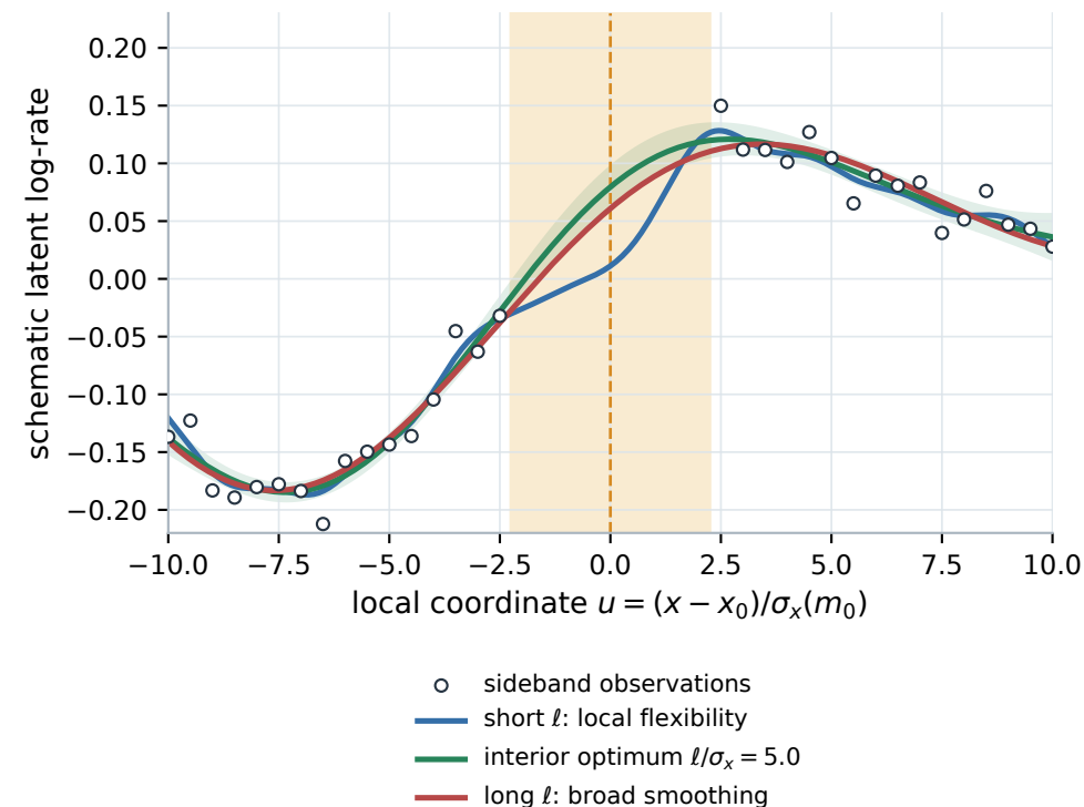
(a) Interpolation through excluded bins
