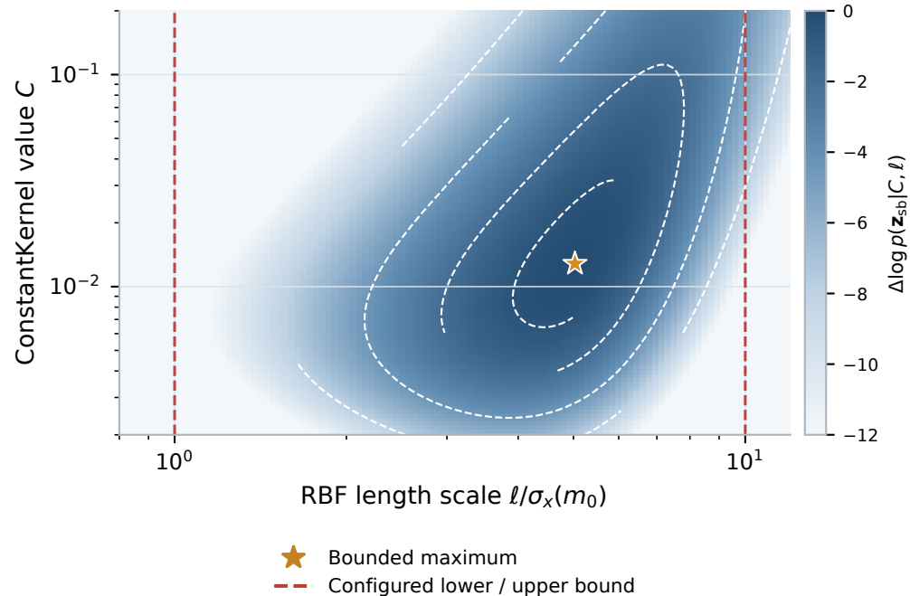
(b) Joint covariance-parameter selection
