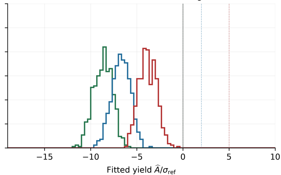
Combined: archived stress background
