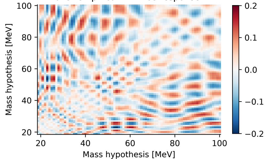
2016: empirical R minus response R
