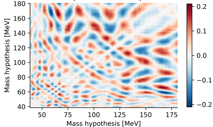
2021: empirical R minus response R
