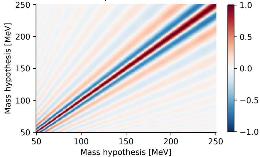
2021: response correlation R
