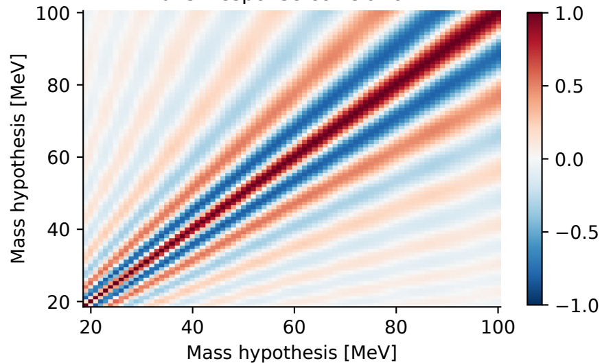
2016: response correlation R
