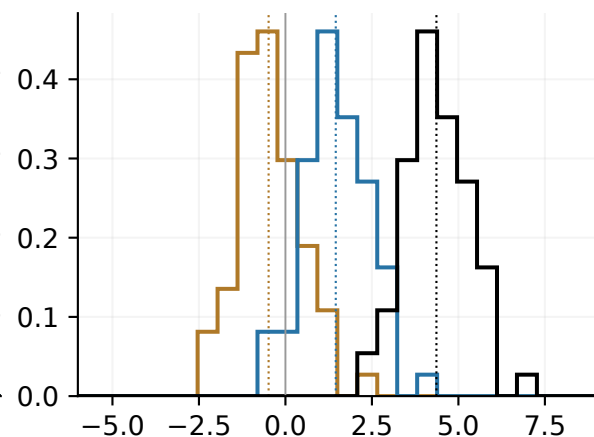
2011 at 71 MeV Local-GP control
