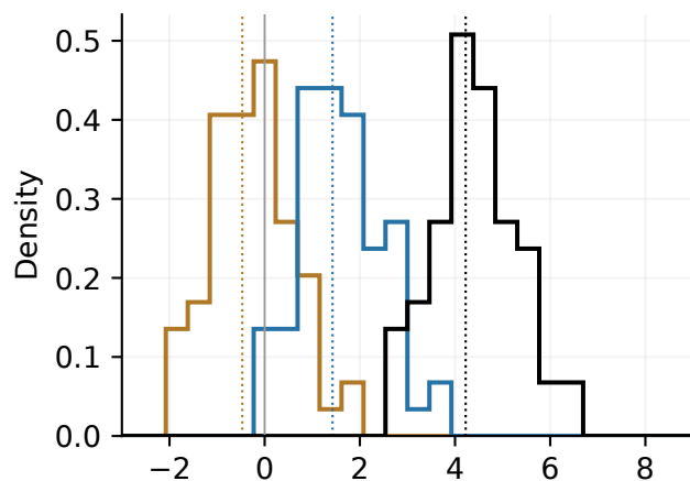
2015 at 95 MeV Local-GP control
