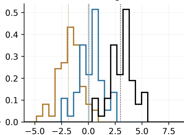
2011 at 71 MeV Stress background
