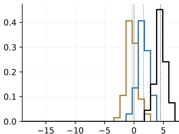
2016 at 76 MeV Local-GP control
