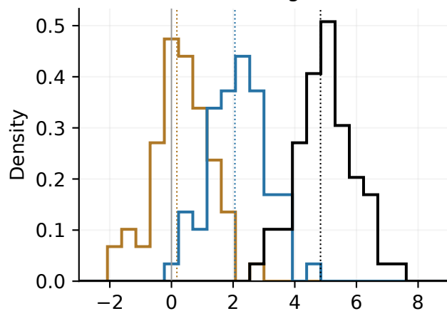
2015 at 95 MeV Stress background
