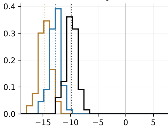
2016 at 76 MeV Stress background
