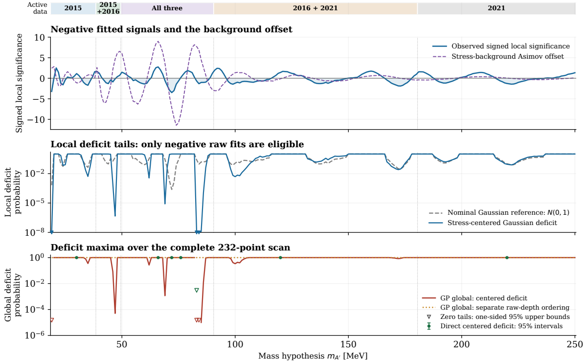
Figure 101: Profiled deficit scan. Top: observed signed local significance and the stress-background offset; shading marks negative fitted contributions. Middle: raw-root Gaussian reference and conditional Gaussian-response tails. Both assign one to nonnegative raw roots. Local triangles mark the 10^{-8} display floor. Bottom: two separate global orderings; triangles mark one-sided 95% zero-count bounds. Direct error bars are central 95% intervals.
