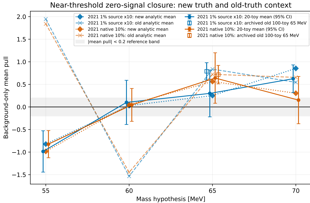
Figure 113: Historical 20-background near-threshold closure. Points carry 95% Student- t intervals; deterministic responses to the old and new analytic means expose the truth-shape dependence. The known 65 MeV response improves in the 1%-source test, while neighboring offsets remain. The later 100-background replacement results in the main text use their own identified truth and support; they are not pooled into these curves.
