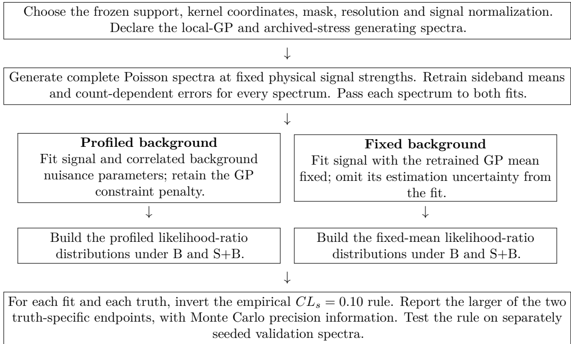
Figure 87: How the two background treatments are calibrated. Both branches receive identical spectra. The primary comparison uses two declared background truths for each method; it does not average the two methods or select whichever gives the tighter observed limit. B denotes background only and S+B denotes signal plus background.
