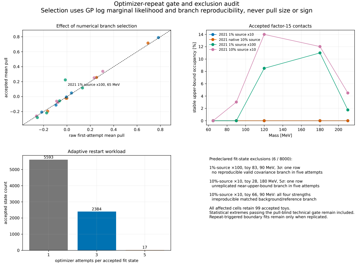
Figure 103: Optimizer-repeat gate and exclusion audit. The upper-left panel compares zero-signal means from the raw first attempts with the accepted LML-selected states; the visibly repaired 1\% \times 100 , 65 MeV point is numerical rather than a pull-based deletion. The upper-right panel reports accepted factor-15 contacts. The lower-left panel gives the adaptive attempt workload, and the lower-right panel lists all six excluded states. Statistical extremes that pass the pull-blind technical gate remain in the headline summaries; repeat-triggered boundary solutions are retained when replicated.
