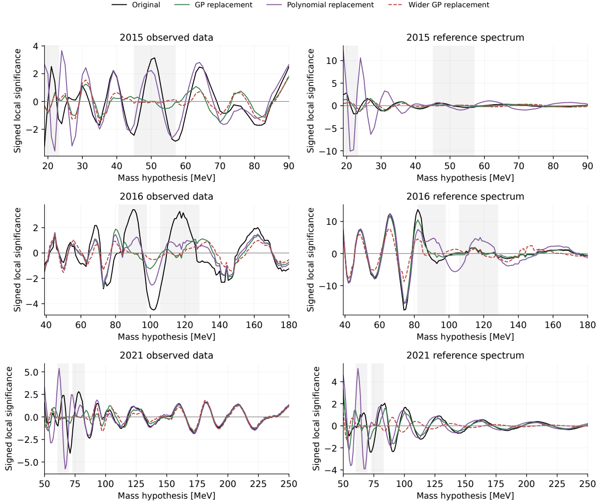
Figure 97: Both-hole replacements in observed counts (left) and the reference spectrum (right). Green: primary GP mean. Purple: exponential-polynomial fill. Dashed red: wider GP holes. The reference ordinate a_m = r_m(B) is the fitted root, not the background event rate. Gray shading marks primary holes; wider holes extend beyond it. All outcomes remain visible, including unsuccessful interpolation. No altered spectrum supplies a new observed-data probability.
