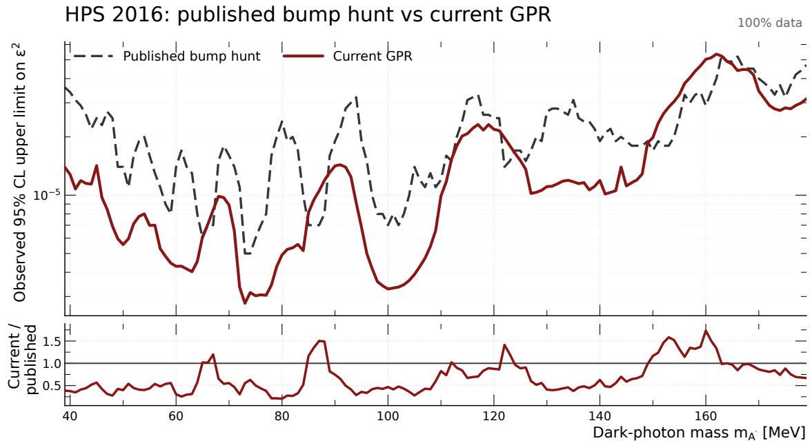
Figure 116: Saved 2016 observed 95% confidence-limit comparison from 5 August 2026, using the full already analyzed 2016 sample. The published reference uses the polynomial CL_s method; the curve labeled “current” in this archived graphic means the then-current v4.1 factor-12 GPR candidate. It does not mean the v5.0.1 configuration. The lower panel gives the pointwise observed GPR/published ratio, whose median is 0.5579 over 141 matched masses. This was an observed, asymptotic comparison with fixed reviewed kernel coordinates, no new toys, and no expected-limit bands.
