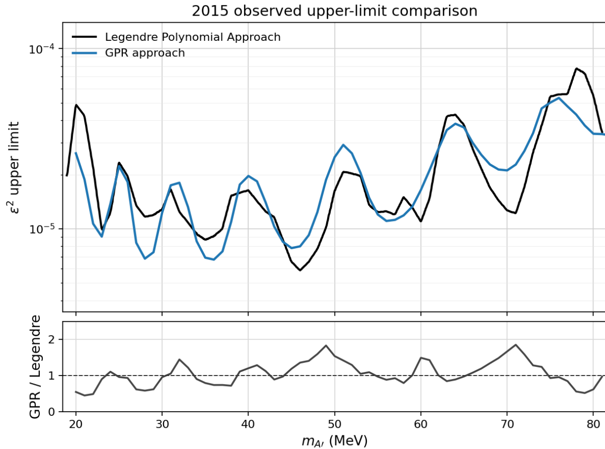
Figure 115: Restored historical 2015 observed 95% confidence-limit comparison from Appendix E of v4.9.7. The black “Legendre Polynomial Approach” curve is the corrected 2015 re-analysis digitized from Fig. 71 of the 2016 internal note; the blue curve is the earlier GPR comparison for the same full 2015 sample. The lower panel is the pointwise ratio of these saved curves, with median 0.99 and mean 1.06 over 20 MeV to 81 MeV. Both curves predate the current v5 settings. Their similar normalization scale does not establish coverage or absence of signal absorption.
