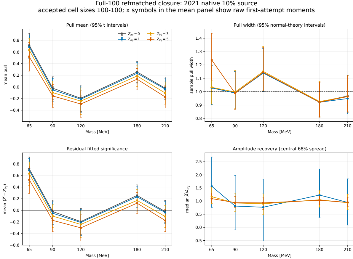
Figure 107: As in Fig. 106, for the native-10% ensemble. All cells retain 100 toys. The largest mean offset is at 65 MeV. The only accepted width outside 0.8–1.2 in the complete study is 1.237 for the 65 MeV, z = 5 cell; its normal-theory 95% interval is [1.086, 1.437] .
