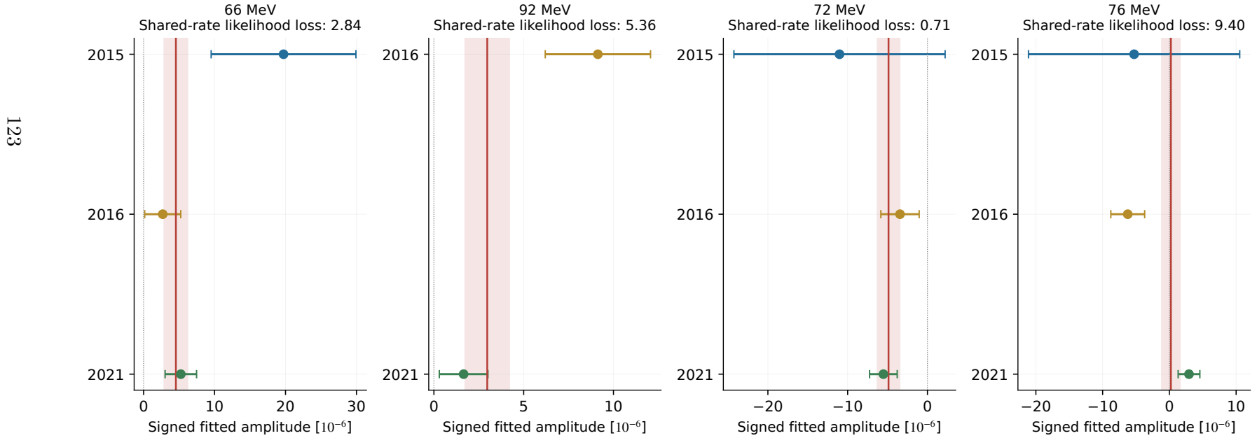
Figure 86: Separate campaign coupling estimates and local curvature errors compared with the common rate. The likelihood loss quantifies how much the local fit improves when each year can choose its own amplitude. The 66 MeV fit has positive contributions from all three years; the 92 MeV separate rates differ more visibly. These selected comparisons and local errors are not post-selection compatibility tests.
