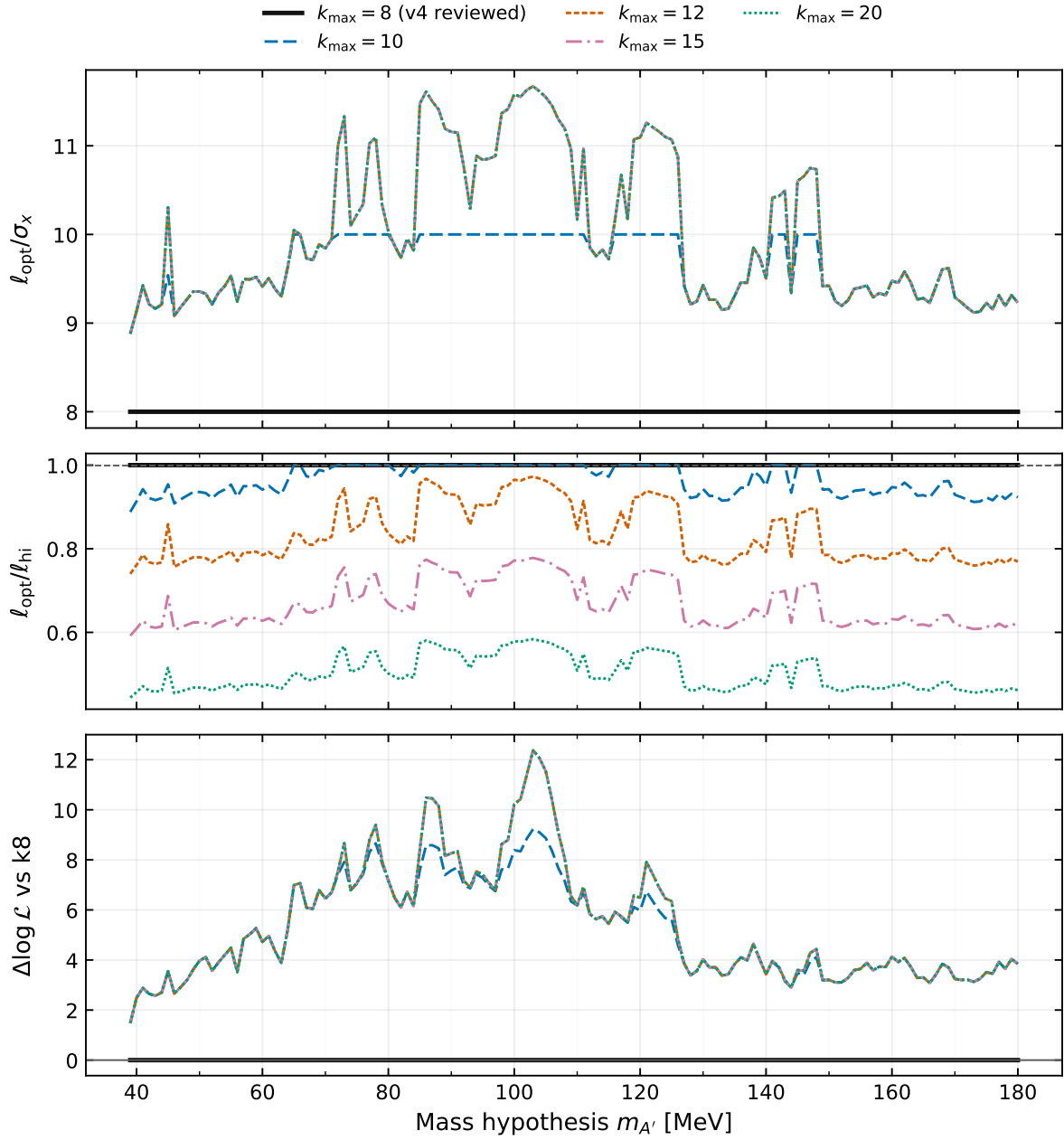
Figure 114: The controlled 2016 upper-length-scale study, restored from v4.9.7 Figure 74. The optimized scales, boundary occupancy and GP log marginal likelihood are compared on identical data and mass hypotheses. Factor twelve is the first nonbinding tested setting and is followed by the factor-fifteen/factor-twenty plateau. This observed-data numerical range diagnosis is not an expected-sensitivity or coverage optimization.
