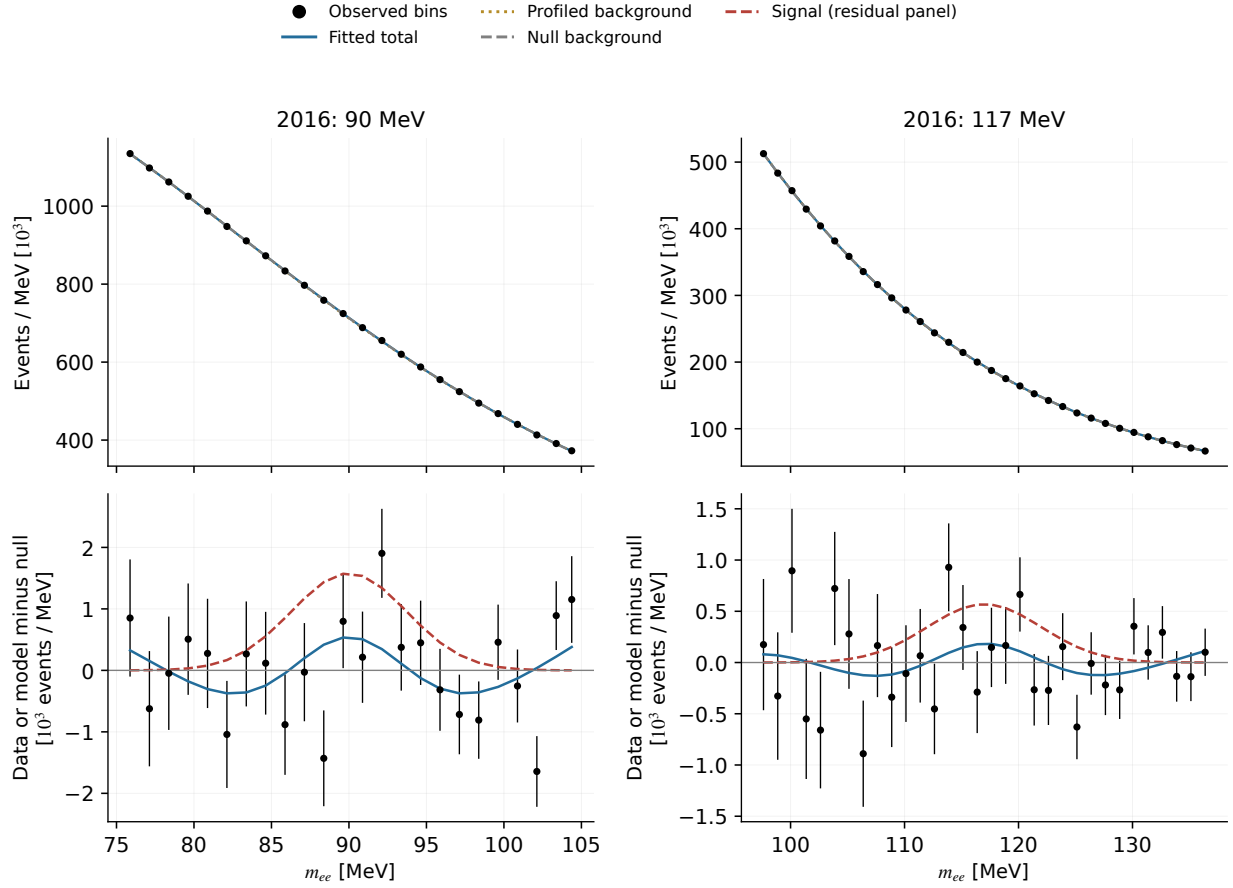
Figure 99: Traditional baseline fits to full 2016 data. At 90 and 117 MeV the nominal local coordinates are 1.998 and 1.525, with D/\text{dof} = 125.35/113 and 165.59/155 . The display sums five adjacent native bins to 1.25 MeV; any partial endpoint is retained. Counts, residuals and predictions are divided by each displayed width. Fits and probabilities still use the original 0.25 MeV bins. Both baseline positive roots are weaker than their GP values. Reducing the polynomial degree gives negative yields and larger deviances (Table 21). All alternatives are retained. Numerical convergence does not establish that a background describes the data; nominal local probabilities refer only to that model at the already selected mass.
