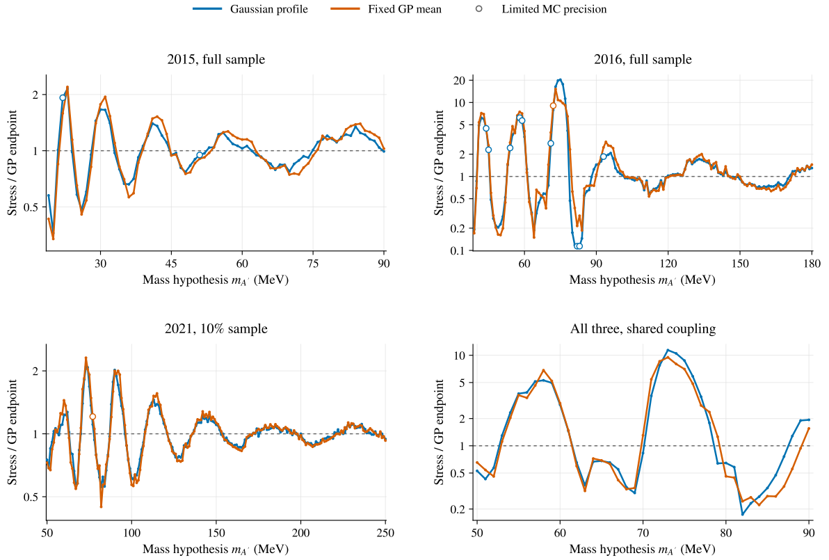
Figure 92: Ratio of the stress-truth to local-GP calibrated endpoint. Values above one indicate that the stress background controls the larger endpoint; values below one indicate that the local-GP control does. Open circles mark limited precision in at least one component, and gaps retain unavailable or censored ratios. This comparison diagnoses the chosen background family rather than certifying either member.
