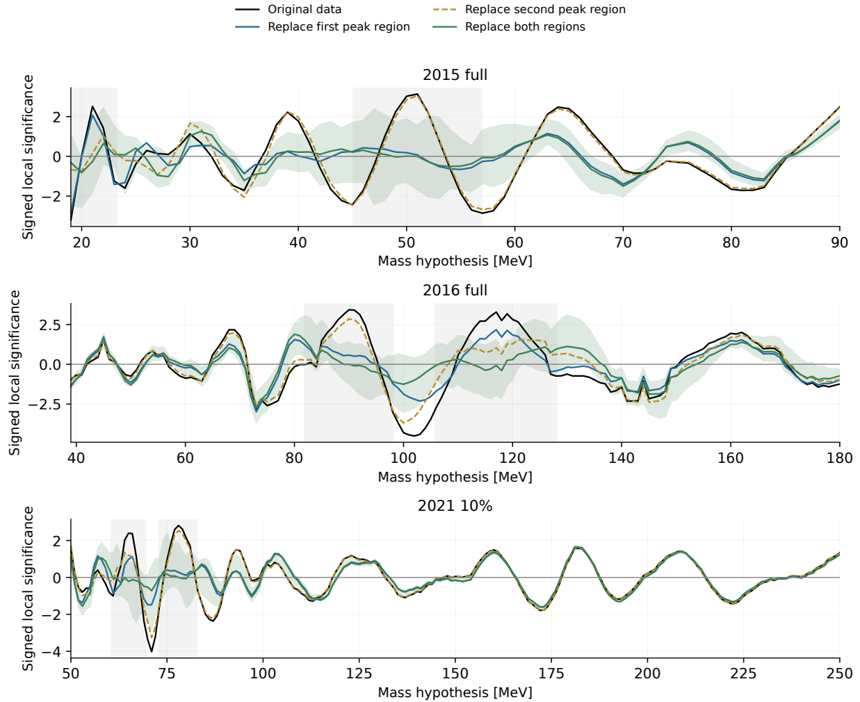
Figure 96: Observed scans before and after replacement. Black: original data. Blue and dashed orange: deterministic replacement of the first or second listed region. Green: both. The light green envelope spans the ten paired, conditional GP-plus-Poisson replacements with both holes filled; it is not a confidence band. Gray vertical regions show the primary holes. Curves join the existing 1 MeV hypotheses without extra smoothing. The ordinate is a signed local significance, not a newly calibrated significance. Removing a peak’s own bins predictably weakens that feature; the informative changes are in the surrounding pattern and retained regions.
