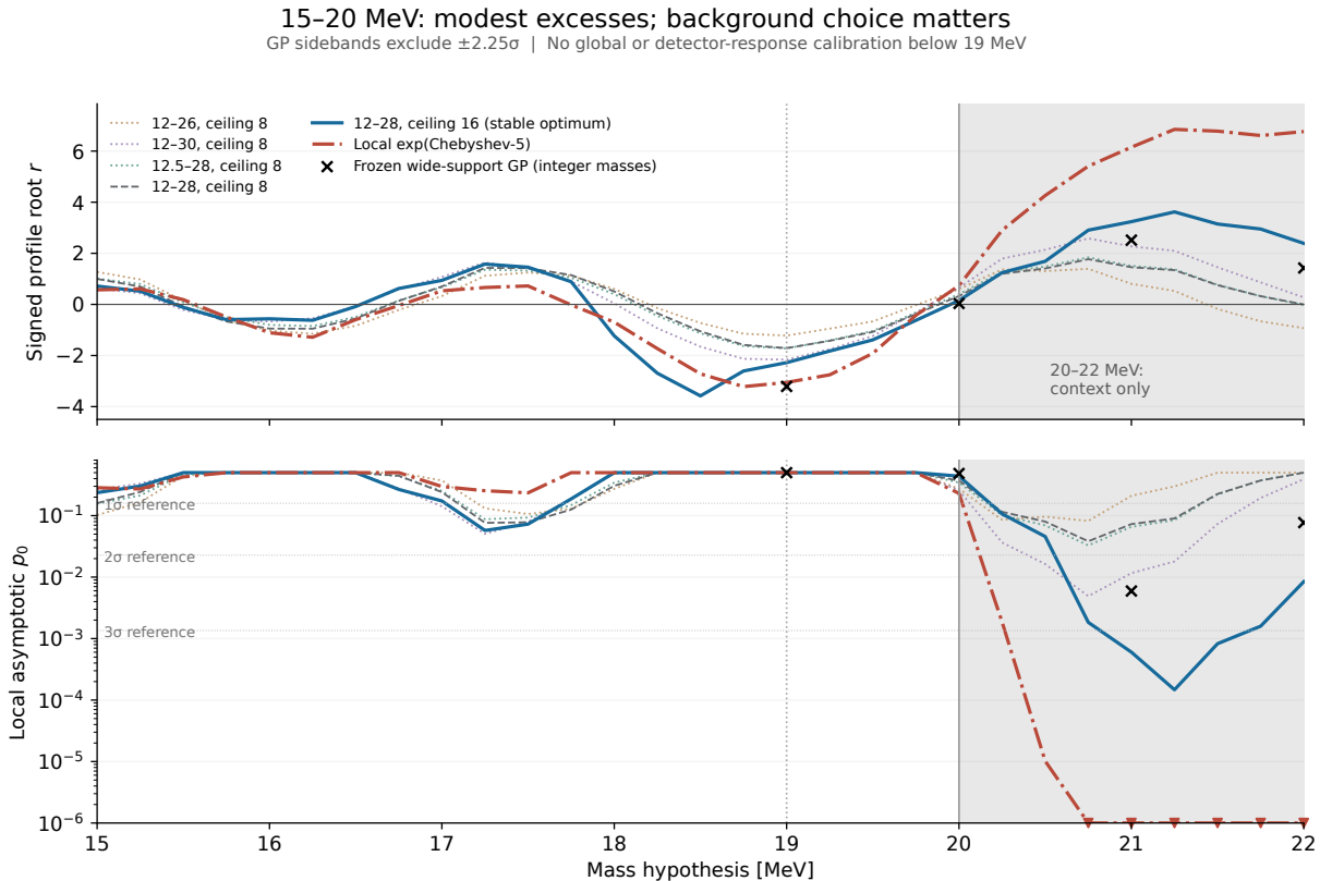
Figure 118: Signed local significance and local asymptotic excess probabilities. All four initial GP supports reach the inherited ceiling of eight resolution units. Raising the nominal-support ceiling to 16 removes every active boundary; ceilings 32 and 64 recover the same optima, with maximum root changes below 0.00054. The local polynomial is a separate background-family check. Gray shading identifies the 20–22 MeV bridge. Triangles mark the 10^{-6} display floor, not resolved global tails.
