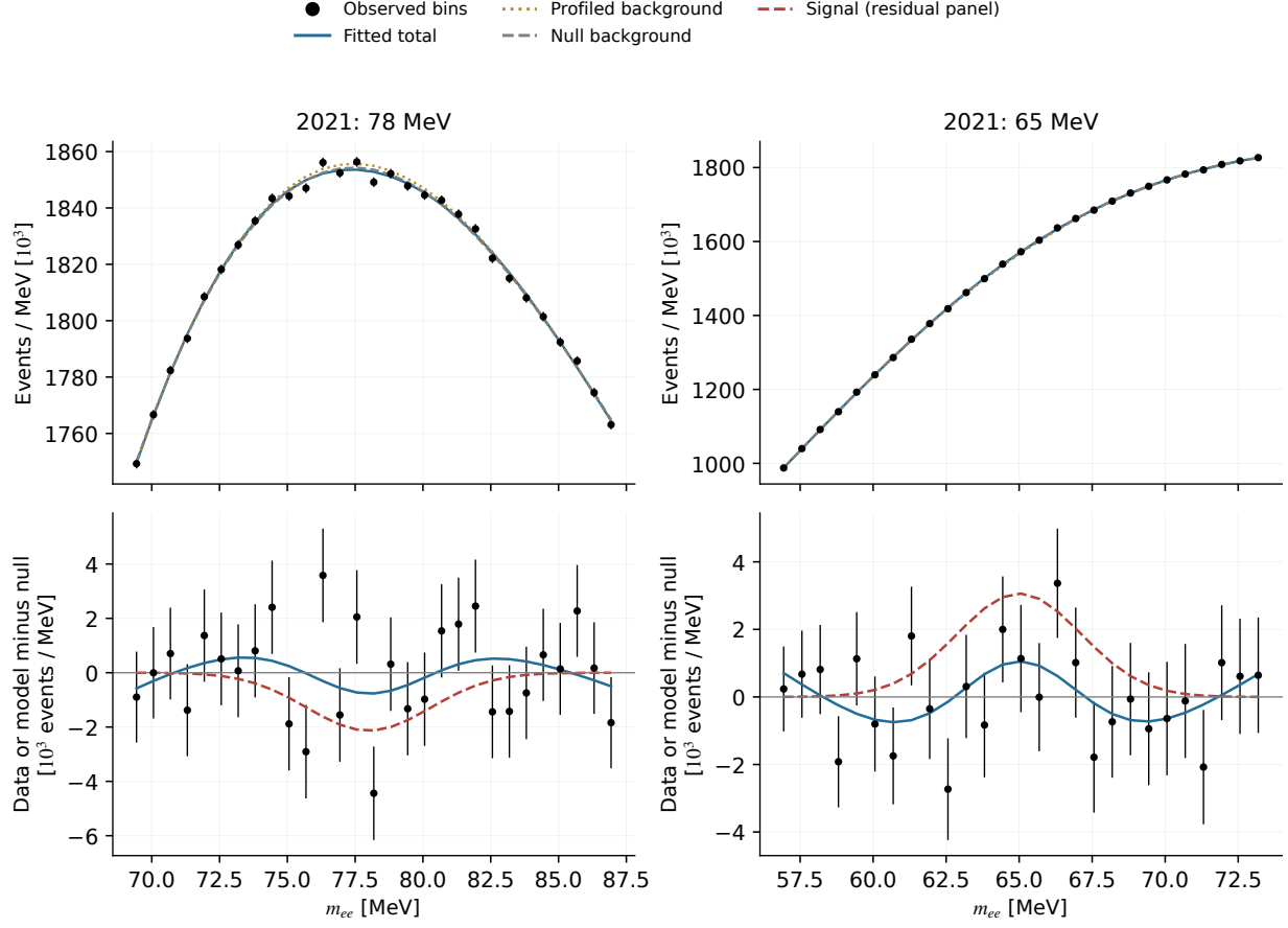
Figure 100: Traditional baseline fits to the released 2021 10% sample. At 78 and 65 MeV the signed local coordinates are -1.350 and 1.960 , with D/\text{dof} = 29.16/24 and 17.36/22 . Original 0.625 MeV bins are retained and displayed as counts per MeV. The 78 MeV feature becomes a deficit for every specified conventional fit. The 65 MeV baseline remains a modest positive excess. Its degree-two alternative gives a very large positive root but D/\text{dof} = 28.10 , showing a severe background-model failure (Table 21). Counting bars and the fitted Gaussian component are visual aids, not independent residual significances. No additional 2021 data were opened.
