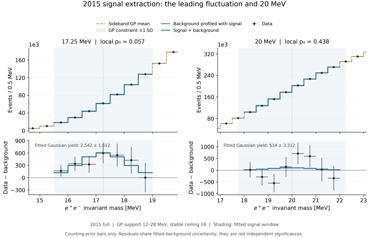
Figure 120: The selected 17.25 MeV upward fluctuation and the fixed 20 MeV hypothesis, with the same conventions and fixed-phase grouping as the preceding displays. Their local asymptotic roots are 1.58 and 0.16. A convincing resonance would need a stable excess across defensible background choices and a validated accepted signal shape.
