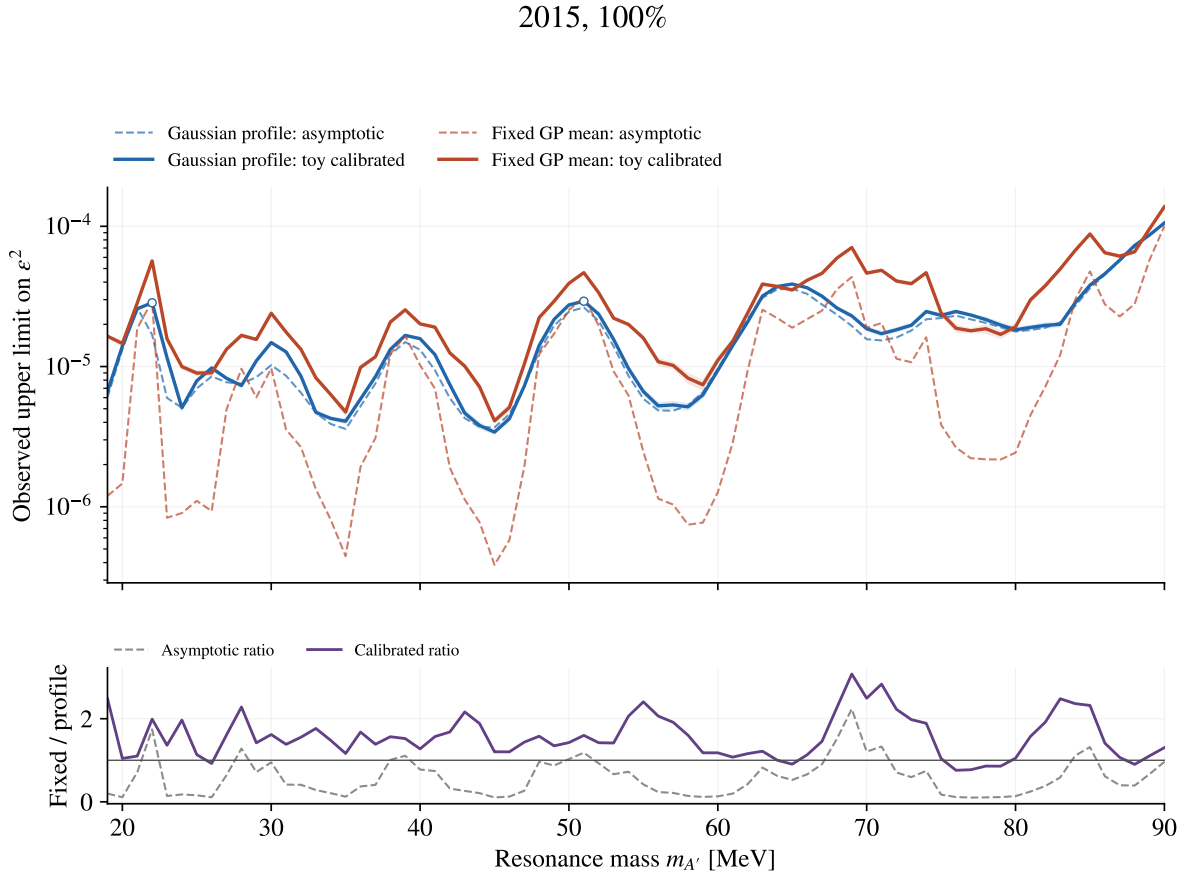
Figure 88: Observed asymptotic and calibrated 90% CL_s limits for 2015 using the two background treatments. Calibration envelopes cover the two stated generating shapes. Shading and open precision markers refer to finite Monte Carlo accuracy; they are not expected-limit bands.
