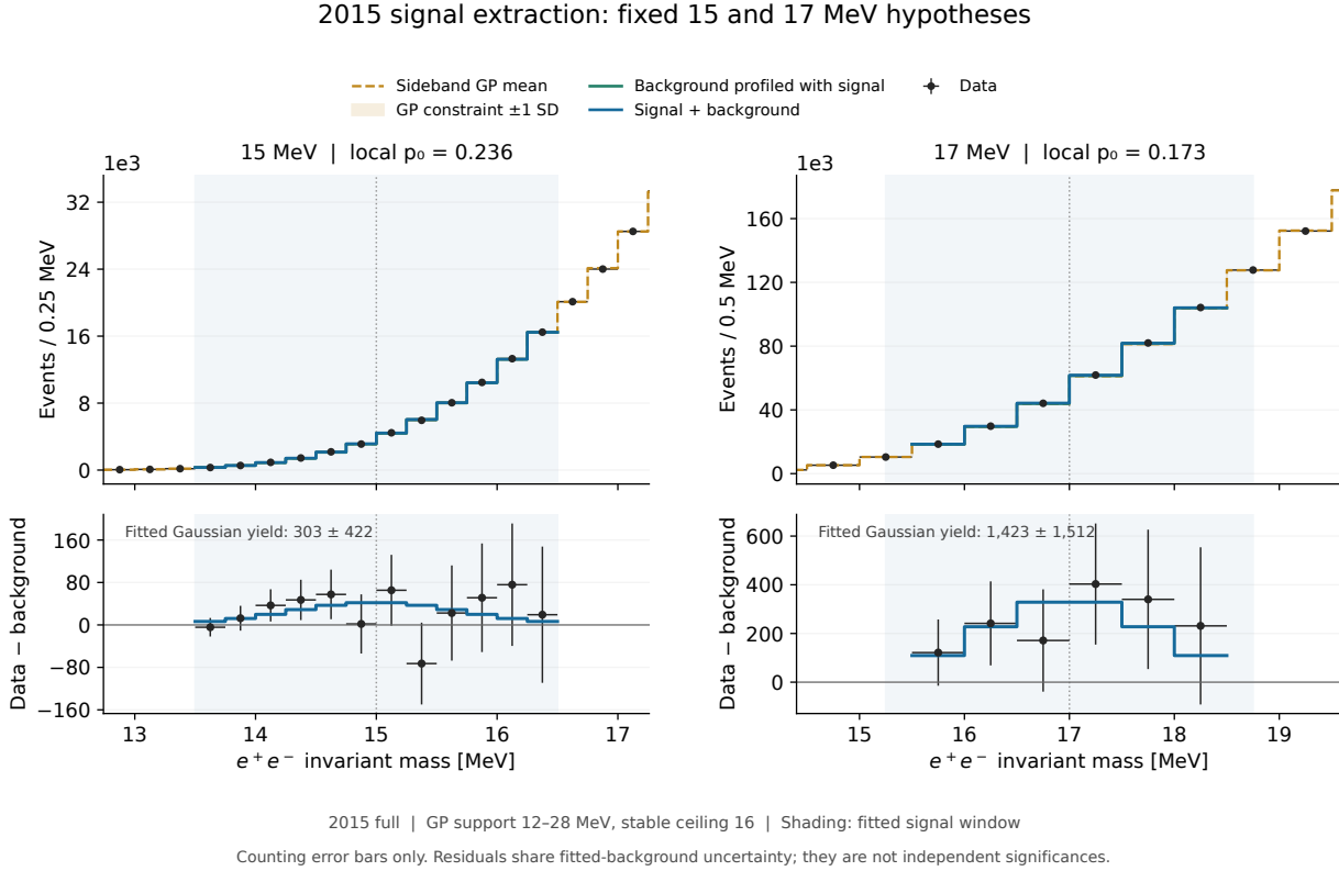
Figure 119: Fixed 15 and 17 MeV hypotheses. Top: data, sideband background constraint, profiled background and signal-plus-background prediction. Bottom: data minus the background profiled with signal, with the fitted Gaussian contribution. The error bars describe counting uncertainty only. The subtraction uses the same data to fit the background and is not an independent pull test.
