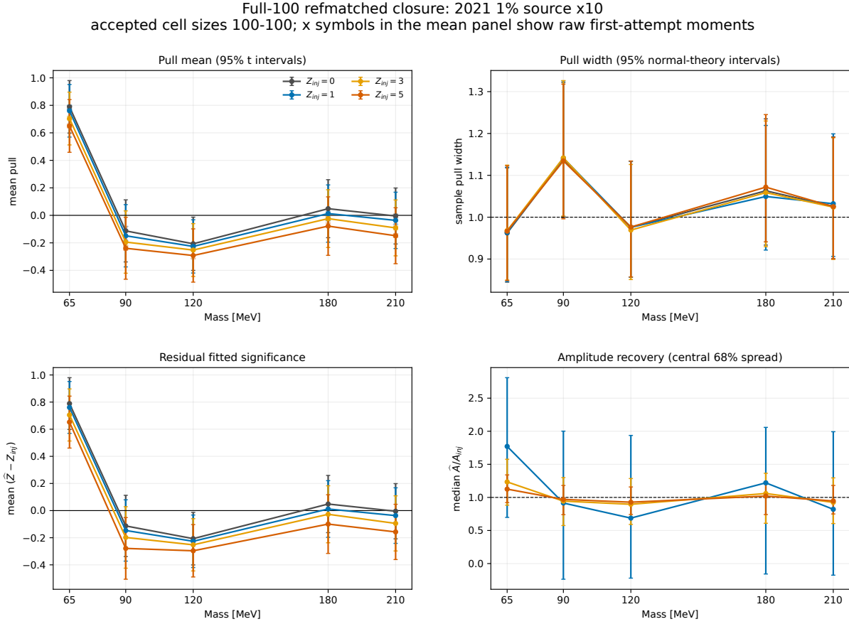
Figure 106: Full-100 refmatched closure for 1\% \times 10 . Every cell retains 100 accepted toys. The persistent positive 65 MeV pull means and the corresponding analytic-mean result are local stress-truth/model offsets; the other masses have near-unit widths and substantially smaller means. Crosses in the mean panel show raw first-attempt moments before the predeclared LML/reproducibility selection.
