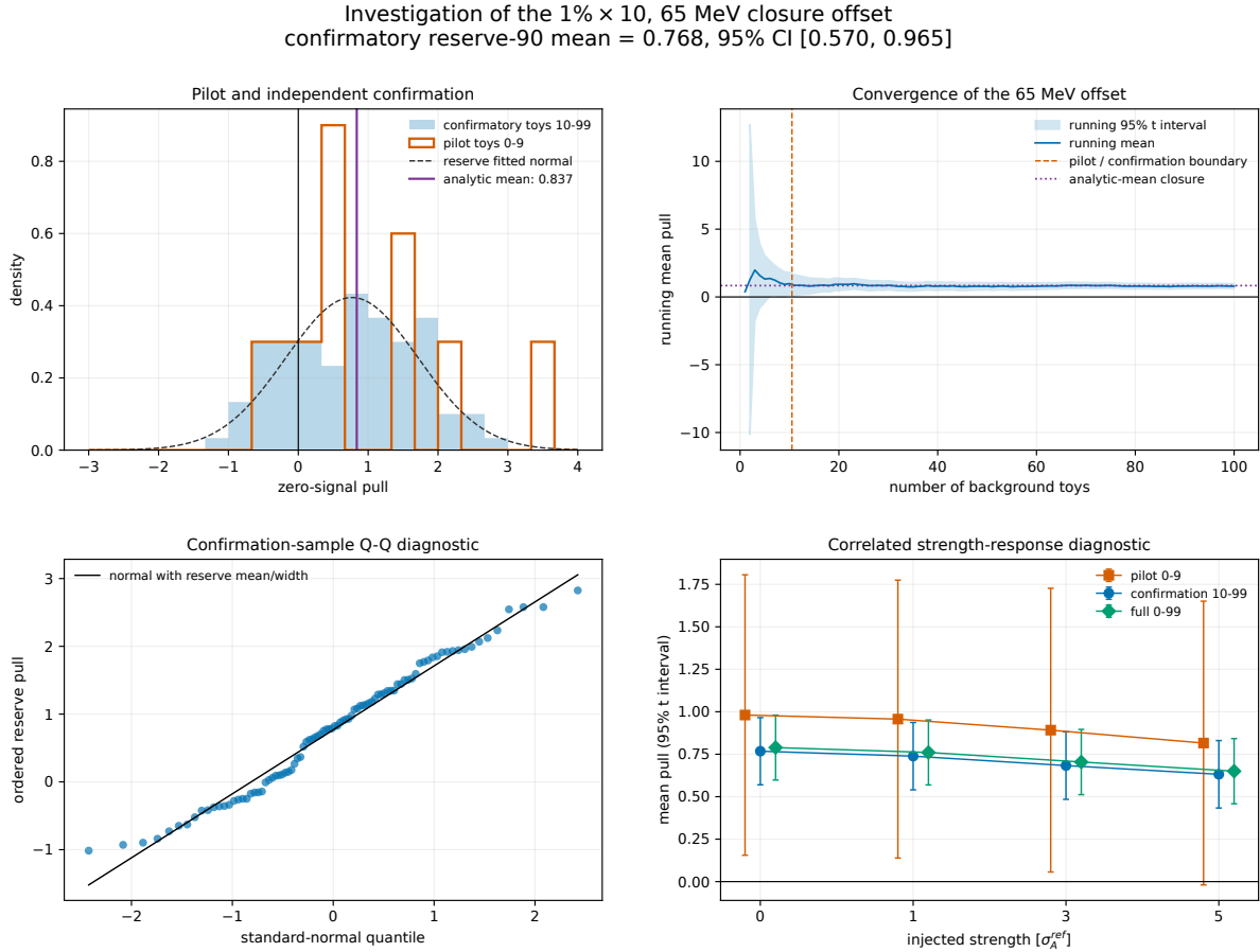
Figure 105: Investigation of the 1\% \times 10 , 65 MeV closure offset. The top-left panel separates the pilot and independent reserve distributions; the top-right tracks the running mean and its 95% Student- t interval, with the pilot/reserve boundary fixed at toy 10. The lower-left normal Q-Q diagnostic shows no isolated tail capable of explaining the mean, and the lower-right panel shows the correlated response across injection strengths. The analytic-mean pull of 0.837 was obtained from the exact stress-truth mean with independent optimizer seeds.
