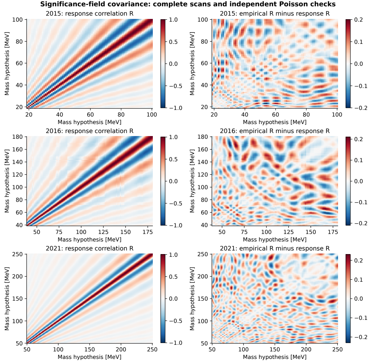
Figure 86: Response-predicted correlations and their empirical comparison using the same 256 complete background-only Poisson spectra at all coordinates. Each row uses its actual mass grid; difference panels have separate color scales. The original 1,000-scan native-grid result is retained separately and is not spliced into these extended matrices. This checks central dependence under the specified stress reference, not the rare global tail.
