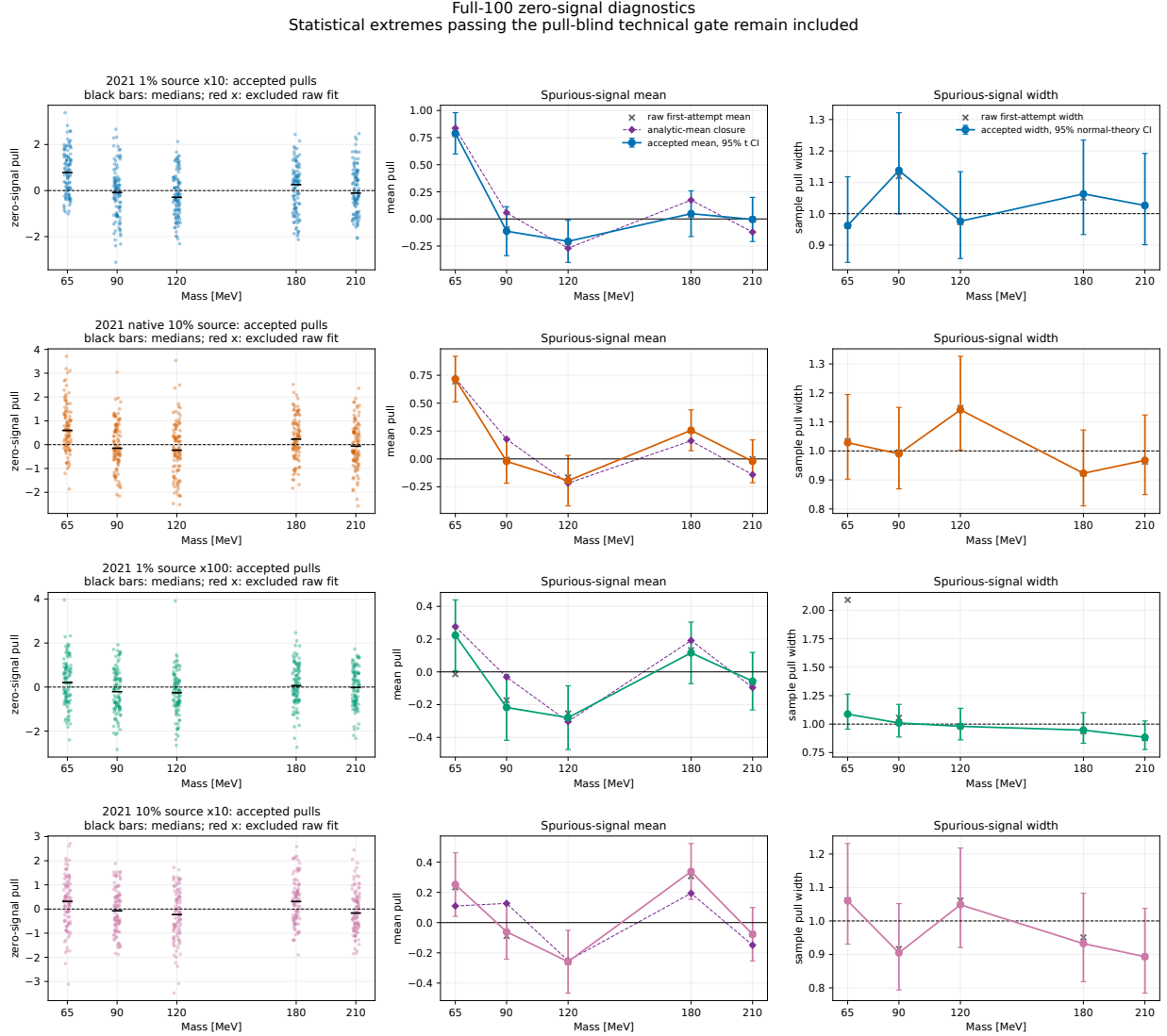
Figure 107: Full-100 spurious-signal study. Each row corresponds to one ensemble. The left panels show every accepted zero-signal pull and its median; the middle panels show raw first-attempt means, accepted means with 95% Student- t intervals, and the deterministic analytic-mean closure; the right panels show accepted sample widths with 95% normal-theory intervals. Red crosses mark excluded raw fit states where present. No accepted pull is clipped. The common mass dependence between analytic-mean and ensemble results diagnoses stress-truth/model closure rather than a statistical outlier.
