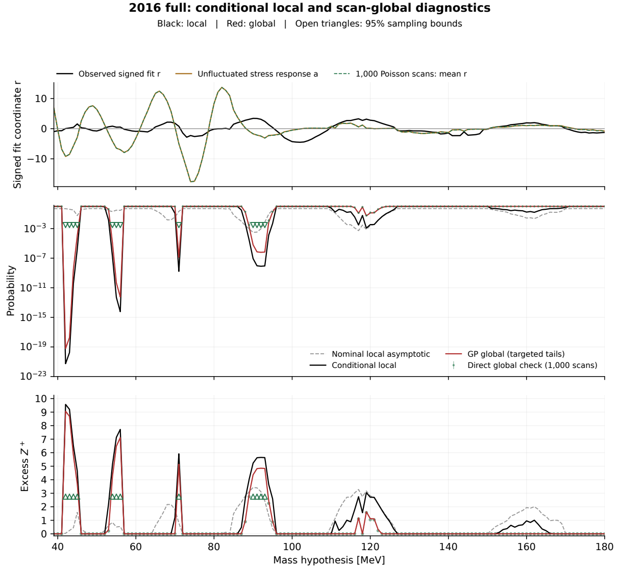
Figure 79: Profiled 2016 conditional global study with the same black-local/red-global convention and integer Z^+ guides. Ordinary sampling uses 2,000,000 fields; targeted importance sampling resolves the previously empty Gaussian tails without altering the field model or ordering. At 42 MeV the conditional Gaussian global probability is 6.096 \times 10^{-20} ( Z = 9.067 ), with 0.16% relative Monte Carlo standard error. This extreme value reflects the biased stress reference, not a particle discovery. The direct Poisson check remains 0/1,000, giving only p < 0.002991 ( Z > 2.749 ); its open triangles retain those bounds. Red shading gives sampling intervals, not background-model uncertainty. This global calculation is different from the Sidak reference.
