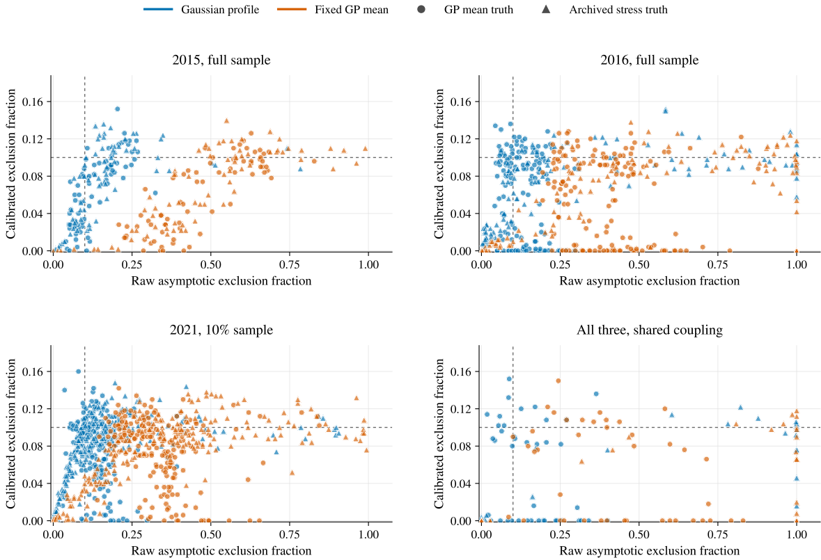
Figure 98: Independent validation with five-reference-error injections. The horizontal coordinate is the fraction of 500 spectra excluding the known injected yield with the raw asymptotic rule; the vertical coordinate uses the calibrated two-truth envelope. A point far to the right has an excessive raw exclusion rate. A point below the horizontal 0.10 guide indicates a conservative calibrated rate in that cell. The guides mark the nominal benchmark, not an expected discovery probability. Finite counts and Monte Carlo uncertainty limit the precision of each conclusion.
