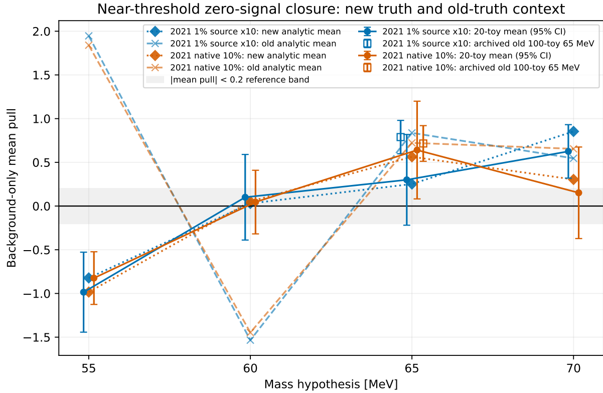
Figure 116: Historical 20-background near-threshold closure. Points carry 95% Student- t intervals; deterministic responses to the old and new analytic means expose the truth-shape dependence. The known 65 MeV response improves in the 1%-source test, while neighboring offsets remain. The later 100-background replacement results in the main text use their own identified truth and support; they are not pooled into these curves.
