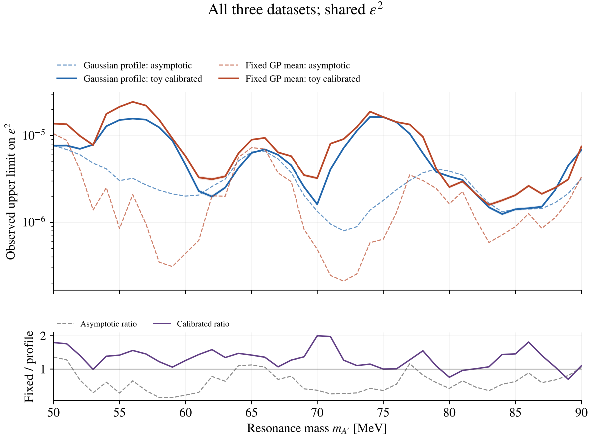
Figure 94: The three-dataset common-range comparison. This calibration covers 41 masses, rather than the later 232-mass union scan. It uses a shared physical coupling and either all local-GP or all archived-stress constituent backgrounds; mixed truth assignments are not included.
