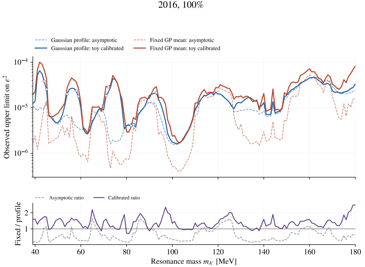
Figure 92: The same comparison for full 2016. The pronounced change is localized and depends on the archived stress construction. A resolved calibration endpoint does not remove the source-convergence qualifications or inherited numerical exception.
