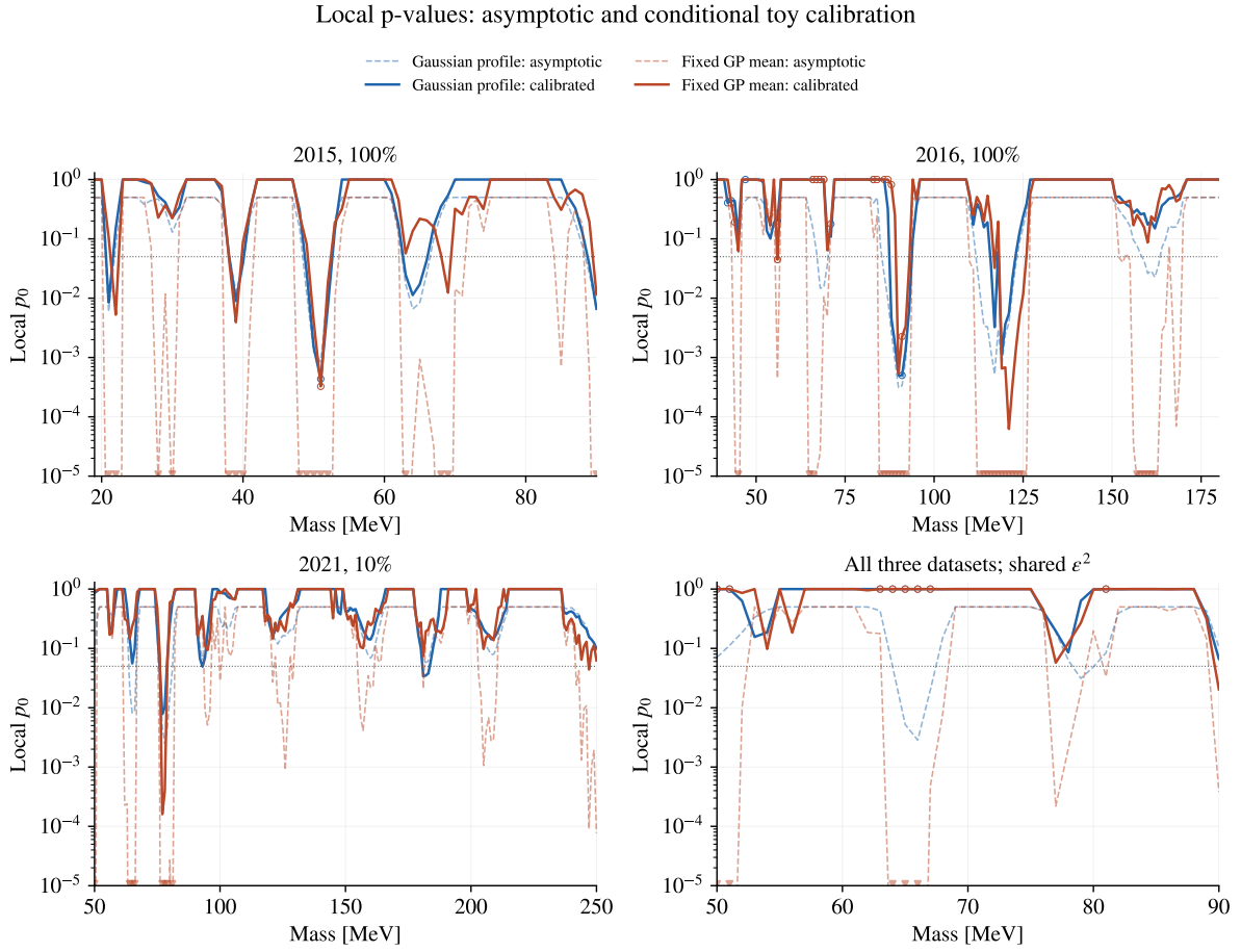
Figure 96: Asymptotic local probabilities and the larger background-only tail from the two calibration truths. The empirical bounded-statistic convention gives one when the discovery statistic is zero; the earlier asymptotic display gives 0.5. Triangles retain asymptotic values below the plotting floor. Open circles flag limited Monte Carlo precision or a noisy estimate displayed at one; numerical ledgers retain unclipped values. No curve in this figure includes a global trials correction.
