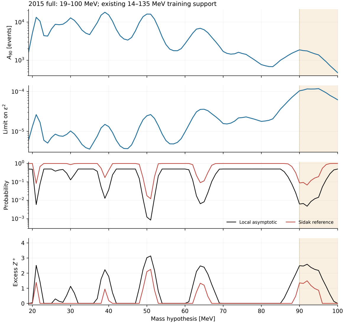
Figure 55: Observed 2015 full-sample scan on 19–100 MeV with 14–135 MeV GP support. From top to bottom: the 90% \text{CL}_s full-template signal-yield upper limit A_{90} , the corresponding \epsilon^2 upper limit, discovery probabilities, and aligned Z^+ values. The local asymptotic reference is black and the Sidak reference is red, with N_{\text{eff}} = 14.521 . At 51 MeV they give Z = 3.139 and Z_{\text{Sidak}} = 2.250 . The added 91–100 MeV fits use the fixed endpoint prescription; the shaded interval has the conditional status in Appendix B. The Sidak reference is distinct from the conditional GP global calculation in Section 6.11.
