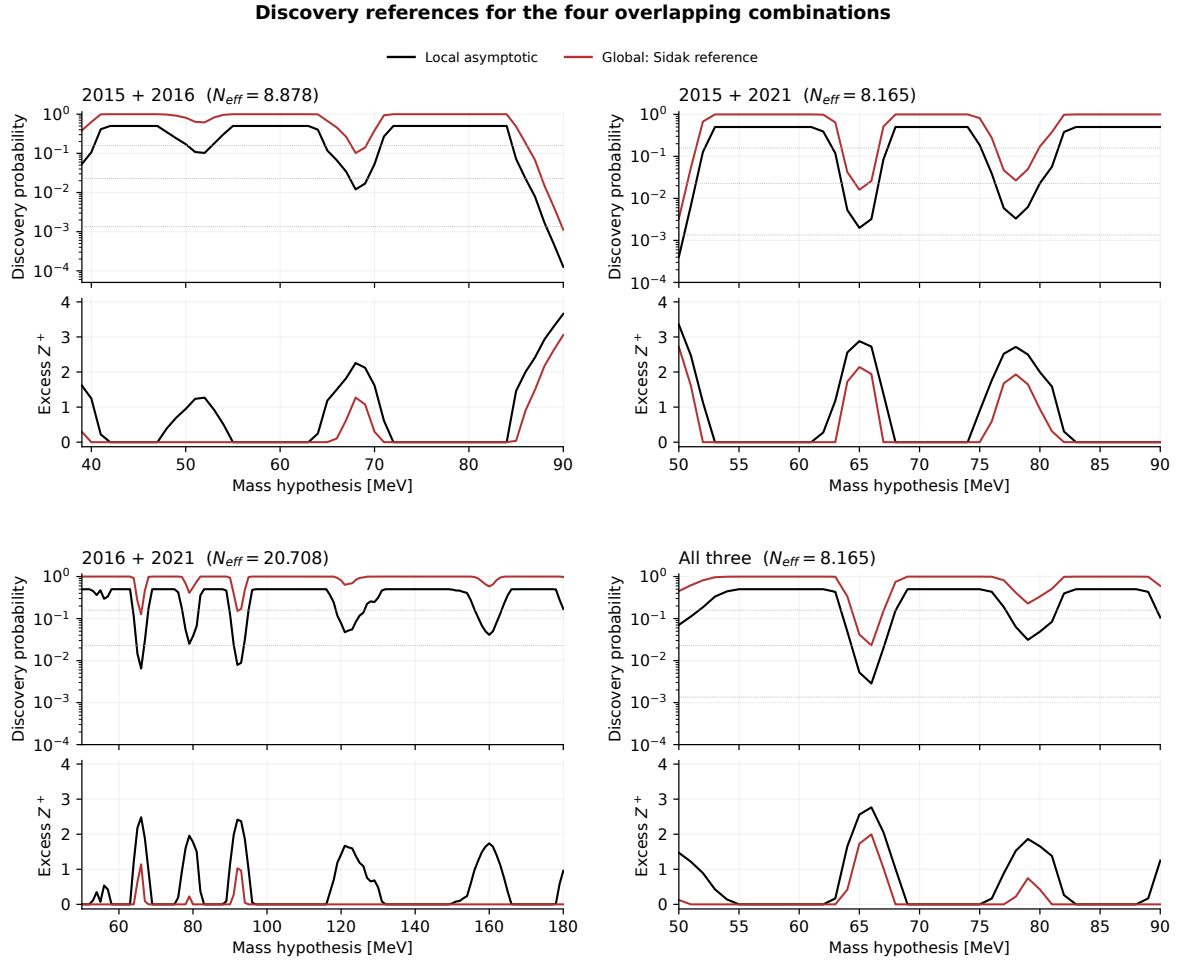
Figure 136: Historical parent Figure 84: combination discovery. This saved display uses the former 2015 endpoint of 90 MeV. The corresponding v5.0.4 result is Figure 82.
