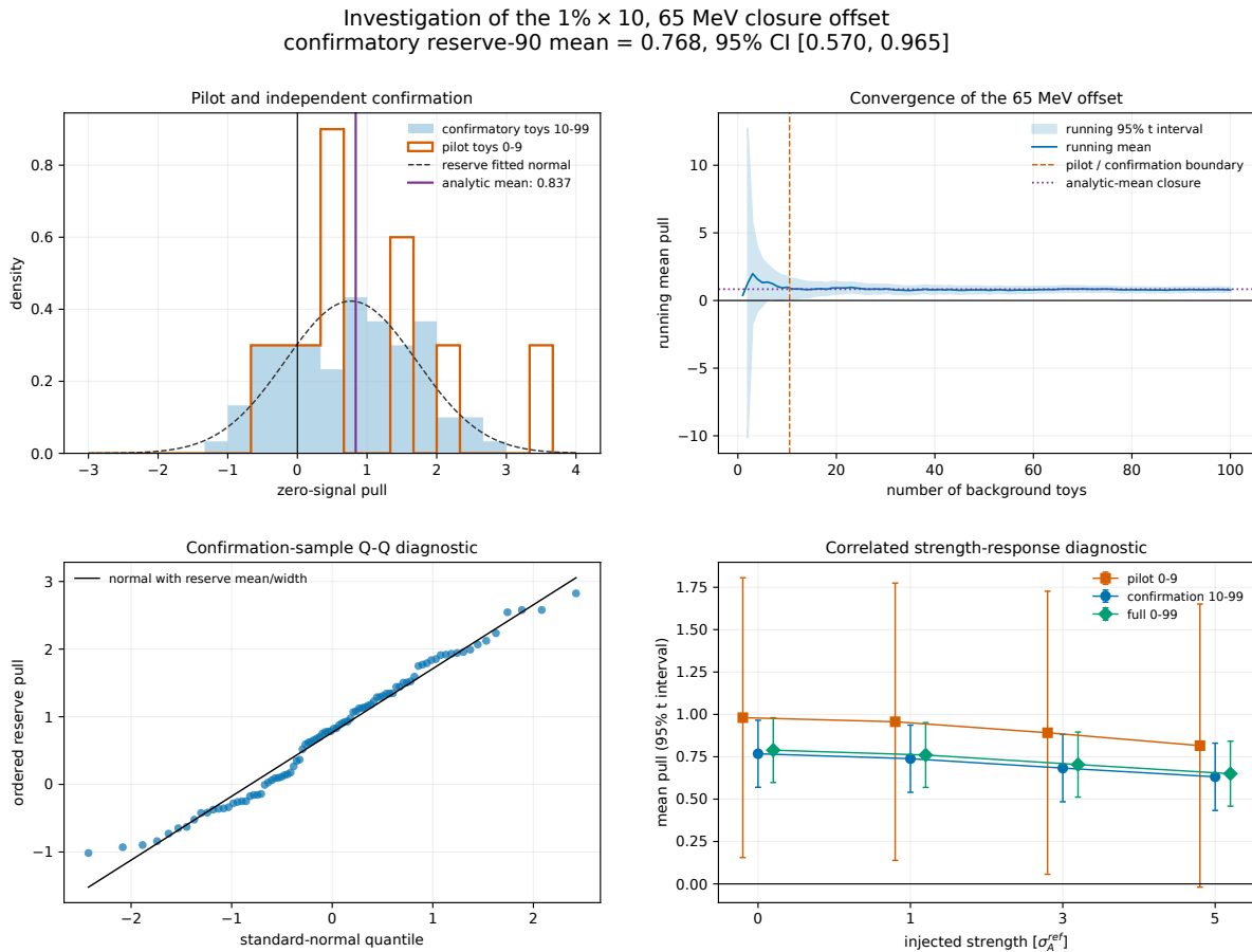
Figure 108: Investigation of the 1\% \times 10 , 65 MeV closure offset. The top-left panel separates the pilot and independent reserve distributions; the top-right tracks the running mean and its 95% Student- t interval, with the pilot/reserve boundary fixed at toy 10. The lower-left normal Q-Q diagnostic shows no isolated tail capable of explaining the mean, and the lower-right panel shows the correlated response across injection strengths. The analytic-mean pull of 0.837 was obtained from the exact stress-truth mean with independent optimizer seeds.
