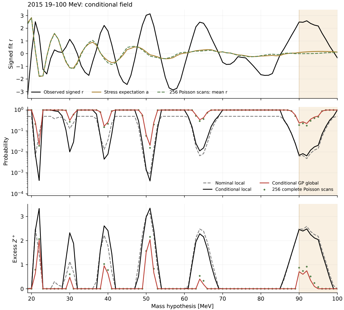
Figure 78: Profiled 2015 conditional local and global probabilities on 19–100 MeV. The full field uses 82 integer hypotheses and the endpoint kernel prescription in Appendix B. Its response matrix and the first 256 coherent Poisson scans are reused from the extended covariance study; 200,000 Gaussian fields integrate the enlarged search. Open symbols retain one-sided 95% bounds for empty direct tails. Probability and Z^+ panels refer to the declared stress model. The interpretation, sigcorr check and sampling method are in Appendix C.
