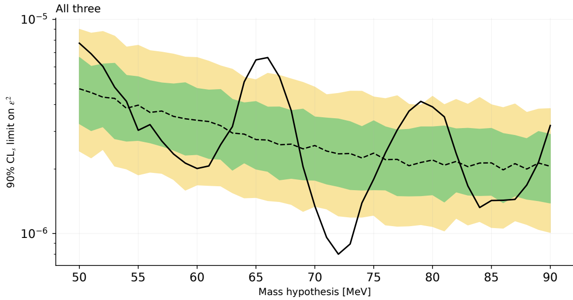
Figure 127: Historical parent Figure 60: all three expected bands. This saved display uses the former 2015 endpoint of 90 MeV. The corresponding v5.0.4 result is Figure 60.
