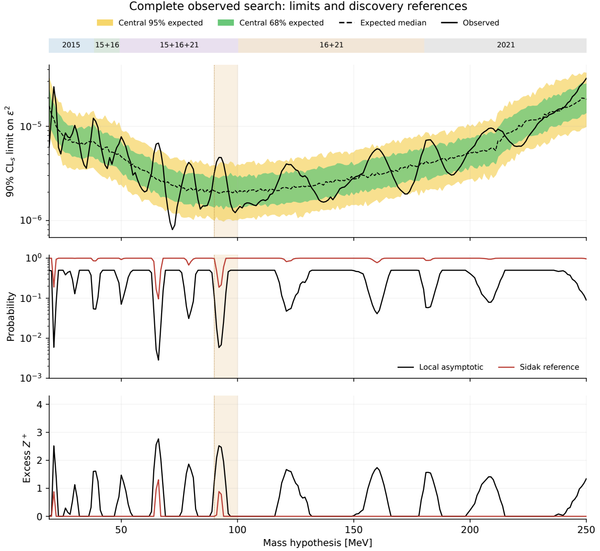
Figure 52: Complete 19–250 MeV observed search, with the preassigned active datasets shown above the curves. The upper panel shows 90% CL_s limits and the median, central 68% and central 95% ranges of the 300 conditional background-only toys per mass, with newly computed bands at the added 2015 coordinates. The next two panels show the fixed-mass asymptotic p_0 and its normal-quantile significance, with the local reference in black and the Sidak reference in red. The latter uses N_{\text{eff}} = 35.381 for the complete search; its value at 66 MeV is Z_{\text{Sidak}} = 1.305 , compared with local Z = 2.765 . The observed polyline connects every adjacent tested mass, including membership transitions; no numerical endpoint is changed by those connections. The physical visible-branching correction is applied once above the dimuon threshold. These are pointwise bands; 2016-inclusive values retain the numerical exception.
