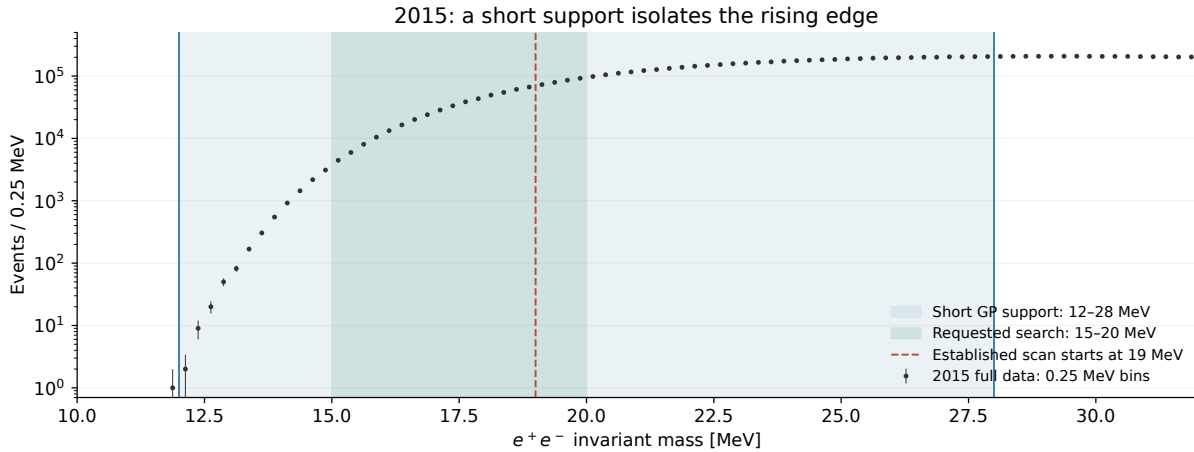
Figure 138: The same released full-2015 histogram, summed from 0.05 to 0.25 MeV bins. The chosen GP support is 12–28 MeV; the requested search is 15–20 MeV. The dashed line marks the lower boundary of the established scan, not the lower boundary of the available counts.
