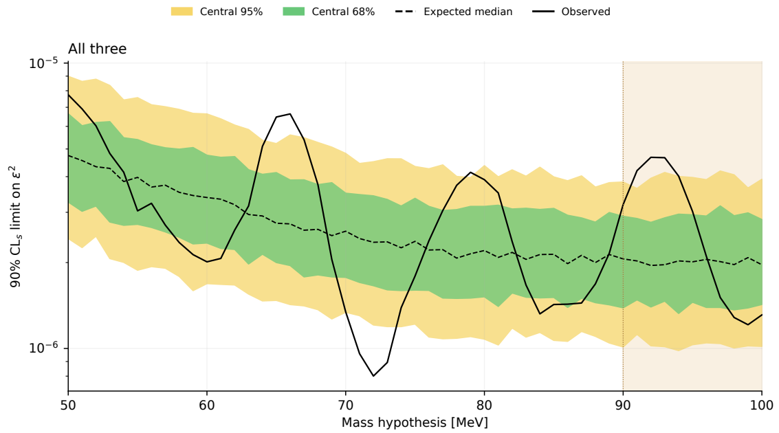
Figure 60: The all-three shared-coupling result on its common 50–100 MeV interval. Green and yellow show central 68% and 95% pointwise ranges, and the dashed curve is the median of 300 conditional background-only toys at each mass. The observed curve uses the same bounded asymptotic construction as the standalone fits.
