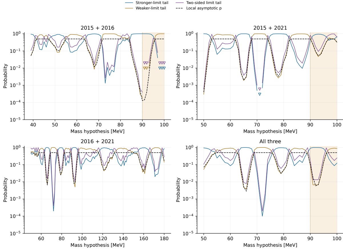
Figure 64: The same empirical limit-tail diagnostics for the pairwise and all-three combinations. Finite estimates and zero-count bounds remain visually distinct. Additional sampling can improve the precision of these conditional diagnostics, but cannot establish physical background validity or a discovery probability.
