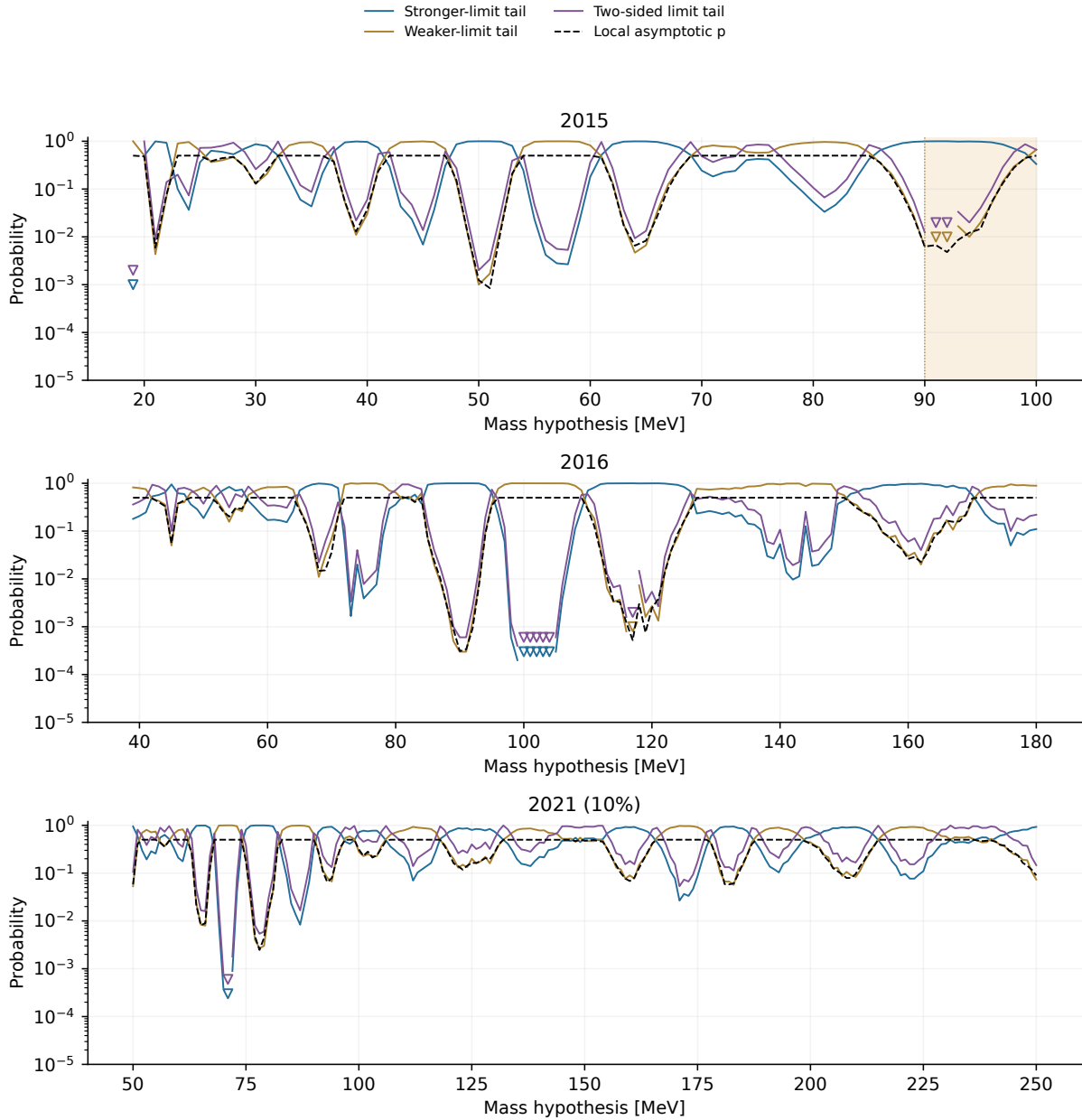
Figure 63: Empirical limit-tail diagnostics for each dataset. Unrefined points use 300 toys; selected coordinates use the saved independent 3,000- or 10,000-toy batches. The newly added 2015 masses use 300 toys and the same bound convention. Open downward triangles show one-sided 95% Monte Carlo upper bounds when no tail event is observed; for the two-sided diagnostic the bound is doubled and capped at one. These probabilities refer to the upper-limit statistic and are distinct from local asymptotic p_0 .
