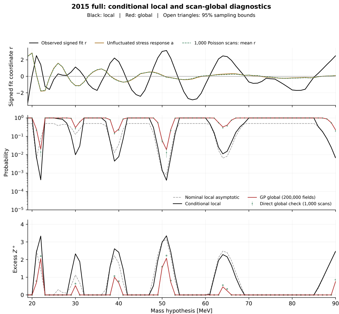
Figure 134: Historical parent Figure 78: global probabilities 2015. This saved display uses the former 2015 endpoint of 90 MeV. The corresponding v5.0.4 result is Figure 78.
