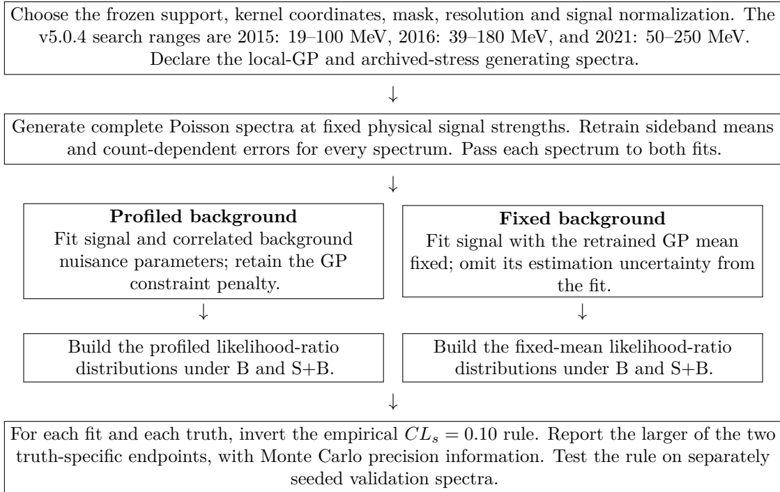
Figure 90: How the two background treatments are calibrated. Both branches receive identical spectra. The primary comparison uses two declared background truths for each method; it does not average the two methods or select whichever gives the tighter observed limit. B denotes background only and S+B denotes signal plus background. The displayed protocol can be applied over the new 2015 range; the archived two-truth calibration results below retain their original tested masses. The 300-toy extension bands in Appendix B do not by themselves execute this two-truth calibration.
