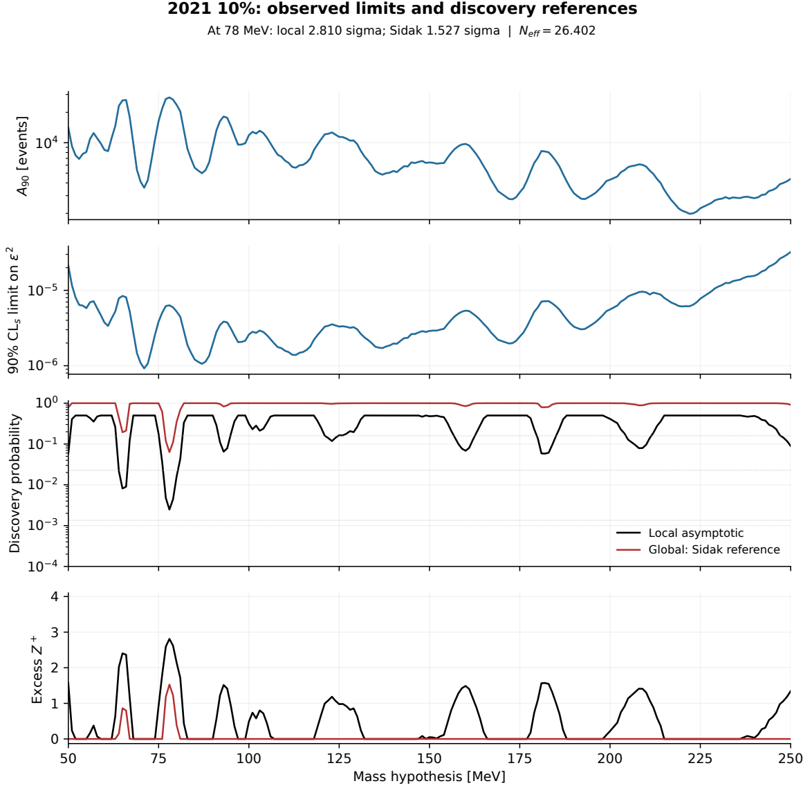
Figure 57: Corresponding observed 2021 10% scan on 50–250 MeV with 36–300 MeV GP support. The panels show the full-template A_{90} , minimal-visible \epsilon^2 limit, discovery probabilities, and aligned Z^+ values. Black is local and red is the Sidak reference with N_{\text{eff}} = 26.402 ; their values at 78 MeV are 2.810 and 1.527. Above the dimuon threshold the inherited branching correction enters the coupling conversion once; it does not change the visible electron-pair yield or local probability.
