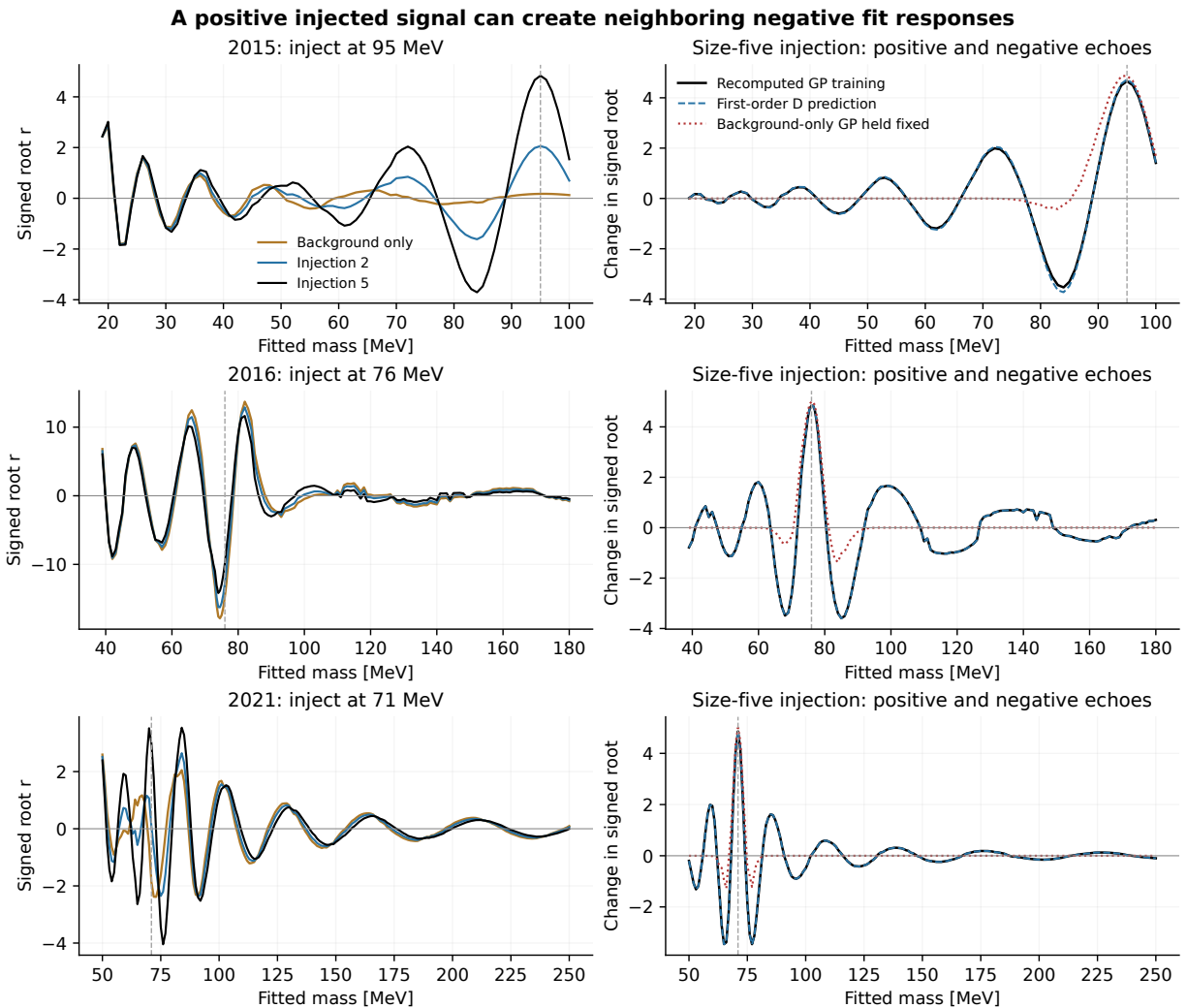
Figure 83: Deterministic signal injections into the coherent stress spectrum. Left: signed roots before and after injection. Right: the size-five change with full retraining, its first-order template projection, and a control holding the background-only GP prediction and covariance fixed. The likelihood’s background nuisance parameters remain profiled in the last control. Vertical lines mark the injected mass. Neighboring negative responses are retained. These full scans contain no Poisson fluctuation.
