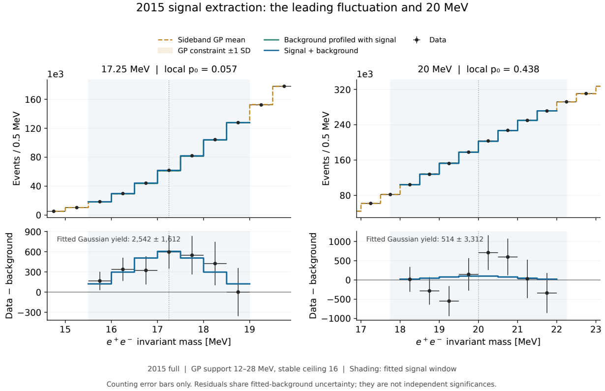
Figure 141: The selected 17.25 MeV upward fluctuation and the fixed 20 MeV hypothesis, with the same conventions and fixed-phase grouping as the preceding displays. Their local asymptotic roots are 1.58 and 0.16. A convincing resonance would need a stable excess across defensible background choices and a validated accepted signal shape.
