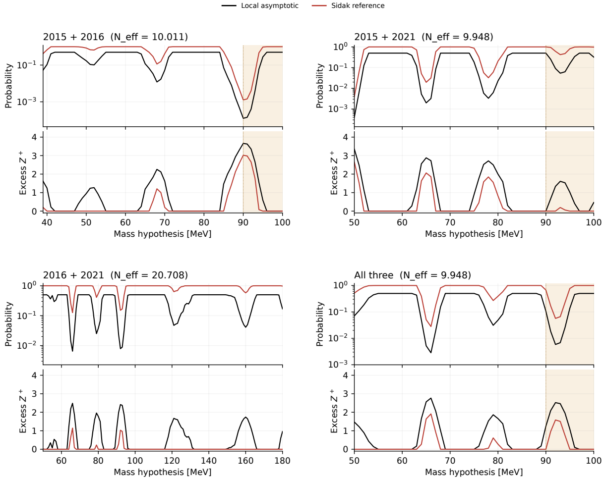
Figure 82: Discovery probabilities and aligned Z^+ values for all four overlapping combinations. Local asymptotic curves are black and Sidak global references are red. Each pair of panels shares its mass axis and uses one fixed N_{\text{eff}} over that scope's full overlap, now through 100 MeV whenever 2015 participates. The 90–100 MeV extension is shaded. These are analytic Sidak references, distinct from the stress-centered correlated-field global probabilities above; no additional correction for selecting among overlapping scopes is included.
