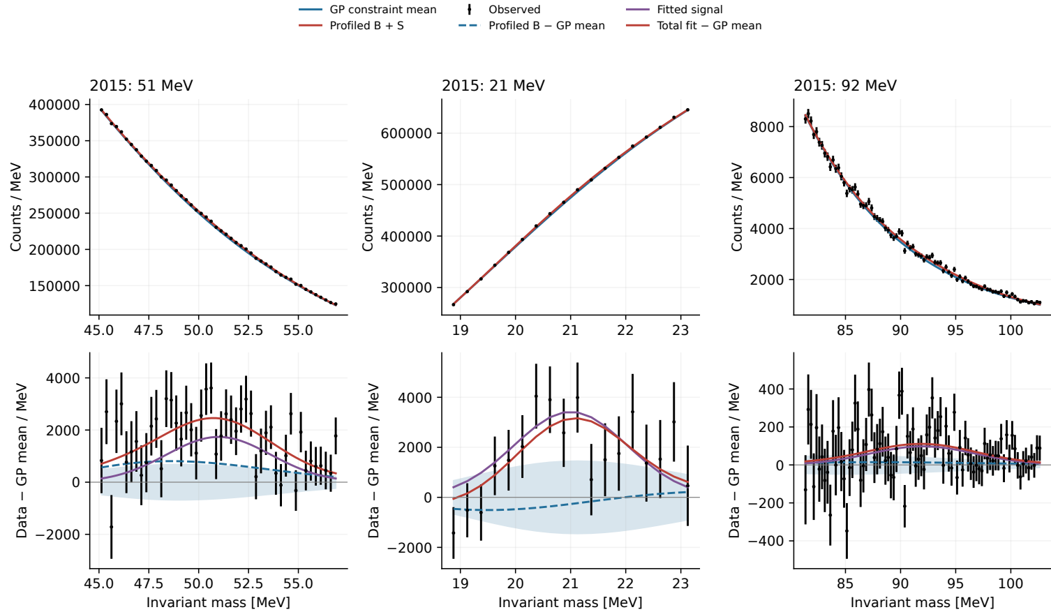
Figure 70: The earlier separated 2015 regions at 51 and 21 MeV, with the added 92 MeV region from the extension. The 21 MeV feature is close to the lower search endpoint. All residuals subtract the unprofiled GP mean; the fitted signal, the background displacement and their sum are shown separately. Bars show counting errors and shading shows the GP constraint width, not a post-fit signal confidence band. The 92 MeV panel is an individual 2015 fit; its preferred amplitude differs from the common-rate extraction in Figure 68.
