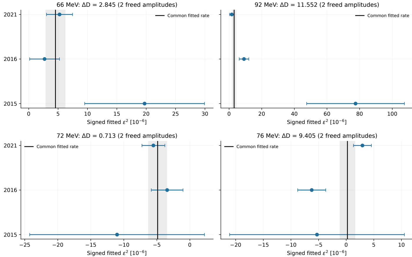
Figure 84: Separate campaign coupling estimates with local curvature errors and the common fitted rate at 66, 92, 72 and 76 MeV. All three campaigns now enter every comparison. At 92 MeV the common fit gives \hat{\varepsilon}^2 = 3.096 \times 10^{-6} ; freeing the three rates lowers twice the negative log likelihood by 11.552, compared with 2.845 at 66 MeV. The shaded band is the common fit's local curvature interval. These selected comparisons are descriptive; the errors are not post-selection intervals and no unadjusted compatibility probability is assigned.
