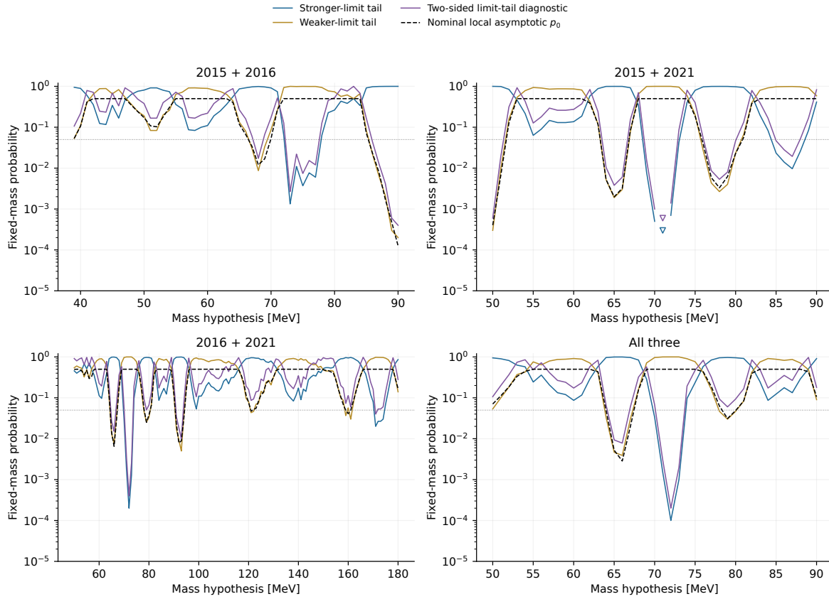
Figure 131: Historical parent Figure 64: combination tail probabilities. This saved display uses the former 2015 endpoint of 90 MeV. The corresponding v5.0.4 result is Figure 64.
