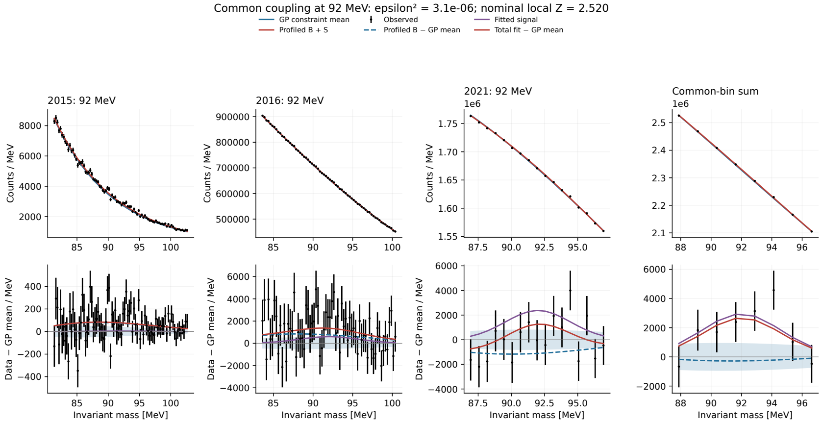
Figure 68: The 92 MeV common-coupling fit now includes 2015, 2016 and 2021. It gives \hat{\epsilon}^2 = 3.096 \times 10^{-6} and nominal local Z = 2.520 . Top: observed counts, sideband GP mean and profiled signal-plus-background prediction. Bottom: observed counts minus that same unprofiled GP mean, with the fitted signal, the profiled-background shift, and their sum displayed separately. The last column sums common whole bins from the three campaigns and has no separate fit. Counting errors and the zero-centered GP constraint band omit post-fit covariance. The large standalone 2015 preferred rate is not the signal height imposed by this common fit; Section 6.12 explains the comparison.
