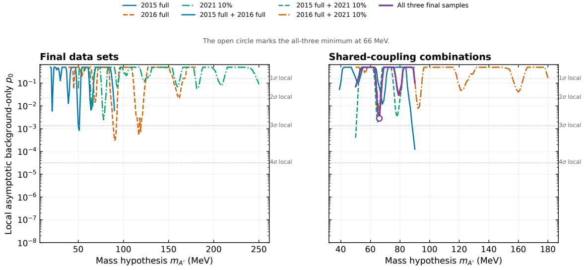
Figure 126: Historical parent Figure 59: final asymptotic pvalues. This saved display uses the former 2015 endpoint of 90 MeV. The corresponding v5.0.4 result is Figure 59.
