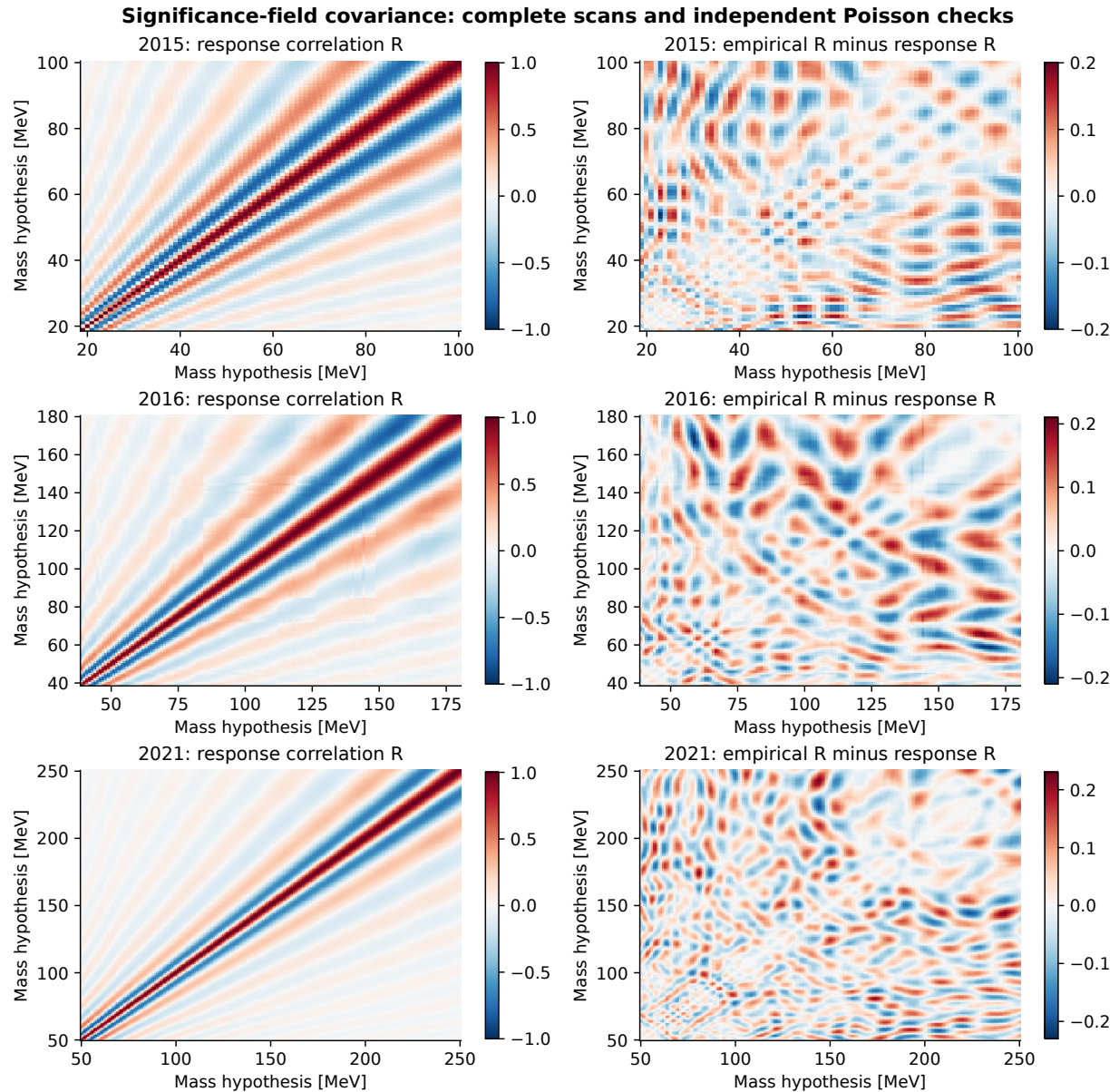
Figure 88: Response-predicted correlations and their empirical comparison using the same 256 complete background-only Poisson spectra at all coordinates. Each row uses its actual mass grid; difference panels have separate color scales. The original 1,000-scan native-grid result is retained separately and is not spliced into these extended matrices. This checks central dependence under the specified stress reference, not the rare global tail.
