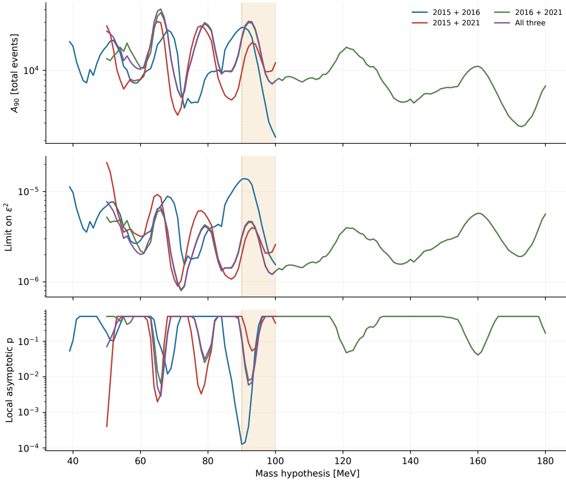
Figure 58: Observed shared- \varepsilon^2 results for the three pairwise combinations and the all-three overlap. For visual alignment, the top coordinate expresses the shared-coupling limit as the total compatible signal yield summed over the active campaigns. The middle panel gives the 90% bounded, piecewise-asymptotic \text{CL}_s upper limit on \varepsilon^2 , and the bottom panel gives the local asymptotic p_0 . The 2015-containing overlaps extend through 100 MeV. The shaded interval marks the extension described in Appendix B. No expected-limit bands are shown.
