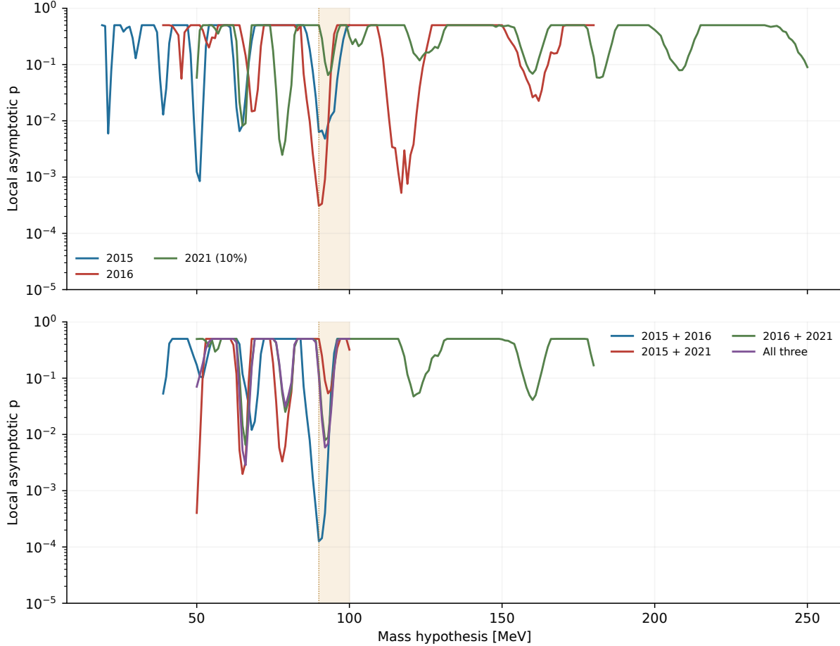
Figure 59: Local one-sided asymptotic background-only p_0 for the three standalone inputs, the three pairs, and the all-three combination. The values are conditional on the frozen GP supports and states. No look-elsewhere correction, global significance, or toy calibration is supplied by these curves. The 2015-containing scopes include 91–100 MeV.
