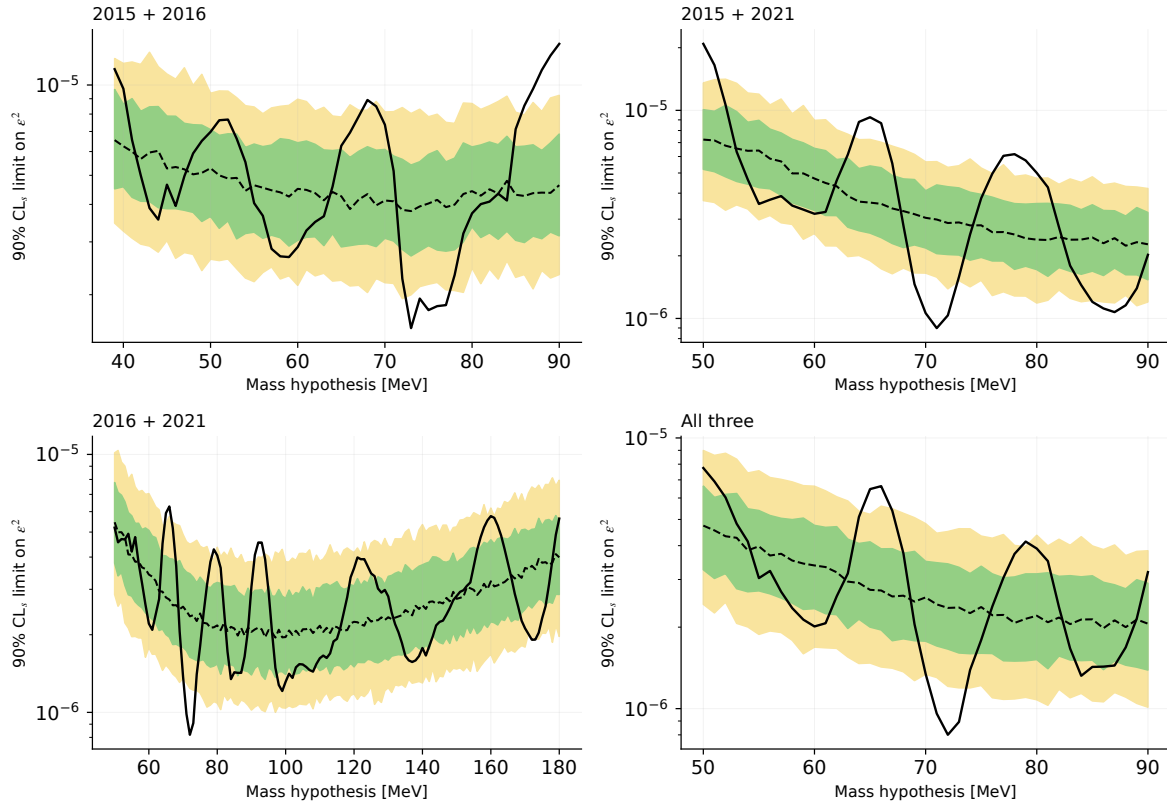
Figure 128: Historical parent Figure 61: combination expected bands. This saved display uses the former 2015 endpoint of 90 MeV. The corresponding v5.0.4 result is Figure 61.
