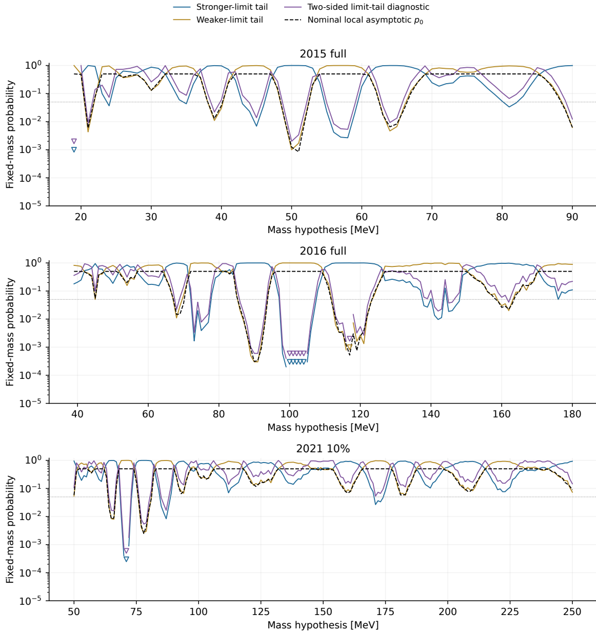
Figure 130: Historical parent Figure 63: individual tail probabilities. This saved display uses the former 2015 endpoint of 90 MeV. The corresponding v5.0.4 result is Figure 63.
