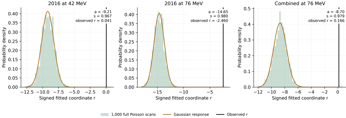
Figure 85: Representative background-only distributions from the saved 1,000 complete Poisson scans. Green histograms show the signed fitted coordinate, gold curves the unfluctuated-response Gaussian approximation, and black lines the observed fit. These panels show why the apparently large centered scores at 2016 42 MeV and combined 76 MeV can coexist with nearly zero raw observed fits. At 2016 76 MeV the observed fit is negative and is excluded by the positive-fit gate. Agreement of the histograms with the gold curves tests the approximation under that reference, not the physical correctness of the reference spectrum.
