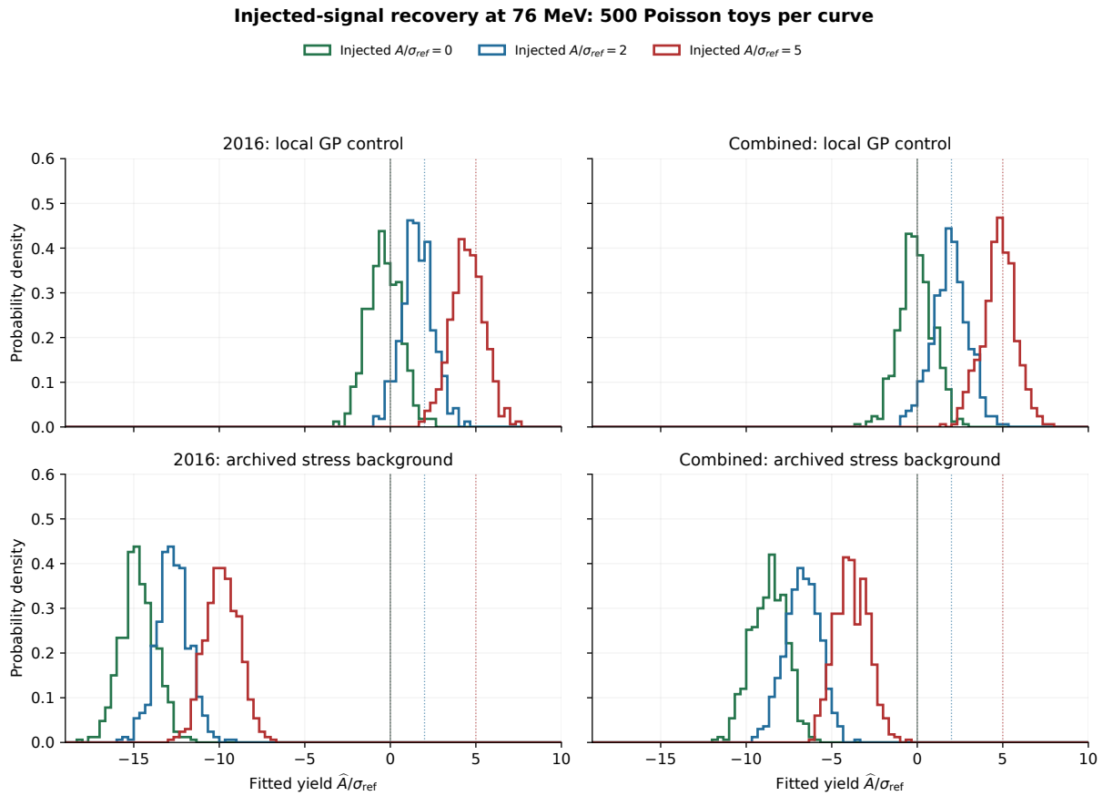
Figure 86: Saved 76 MeV signal-injection experiments, with identical axes for the local-GP controls (top) and archived stress backgrounds (bottom). Each curve has 500 independent Poisson spectra; dotted vertical guides mark the true injected yields 0, 2, 5 in units of that scope’s fixed \sigma_{\text{ref}} . The distributions move with injection, but the stress-background bias persists. These fitted-yield distributions show recovery and its failure mode explicitly; injection size five does not mean a measured 5\sigma signal. No new injection toys were generated for this display.
