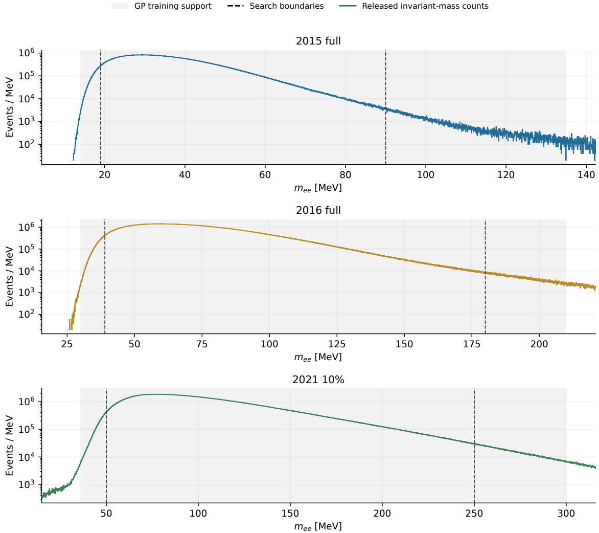
Figure 120: Historical parent Figure 7: dataset mass distributions log. This saved display uses the former 2015 endpoint of 90 MeV. The corresponding v5.0.4 result is Figure 7.
