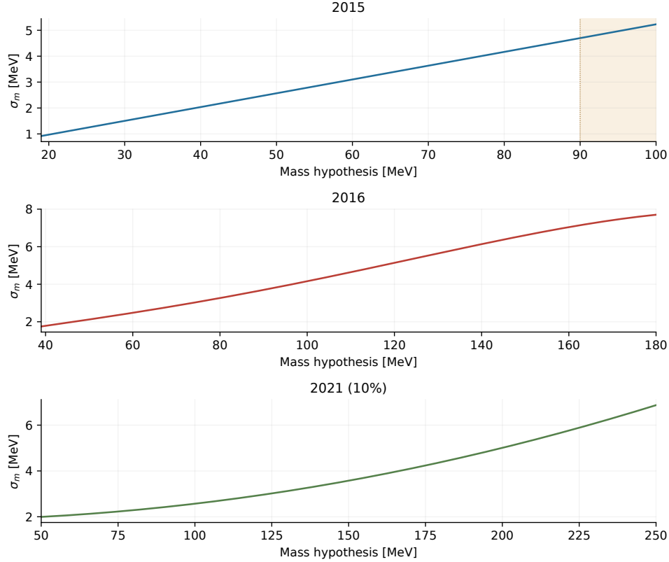
Figure 18: Mass-resolution parameterizations used by the analysis over the adopted scan ranges. The 2016 scan ends at the polynomial boundary of 180 MeV, so its configured high-mass continuation is not used. The 2021 panel shows the target-constrained V0 parameterization after multiplication by the TC smearing scale s_{\text{TC}} = 2.186/1.745 \simeq 1.25 and extended to 250 MeV.
