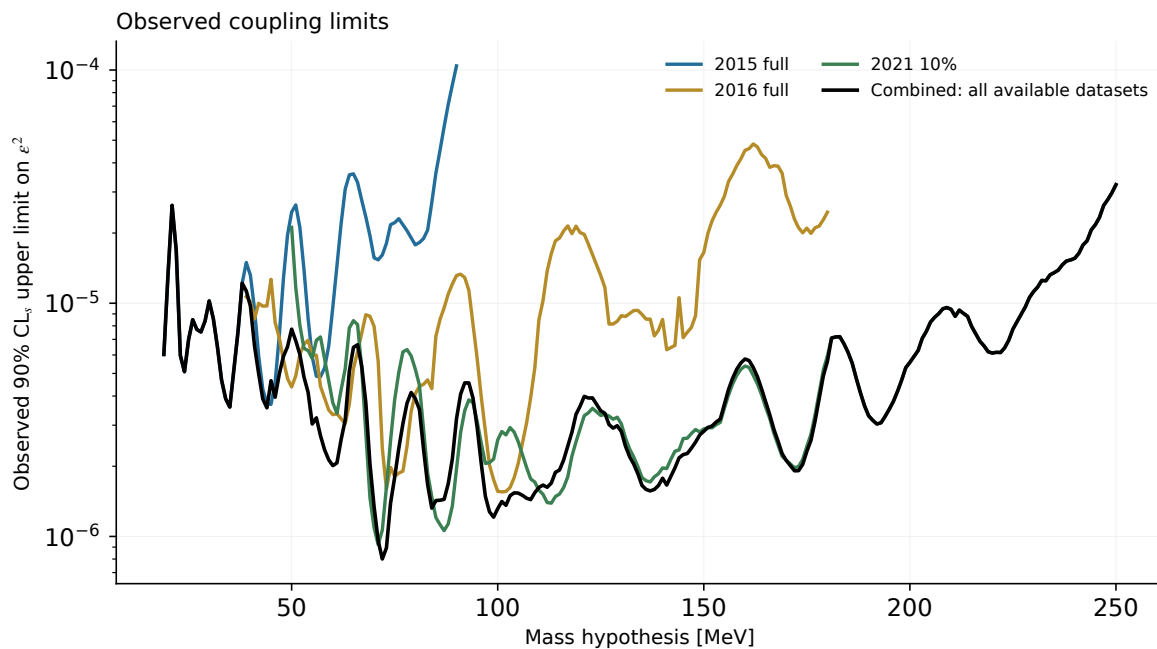
Figure 122: Historical parent Figure 53: observed coupling overlay. This saved display uses the former 2015 endpoint of 90 MeV. The corresponding v5.0.4 result is Figure 53.
