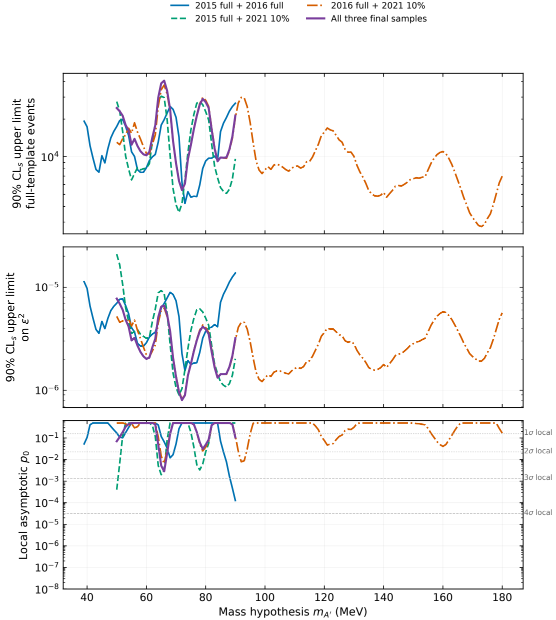
Figure 125: Historical parent Figure 58: combined final results. This saved display uses the former 2015 endpoint of 90 MeV. The corresponding v5.0.4 result is Figure 58.
