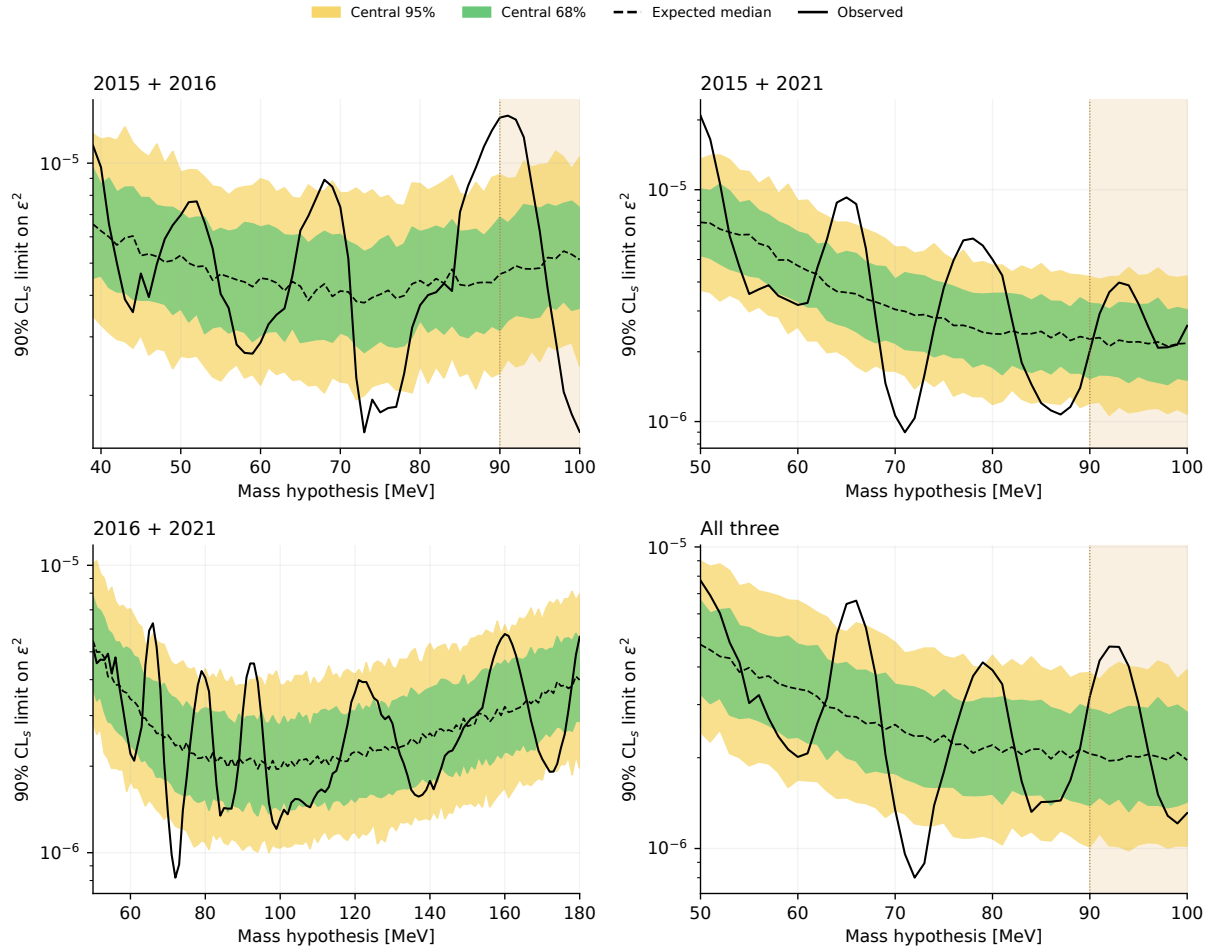
Figure 61: Pairwise and all-three results with the same conditional 300-toy pointwise bands. Comparisons at a given mass use paired constituent draws. Correlation between these panels does not supply correlation between separate mass hypotheses.
