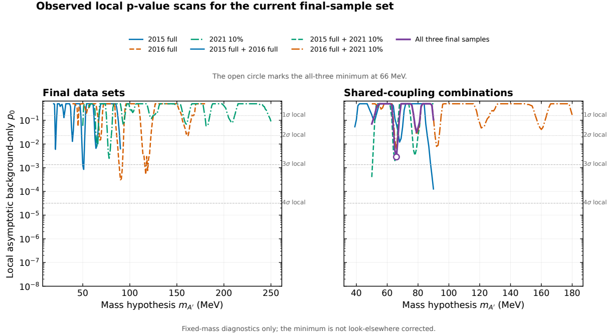
Figure 32: Local one-sided asymptotic background-only p_0 for the three standalone inputs, the three pairs, and the all-three combination. The values are conditional on the frozen GP supports and states. No look-elsewhere correction, global significance, or toy calibration is reported.
