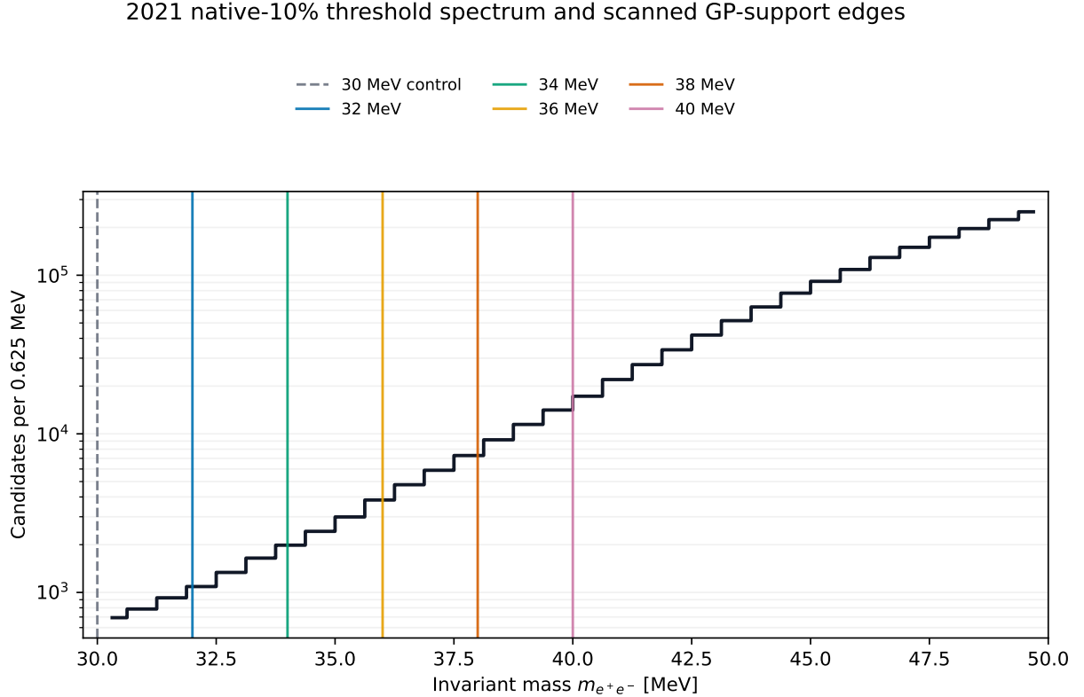
Figure 28: Native 2021 10% source histogram near threshold. Vertical lines mark the 30 MeV control and the five candidate lower edges of the GP support. The logarithmic vertical scale makes the low-count shoulder and rapid turn-on visible.
