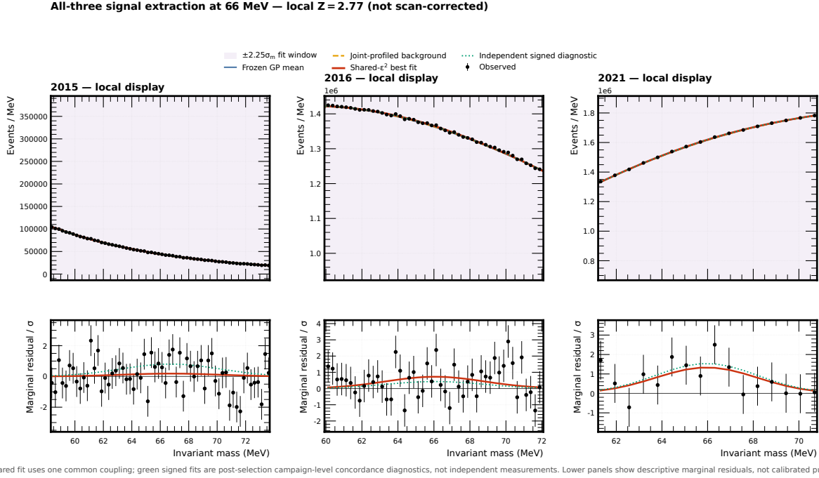
Figure 33: Signal extraction at 66 MeV, the mass hypothesis with the smallest local asymptotic p_0 in the all-three scan. The panels show full 2015, full 2016, and the 2021 10% sample with their frozen GP background descriptions and the signal contribution from the shared- \epsilon^2 profile fit. The quoted p_0 and Z are local asymptotic diagnostics, not a scan-calibrated discovery claim.
