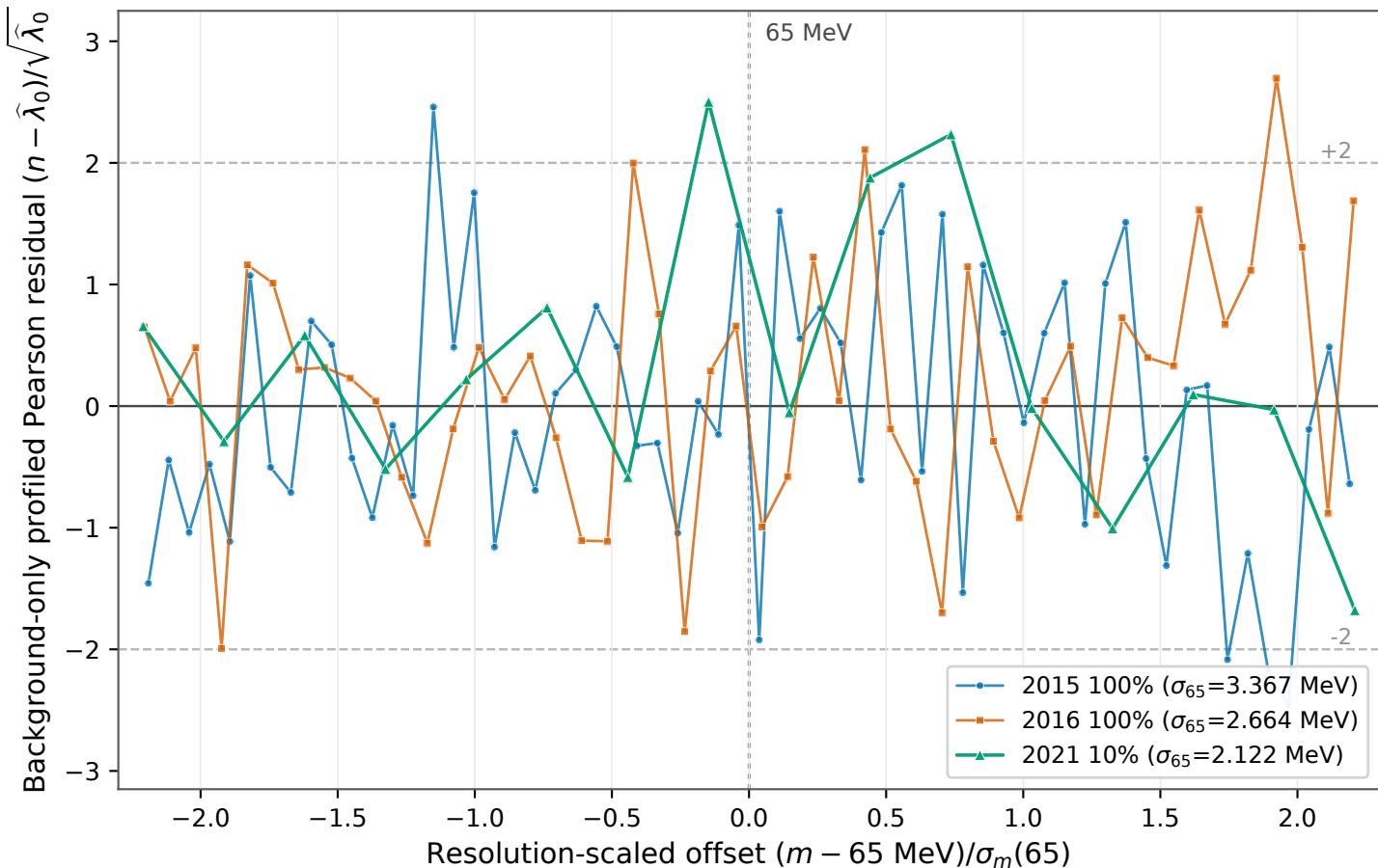
Profiled residuals aligned at the 65 MeV hypothesis
