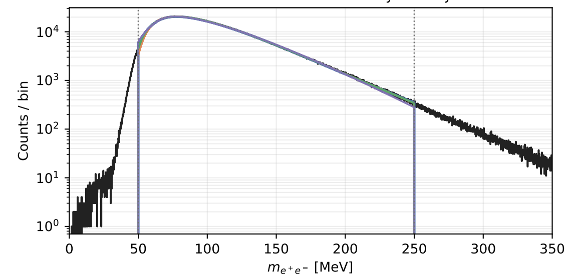
HPS 2021 1% candidate-family overlay
