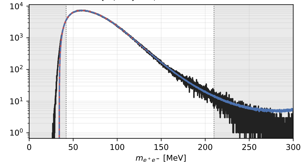
HPS 2016 10% / shifted sigmoid*power*exp + tail Scan [42, 210] MeV / N events = 7.483e+06
