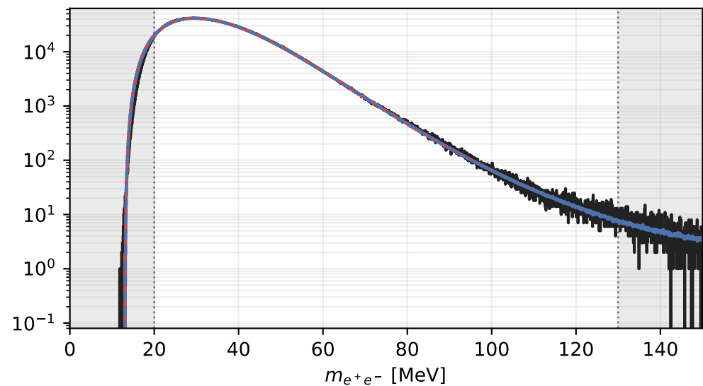
HPS 2015 / shifted sigmoid*power*exp + tail Scan [20, 130] MeV / N events = 2.145e+07
