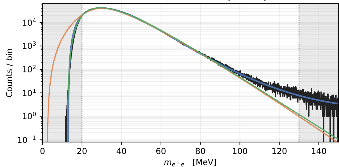
HPS 2015 candidate-family overlay
