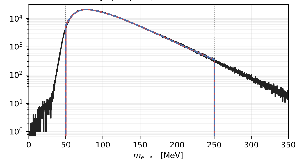
HPS 2021 1% / sigmoid*power*exp + raw expquad Scan [50, 250] MeV / N events = 1.229e+07
