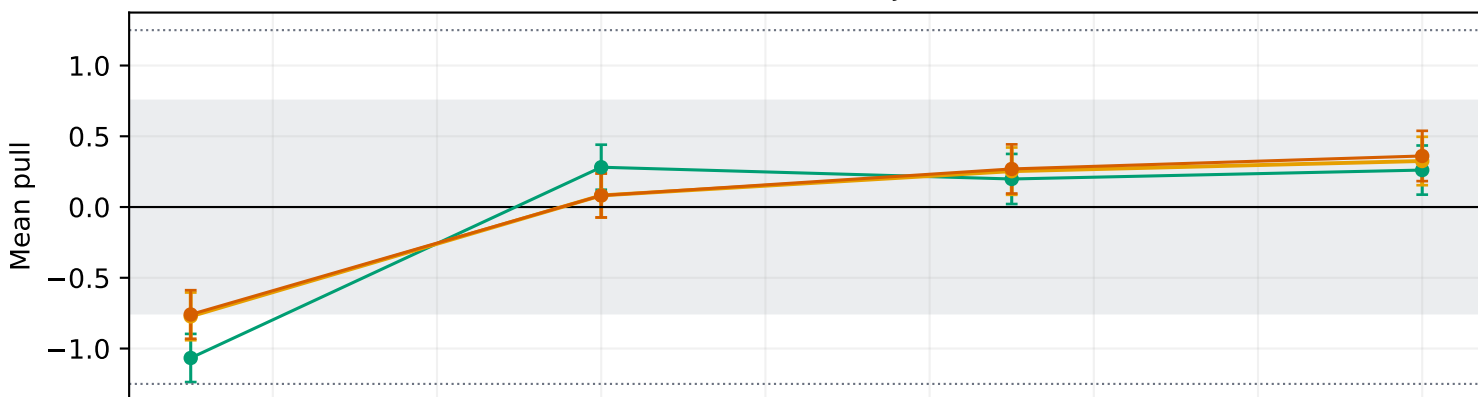
Matched-reference injection: 0\sigma
