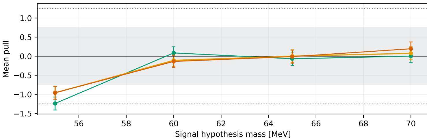
Matched-reference injection: 5\sigma
