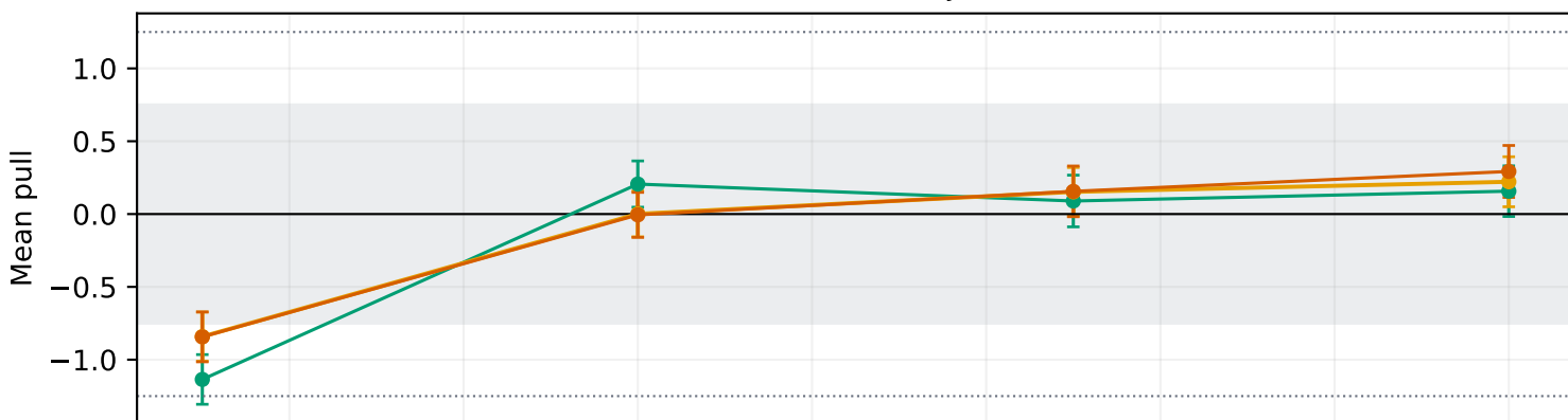
Matched-reference injection: 2\sigma
