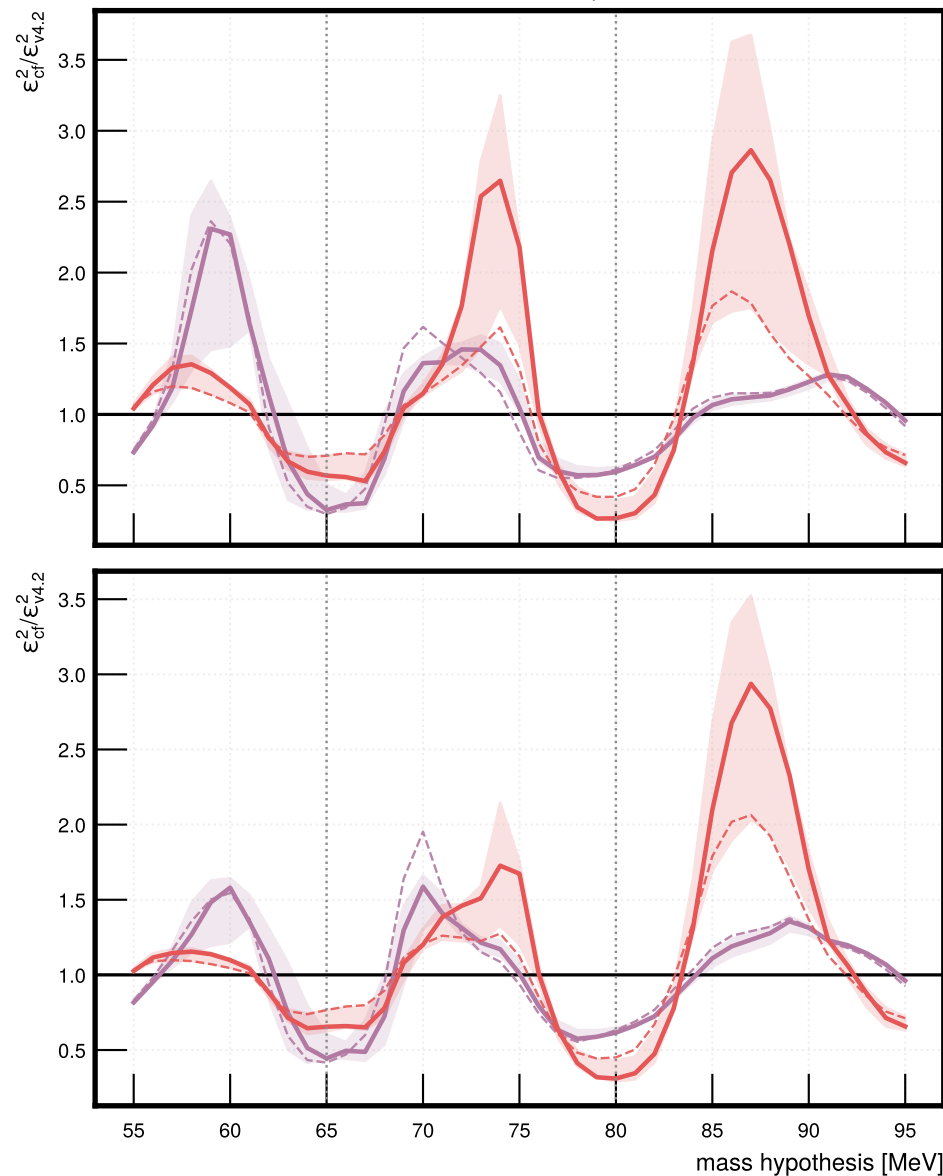
Observed-limit response
