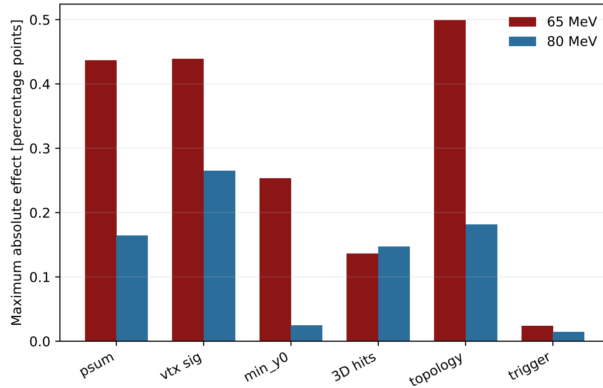
65 MeV mass-binning sensitivity
