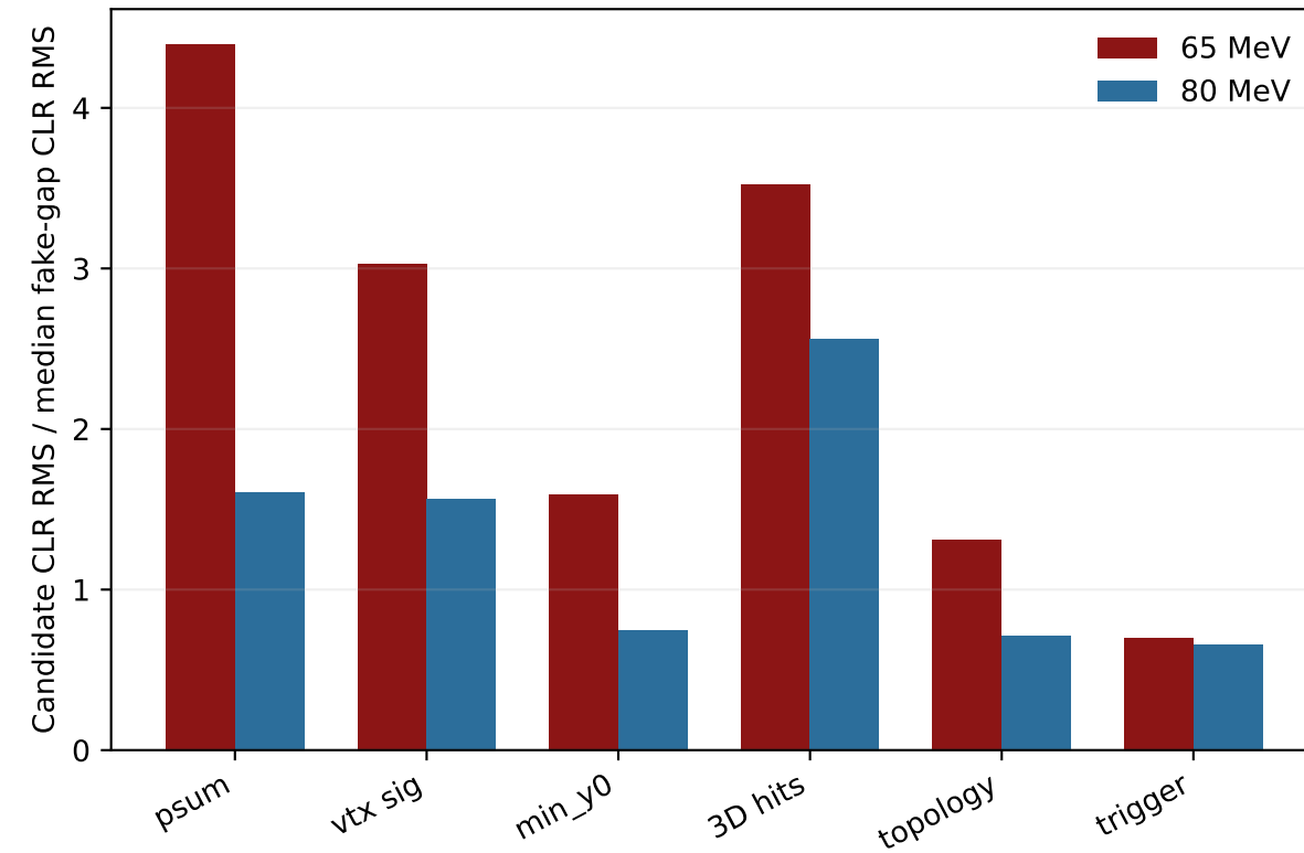
80 MeV mass-binning sensitivity
