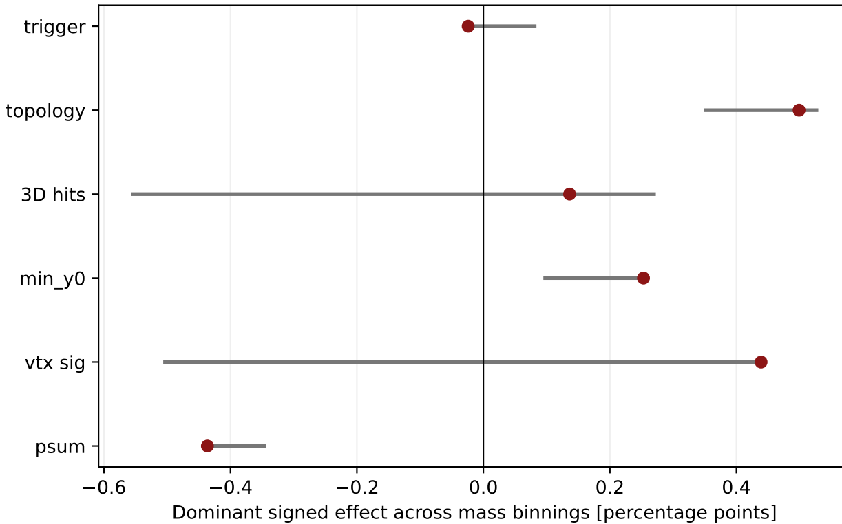
65 MeV mass-binning sensitivity
