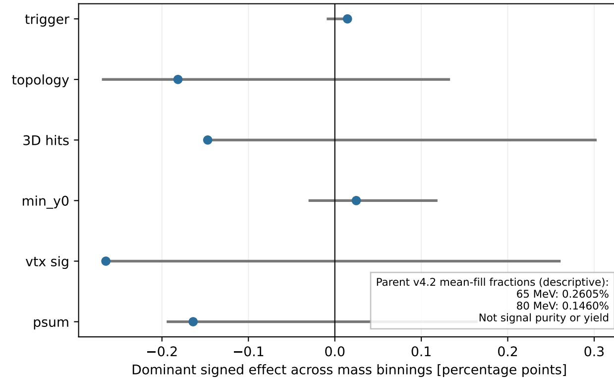
80 MeV mass-binning sensitivity
