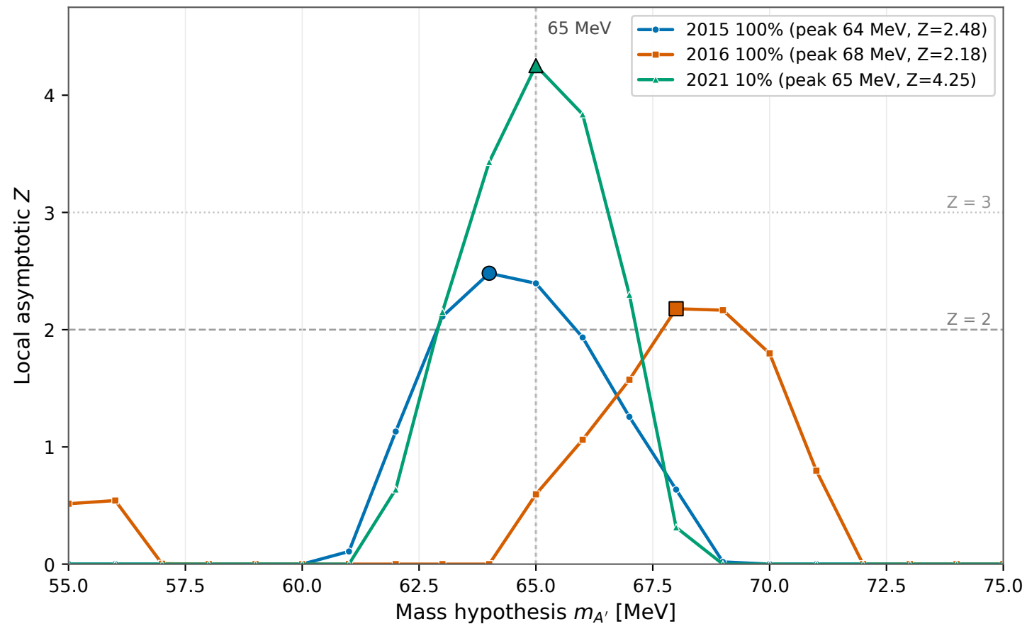
Standalone local excess profiles around 65 MeV
