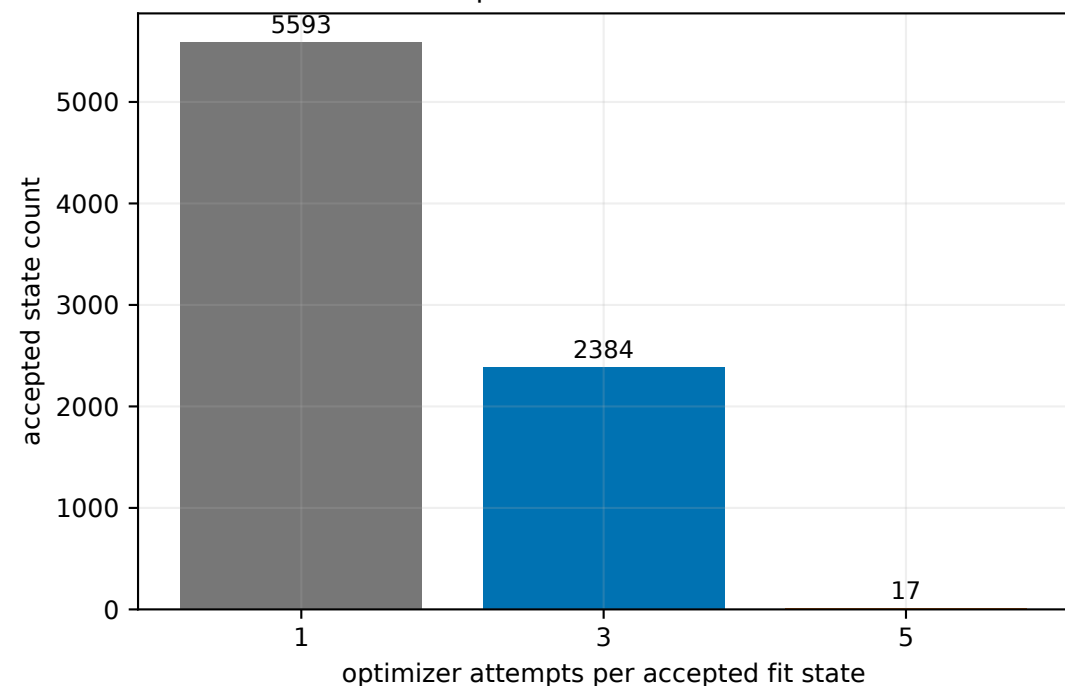
Adaptive restart workload
