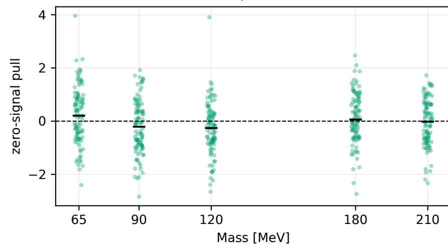
2021 10% source x10: accepted pulls black bars: medians; red x: excluded raw fit
