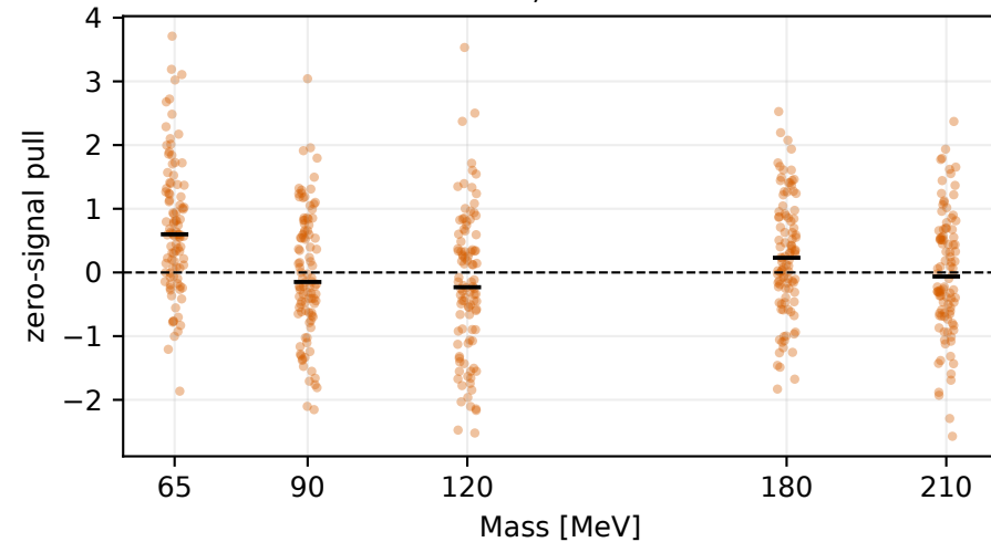
2021 1% source x100: accepted pulls black bars: medians; red x: excluded raw fit
