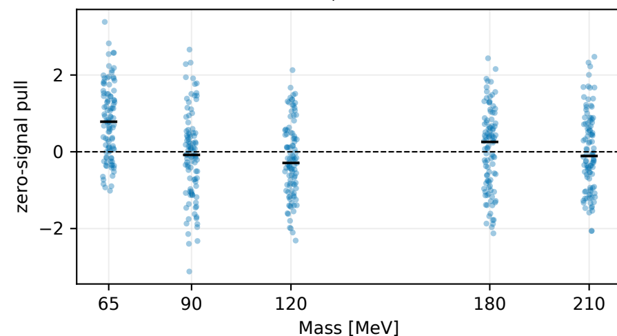
2021 native 10% source: accepted pulls black bars: medians; red x: excluded raw fit
