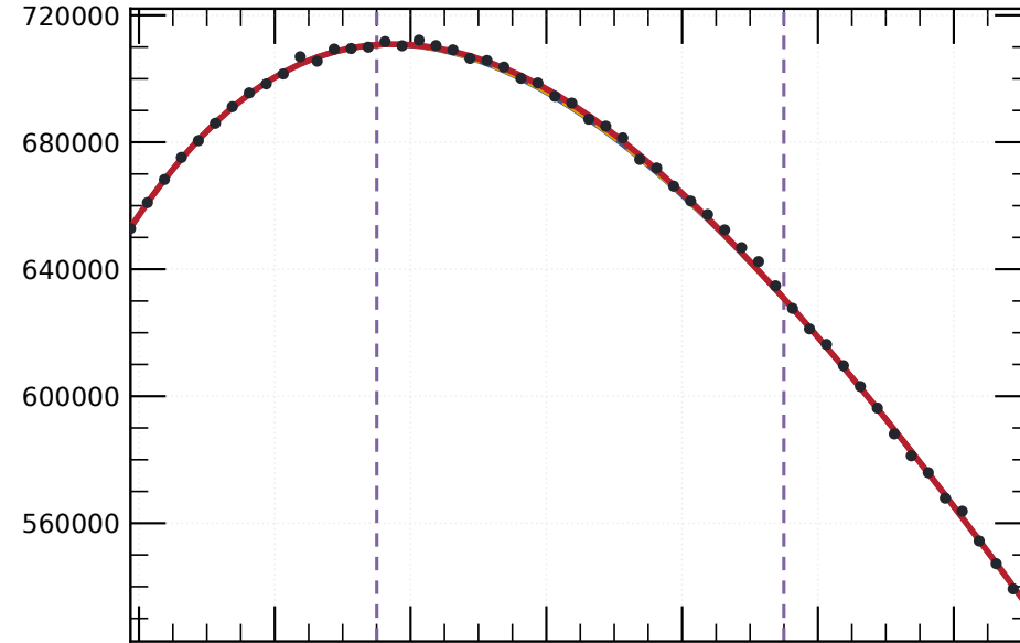
2016 100% (0.5 MeV/bin)
