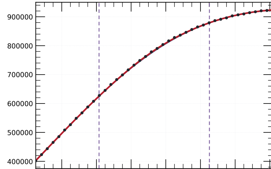
2021 10% (0.5 MeV/bin)
