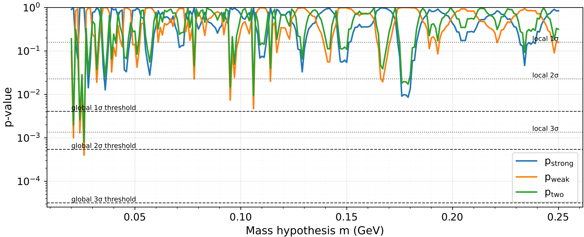
Toy-limit diagnostics with corrected global-threshold references
