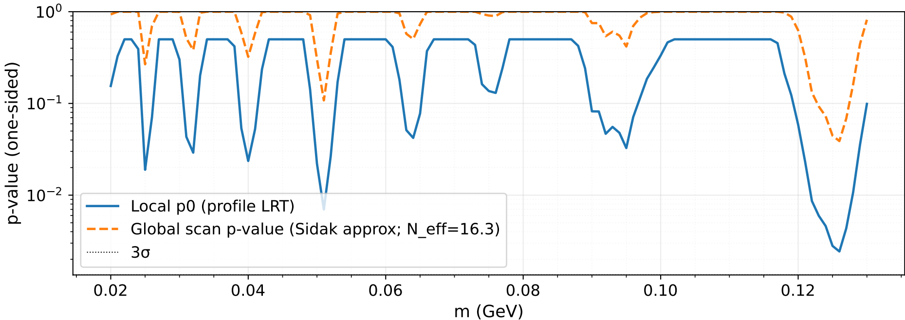
2015: local p0 and global p-value overlay
