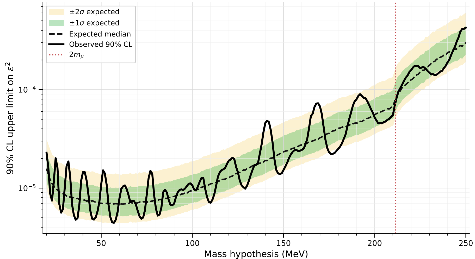
90% CL limits with minimal-model dimuon-threshold correction
