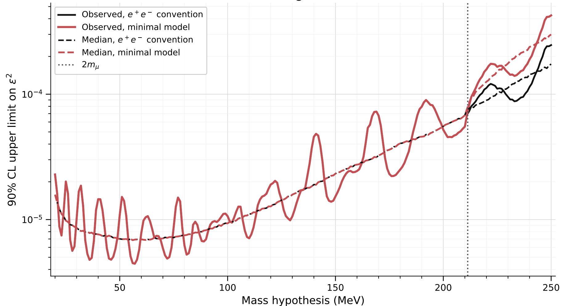
Effect of the dimuon branching correction on the 90% CL limit
