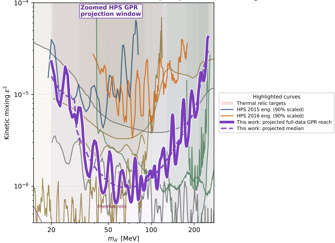
Projected full-data HPS GPR reach in the HPS prompt-search mass range
