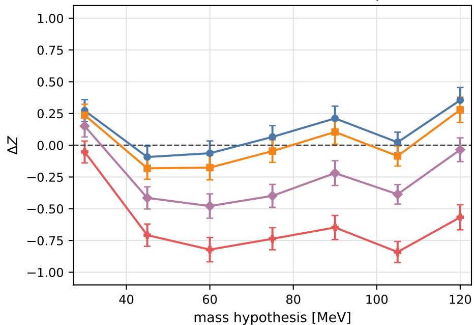
Significance residual, \hat{Z} - Z_{inj}
