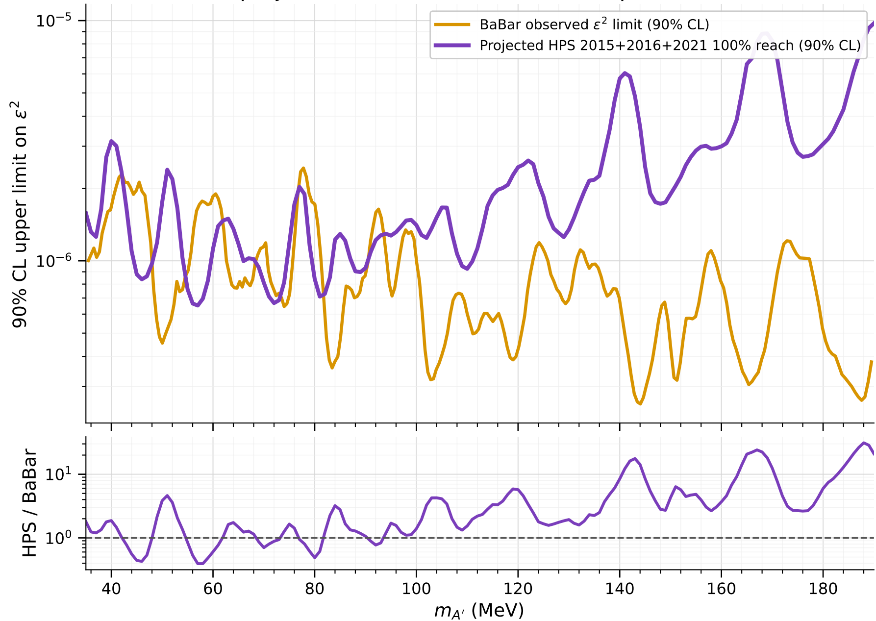
90% CL projected full-data HPS reach compared with BaBar
