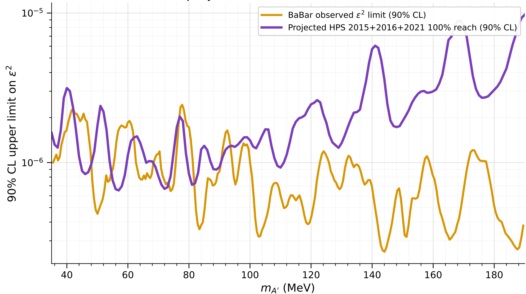
90% CL projected full-data HPS reach vs BaBar
