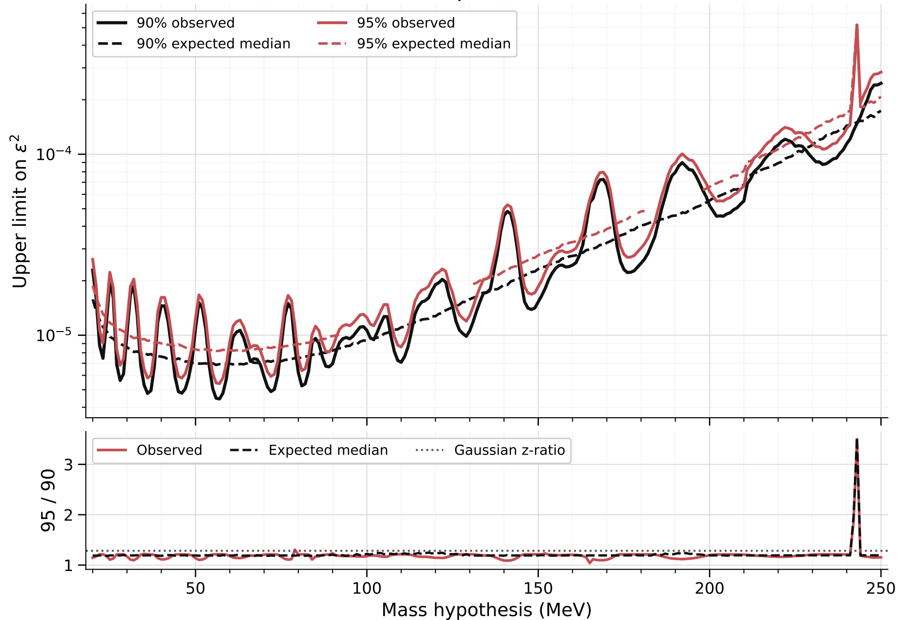
Combined observed and expected limits: 90% CL vs 95% CL
