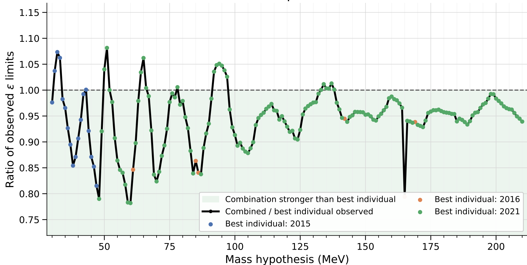
90% CL combined observed limit compared with the best individual dataset
