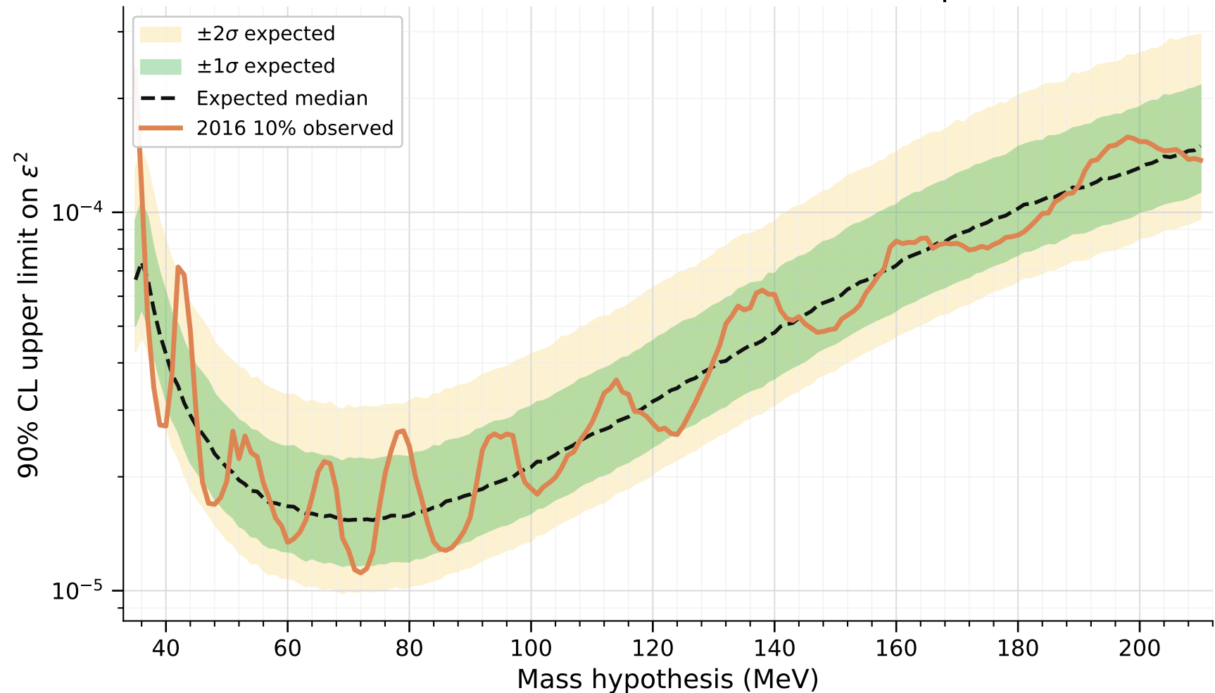
2016 10% individual 90% CL observed and expected limit
