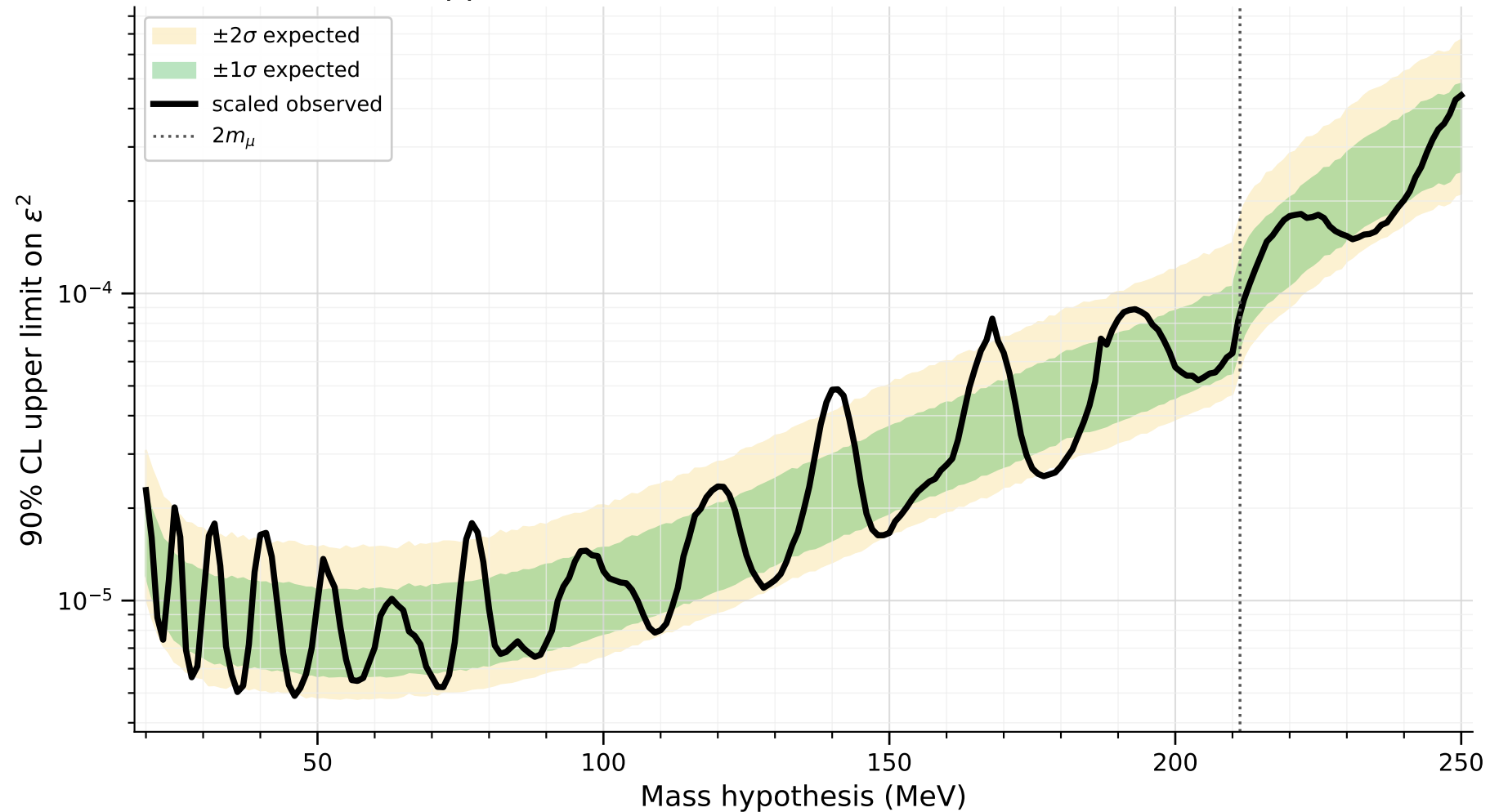
90% Combined upper limit with dimuon correction and 2021 scaled resolution
