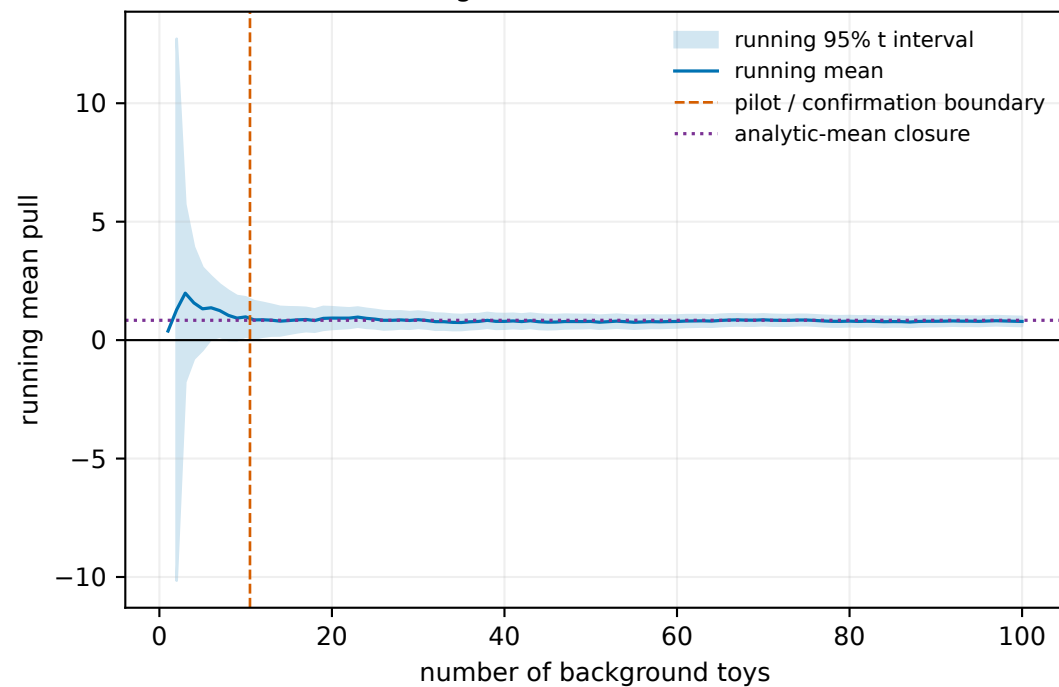
Convergence of the 65 MeV offset
