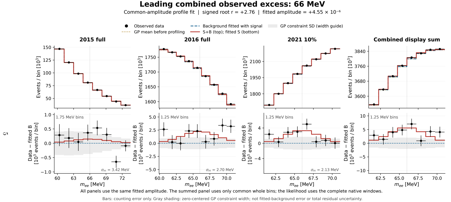
Figure 3: The 66 MeV common-amplitude fit, shown separately for each year and as a display sum. The shared signed amplitude is \hat{\epsilon}^2 = 4.55 \times 10^{-6} and r = 2.76 . Every panel uses the same amplitude, with the appropriate year-specific yield and resolution. Summed panels omit boundary pieces; the likelihood root and quoted fitted yields use the full native windows.
