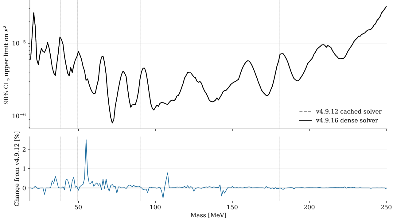
Figure 16: The pointwise upper-limit construction with the current dense and earlier cached solvers. The lower panel shows their relative difference. Both curves have the same membership and branching correction. Their difference is not a look-elsewhere adjustment or a sensitivity measurement.
