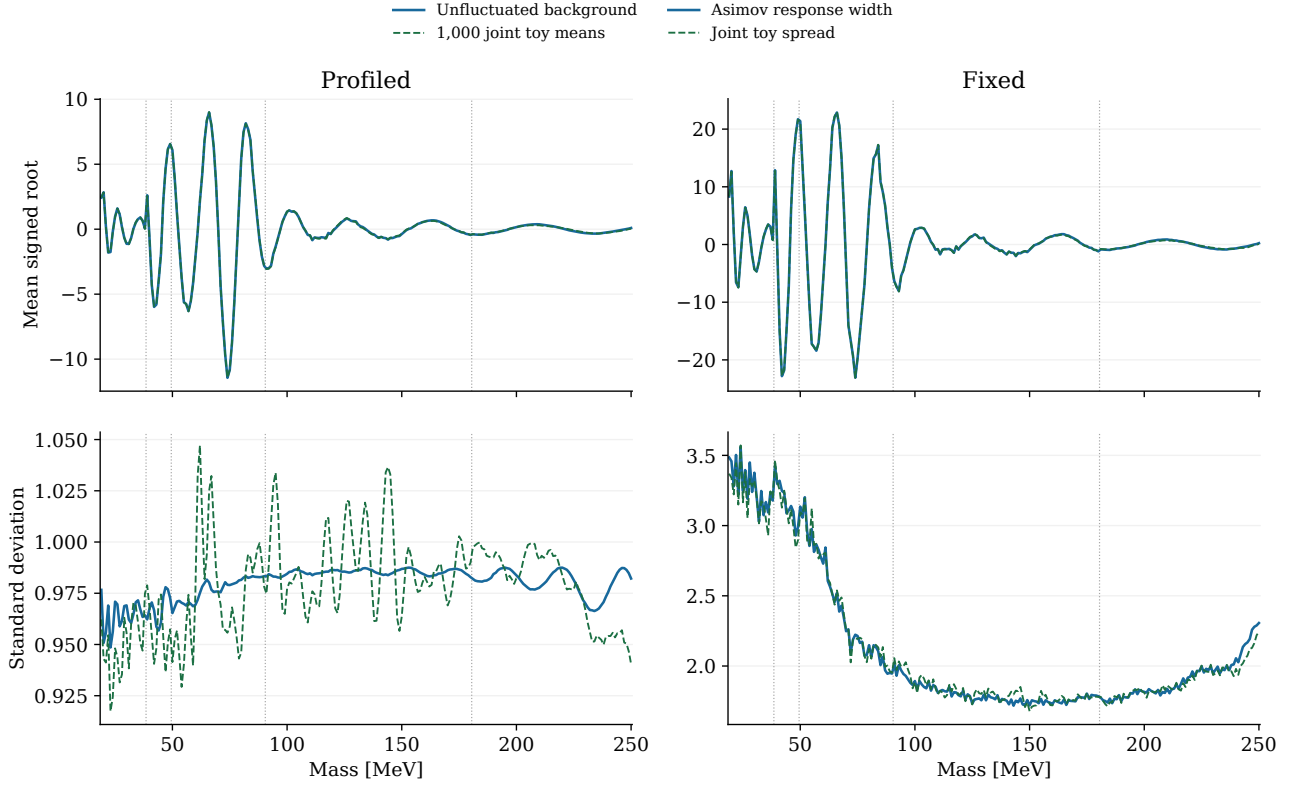
Figure 13: Asimov-response predictions compared with 1,000 joint Poisson scans. Top panels show the offset in the signed root; bottom panels show its spread. Vertical lines mark membership changes. Agreement tests the approximation under the generating means, without establishing their physical validity.
