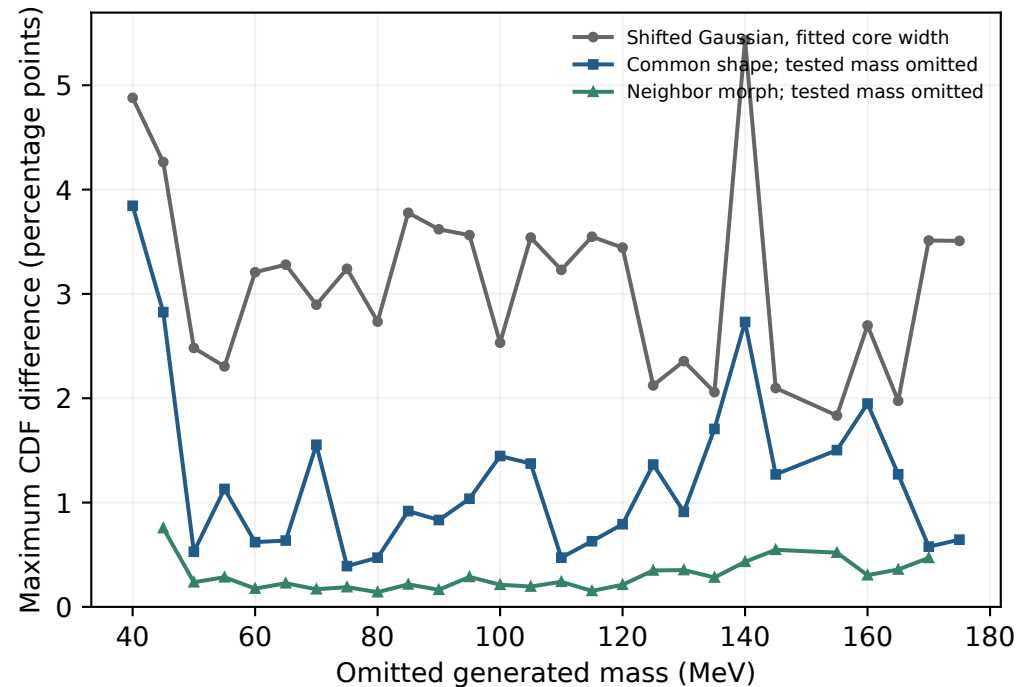
Full distribution
